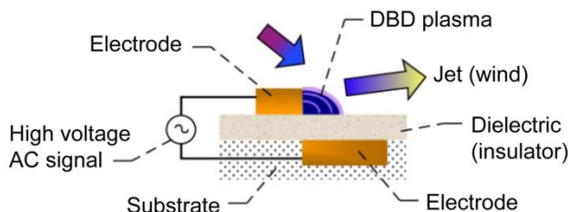
Figure 1.—Schematic of a DBD Plasma Actuator.
