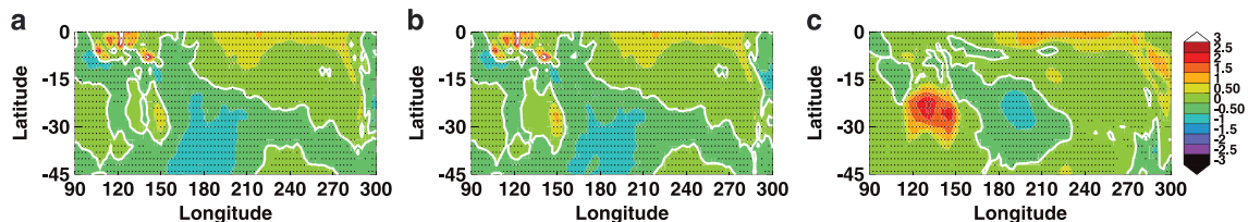
Figure 11. WPEN-NTRL 2 m temperature differences (K) in the equatorial and South Pacific in austral spring, for (a) P W -P N , (b) IDEAL W -P N , and (c) F W -F N . Black crosses indicate differences significant at the 95% level, in a two-tailed t test. White contours denote zero difference.
