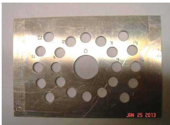
Figure 1.—Sample holder plate used in the 35 kHz hyperthermal asher.
