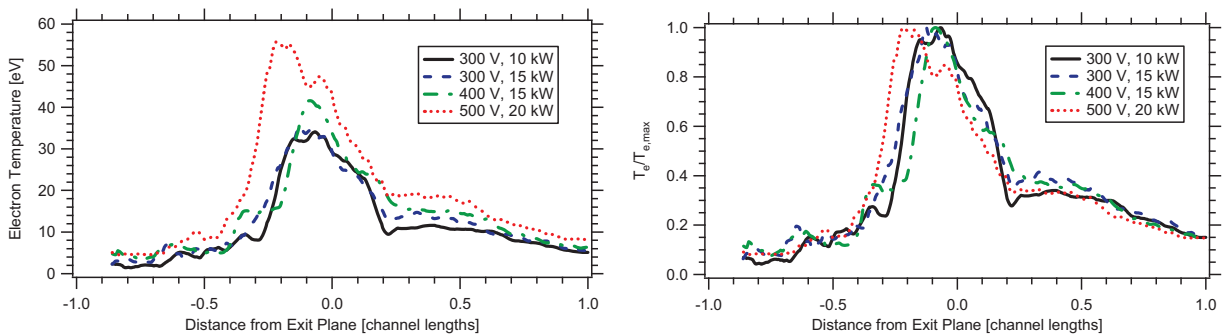
Figure 9.—Measured electron temperature axial profiles along the channel centerline of the 300M (left). Electron temperature profiles normalized by the peak temperature. All profiles are highly similar, with only slight shifts in the location of the peak (right).
