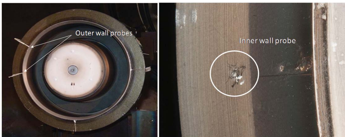
Figure 7.—Photographs of flush-mounted Langmuir probes installed on the 300MS. Probes on the outer wall, with lead wires seen routed around outer front magnetic pole (left). Close-up of probe on the inner wall (right).
