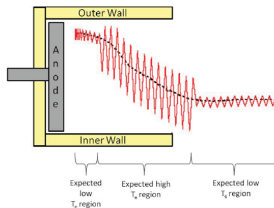
Figure 5.—Illustration of how the probe voltage was generated along channel centerline for the cylindrical Langmuir probe. Voltage was applied around the measured floating potential (dotted line), and the amplitude of the voltage was increased in the region of high expected electron temperatures. Not to scale.
