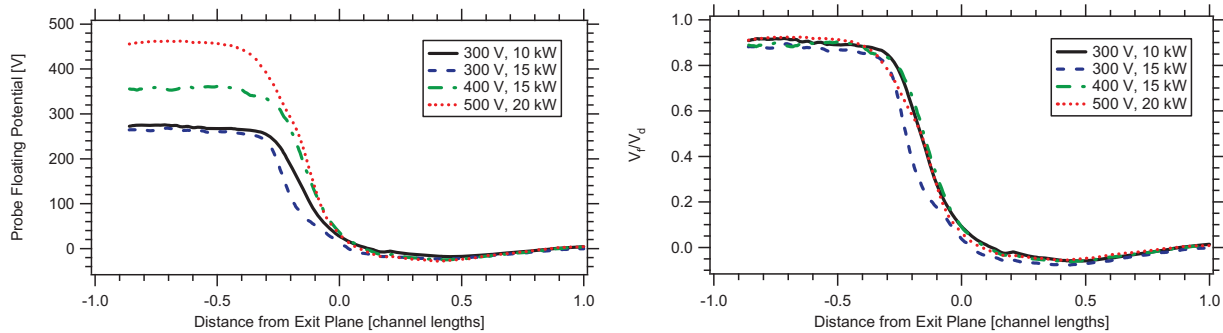
Figure 8.—Measured probe floating potential axial profiles along the channel centerline of the 300M (left). Once normalized by the discharge voltage, these profiles were found to be highly similar (right).
