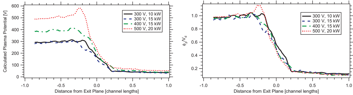
Figure 10.—Calculated plasma potential axial profiles along the channel centerline of the 300M (left). Profiles non-dimensionalized by the discharge voltage, showing highly similar acceleration zones (right).
