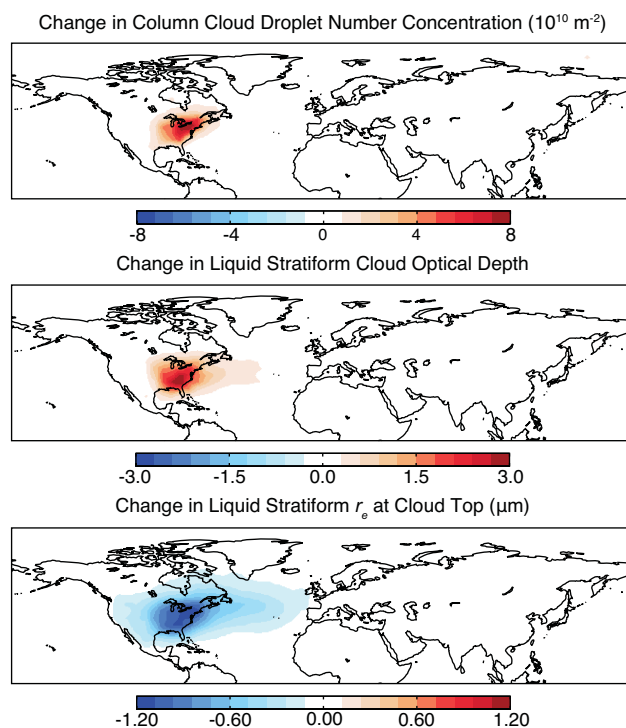
Fig. 9. Effect of US anthropogenic aerosols on column integrated cloud droplet number concentration, liquid stratiform cloud droplet effective radius at cloud top ( r_c ), and liquid stratiform cloud optical depth. Values are annual model means for 1980.
