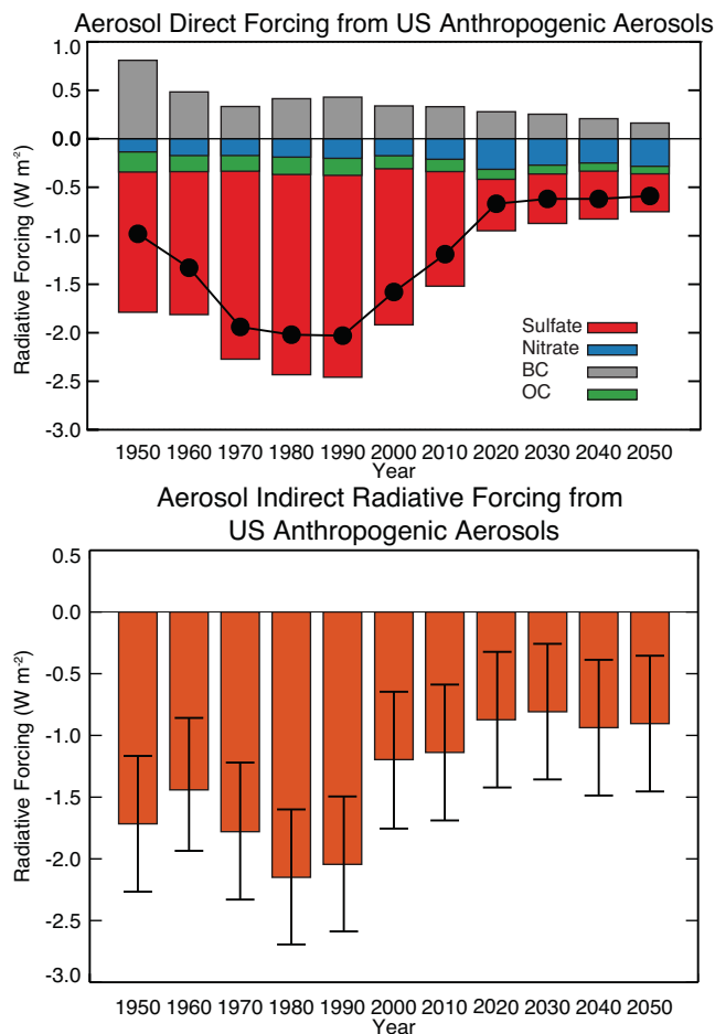
Fig. 8. 1950–2050 evolution of aerosol direct (top) and total (first + second) indirect radiative forcing (bottom) from US anthropogenic sources over the eastern US (east of 100^{\circ} W). Circles represent the net direct radiative forcing and the bars give the contributions from the different components. The direct radiative forcing calculations are for an internal aerosol mixture. Aerosol indirect radiative forcing is calculated as the difference between two 50-yr equilibrium climate simulations with vs. without US anthropogenic aerosols. The error bars represent the 95 % confidence interval of the forcing based on model interannual variability.
