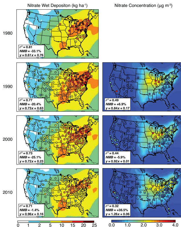
Fig. 5. Same as Fig. 2 but for nitrate.
