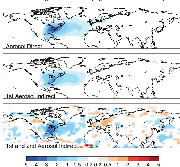
Fig. 7. Annual mean aerosol direct (top), first indirect (middle), and total indirect (bottom) radiative forcing from US anthropogenic sources for year 1980.
