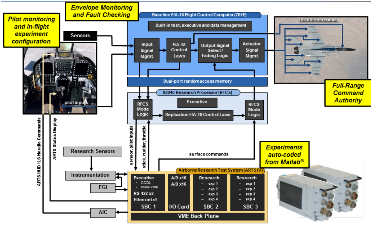
Figure 7.1-4. RFCS/ARTS
