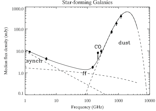
Figure 3. The median flux densities in NVSS, PMN/GBT, ACT and Herschel surveys of SFGs from Best & Heckman (2012). Described in Section 3.3.1, a model with synchrotron, free-free, the CO line for z = 0.05 (rest frame frequency 230.5 GHz) and dust gray body emission is fit to the SFG data, and the model parameters describing the best fit (shown here) are listed in Table 2. The dashed lines illustrate the synchrotron component, the free-free emission component and the dust gray body component of the model, and the solid line illustrates the full model evaluated for the best fit parameters. The error bars on the medians shown are the diagonal elements of the covariance matrix computed via bootstrap sampling (off-diagonal elements were included for the fitting). The error bars on the low frequency median flux densities are smaller than the size of the symbols.
