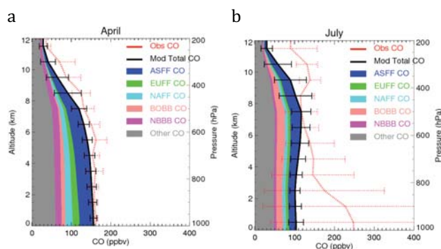
Fig. 8. Vertical distribution of the CO volume mixing ratio (ppbv) from GEOS-5 simulation when the model results are averaged over the Arctic region 50N–90N and 190E–320E for April (a) and July (b). The GEOS-5 CO is shown by the thick black line for total and by the color shaded areas for the corresponding tagged components. The “Other CO” refers to the global CO other than the five tagged CO species defined in Fig. 1a and it is mostly attributed to the CO chemical formation from methane oxidation. The CO mixing ratio from along the DC-8 flight tracks is also shown by the dotted red line with the standard deviation shown by horizontal bars for a reference.
