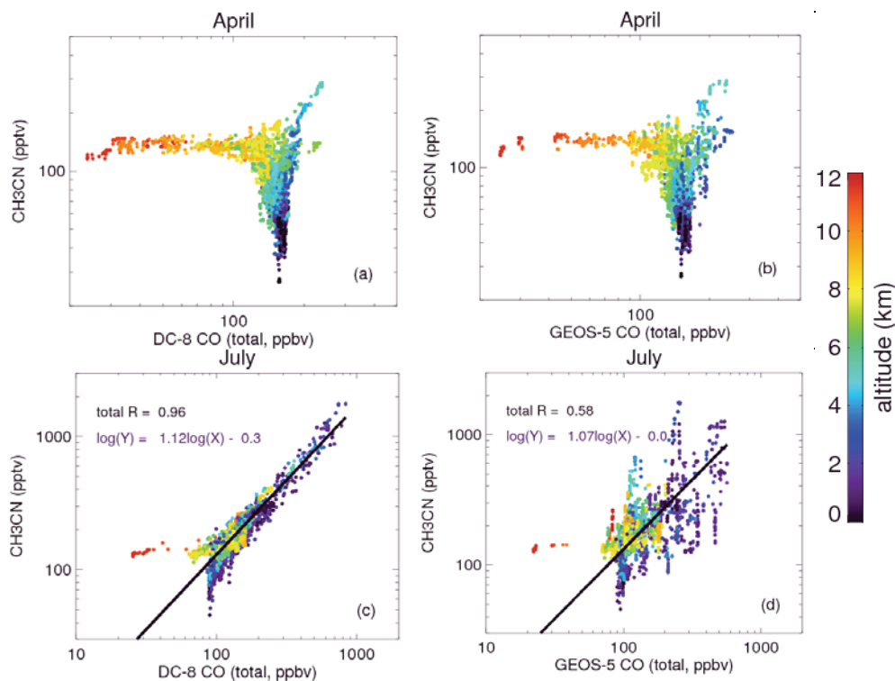
Fig. 5. Scatter plots of observed CH 3 CN (pptv) and DC-8 observed CO (ppbv) (a and c) and of observed CH 3 CN (pptv) and GEOS-5 simulated total CO (b and d) in ARCTAS-A and -B campaigns. The results are colored according to the measurement altitudes. Each point represents median values of model results and observations within 10 min.
