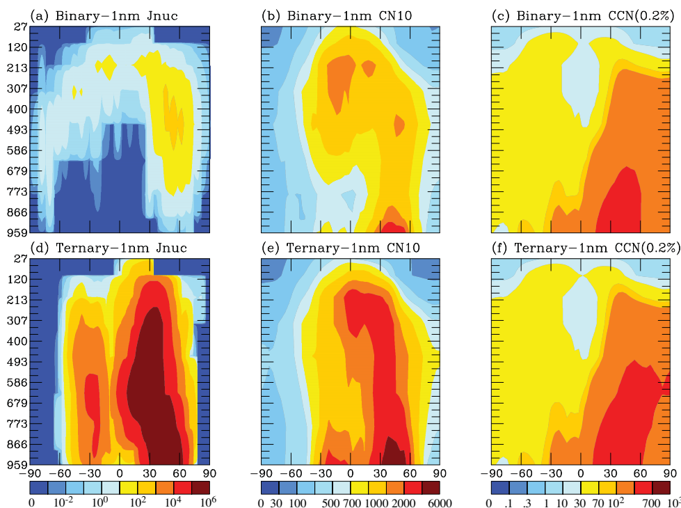
Fig. 2. Pressure (hPa) vs. latitude maps for March-to-May averaged nucleation rates ( J_{\text{nuc}} ) ( \text{cm}^{-3} \text{s}^{-1} at 273 K and 1 atm), CN10 ( D_p \geq 10 nm) ( \text{cm}^{-3} at 273 K and 1 atm), CCN(0.2%) ( \text{cm}^{-3} at 273 K and 1 atm) for Binary-1 nm and Ternary-1 nm simulations.
