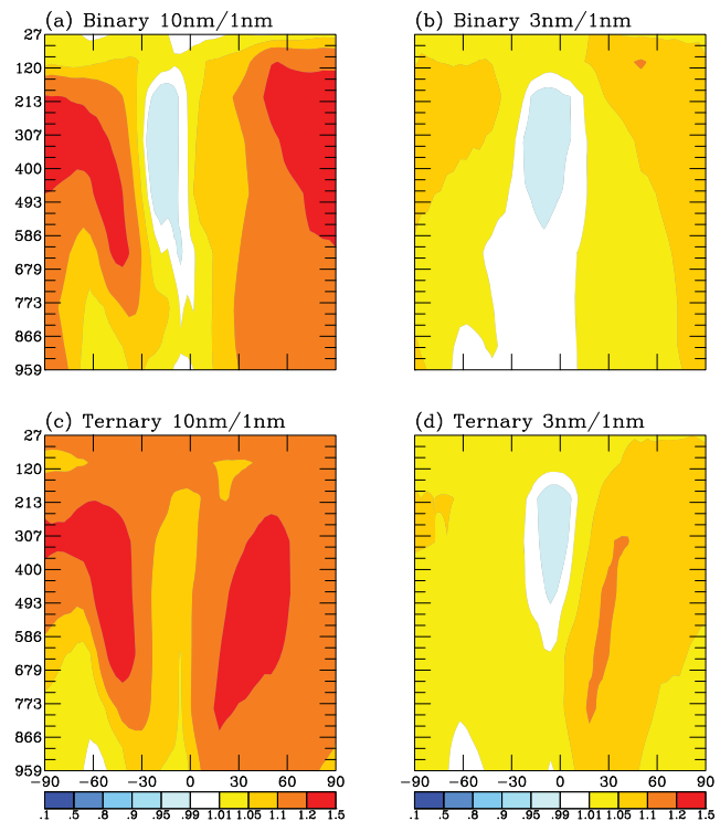
Fig. 5. Pressure (hPa) vs. latitude maps for March-to-May averaged ratios of CCN(0.2 %) concentrations from the following scenarios: (a) Binary-10 nm to Binary-1 nm, (b) Binary-3 nm to Binary-1 nm, (c) Ternary-10 nm to Ternary-1 nm, and (d) Ternary-3 nm to Ternary-1 nm.
