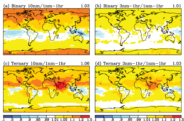
Fig. 9. Same as Fig. 6 but for the following scenarios: (a) Binary-10 nm to Binary-1 nm-1 h, (b) Binary-3 nm-1 h to Binary-1 nm-1 h, (c) Ternary-10 nm to Ternary-1 nm-1 h, and (d) Ternary-3 nm-1 h to Ternary-1 nm-1 h. The value on the top right of each figure is a global average of the ratios displayed in the map.
