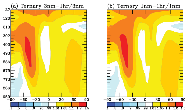
Fig. 7. Same as Fig. 5 but for the following scenarios: (a) Ternary-3 nm-1 h to Ternary-3 nm and (b) Ternary-1 nm-1 h to Ternary-1 nm.
