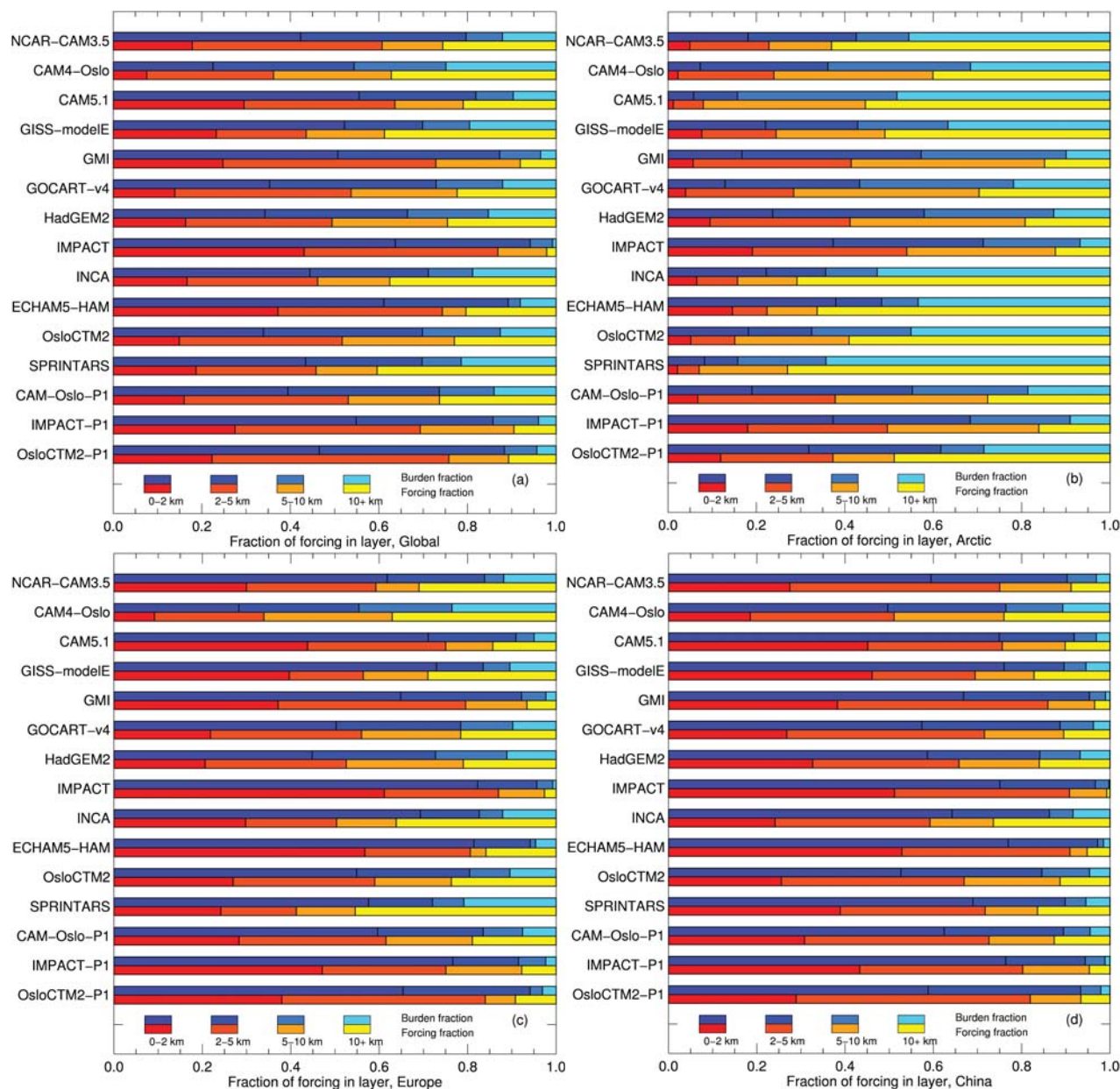
Fig. 4. Mass and forcing fractions in four altitude bands, globally and for three regions. Upper rows show burden fractions in blues, lower rows show RF fractions in reds. (a) Global mean, (b) Arctic, (c) Europe, (d) China.
