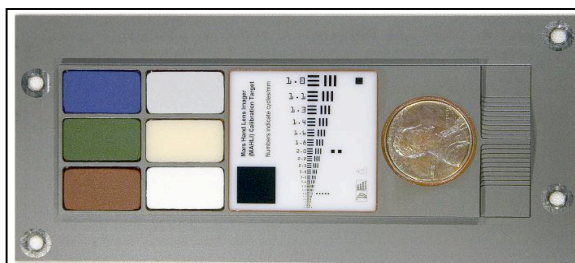
Figure 1: The calibration target for the MAHLI imaging instrument on MSL. Targets include color targets (six coupons at left), visual calibration target (center), a US penny (right), and a stepped auto-focus target to the right of the penny. The SHERLOC instrument will leverage the flight heritage of this hardware. The auto-focus target will remain in the SHERLOC calibration target, but the other targets will be replaced with targets to include carbon-bearing glass targets, EMU material samples, two meteorites (carbonaceous and martian) as described in the text.
