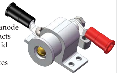
Figure III: Mechanical design of the \mu CAT
