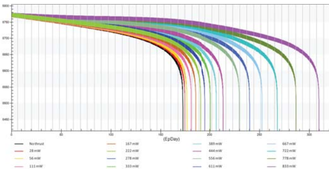
Figure II: Increased orbital lifetime. Semi-major axis evolution for various power ranges for a 1U Cubesat in a 400 km circular orbit
