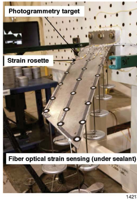
Figure 15. Test setup for the test plate.
