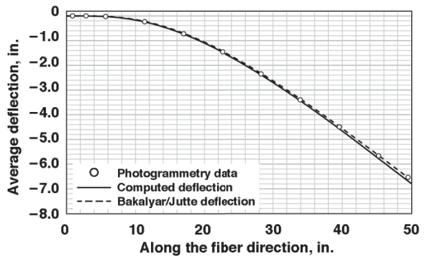
b) Leading-edge fiber (step 2 result with 10 modes).
