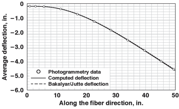
a) Leading-edge fiber (step 1 result).
