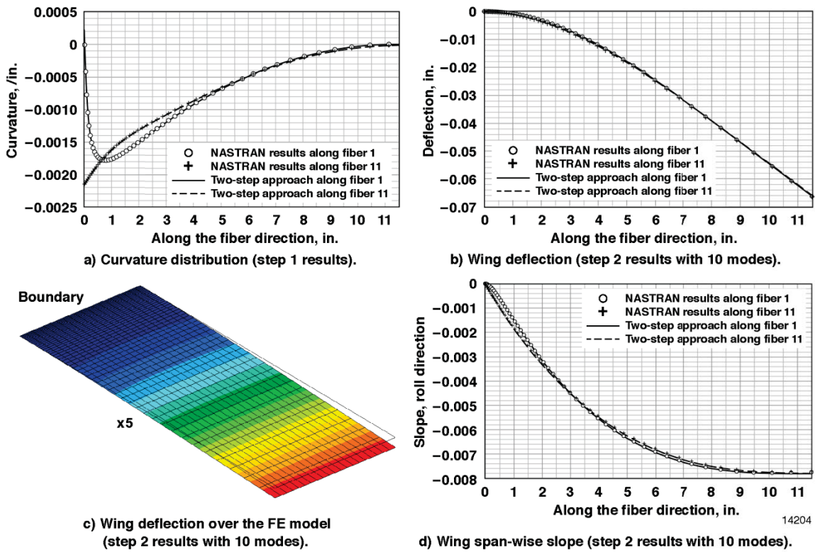
Figure 6. Curvature, wing deflection, and slopes of the rectangular wing model along Fibers 1 and 11 under a 1g load.
