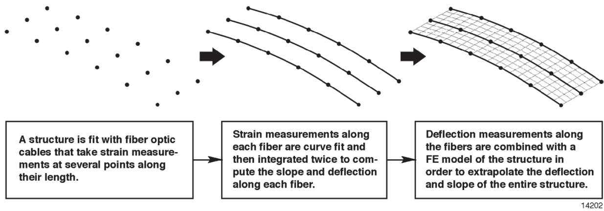
Figure 4. Steps used to compute deflection and slope.
