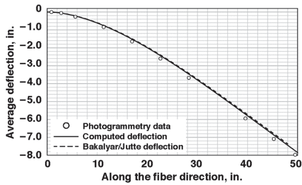
e) Trailing-edge fiber (step 1 result).
