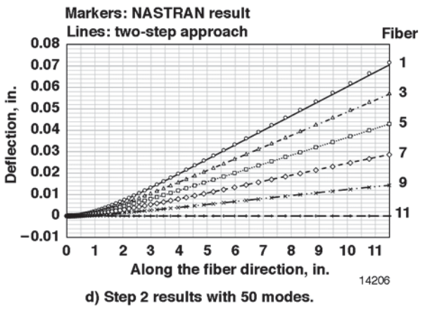
Figure 8. Effect of the number of modes on the wing deflection during the second step.
