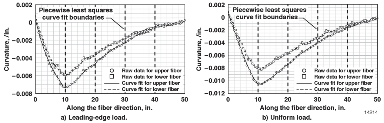
Figure 16. Pieewise least squares curve fit of curvature data along the leading-edge fiber for the test plate.
