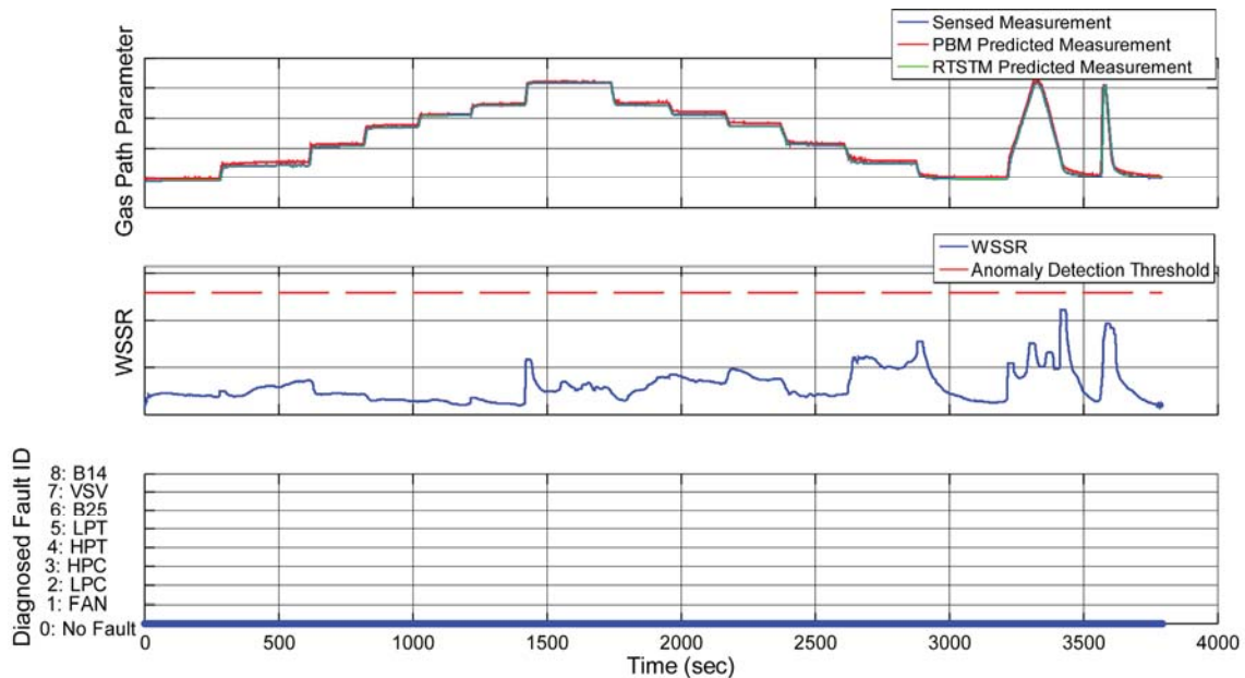
Figure 3.—Baseline VIPR I results.
