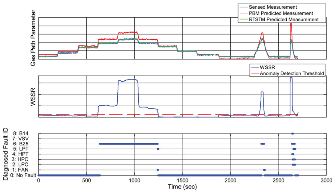
Figure 6.—Station 2.5 bleed valve fault VIPR II results.
