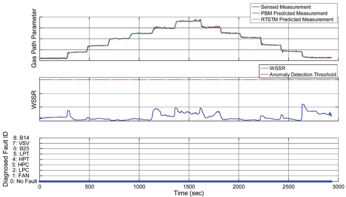
Figure 4.—Baseline VIPR II results.
