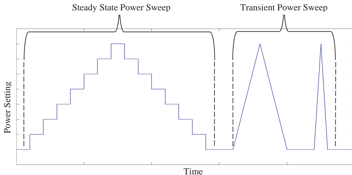
Figure 2.—Representative VIPR event test sequence.
