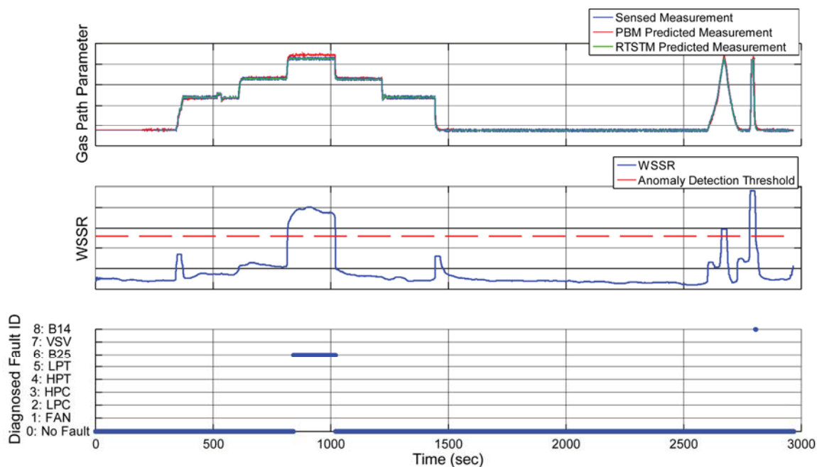
Figure 5.—Station 2.5 bleed valve fault VIPR I results.
