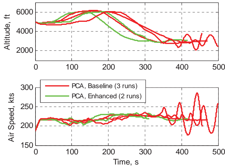
Figure 17.—Climb/descend maneuver: piloted evaluations.
