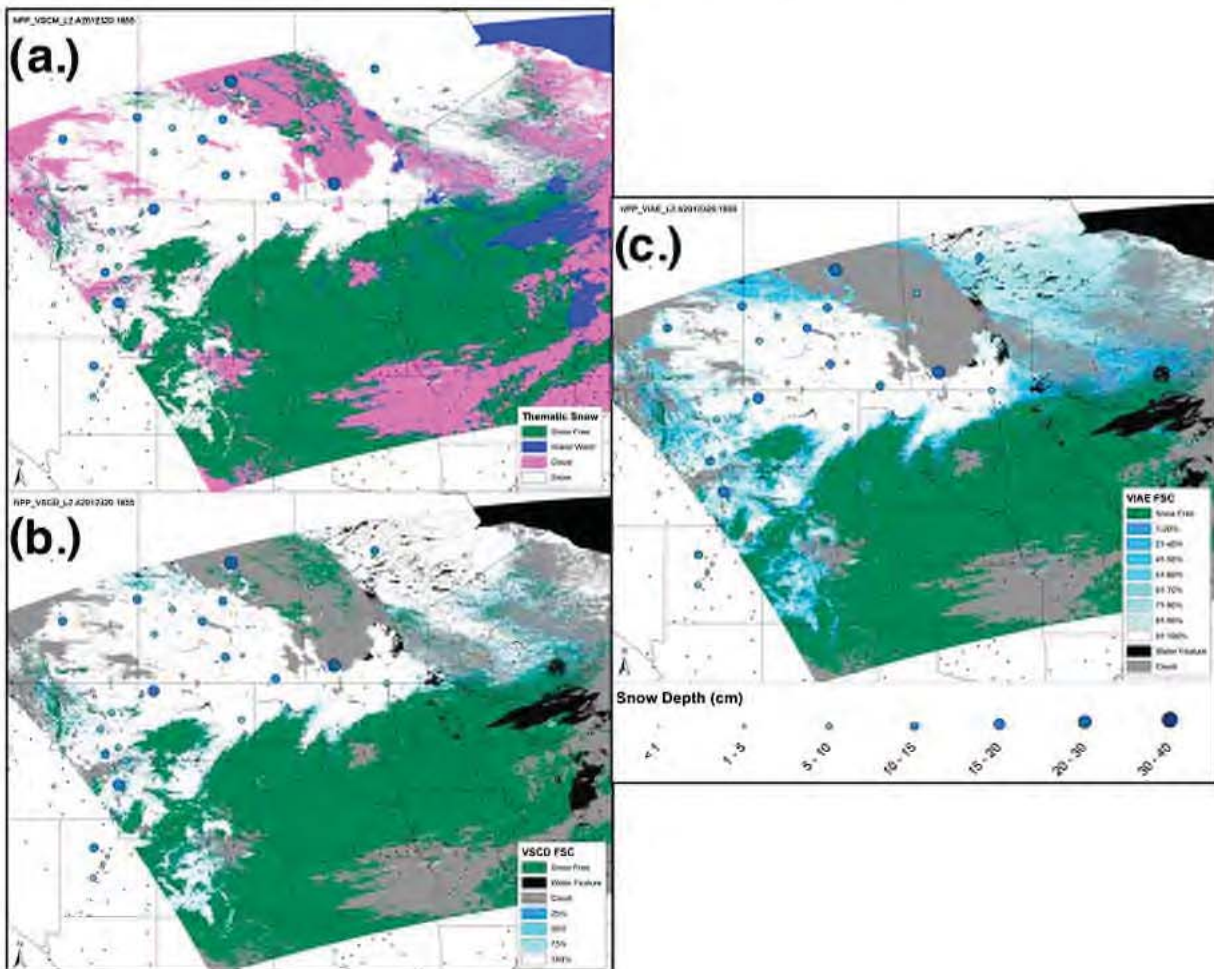
Figure 8. (a) VIIRS Snow Cover Binary Map (NPP_VSCM) compared to (b) Level 2 VIIRS Snow Fraction Product at 750 m (NPP_VSCD) and (c) VIIRS fractional snow cover based on MODIS heritage algorithm using the Level 1 VIIRS Sensor Data Record (SDR) at 375 m (NPP_VIAE). (NPP_VIAE) (acquired 15 November 2012).
