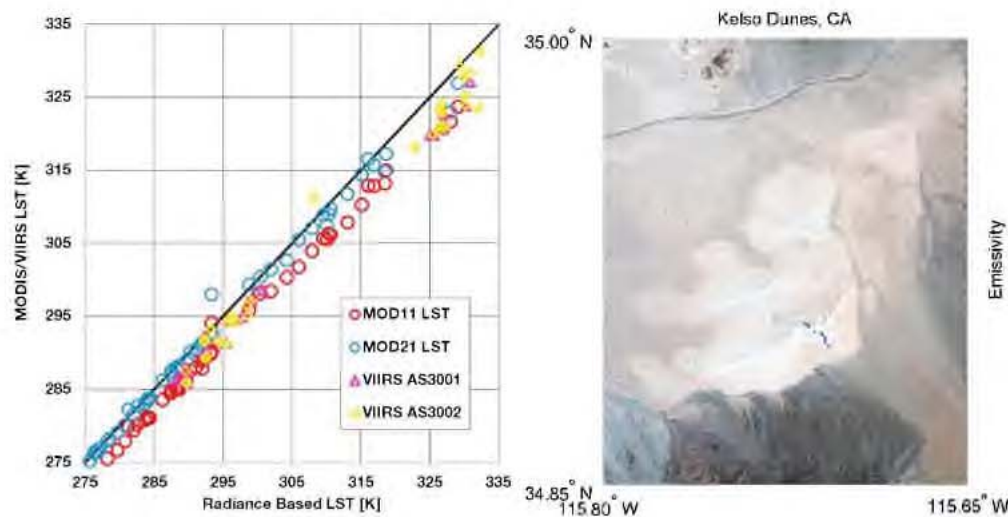
Figure 1. (left) Plot of MODIS/VIIRS LST at the Kelso Dunes, California, pseudo-invariant site (image on right) versus radiance-based LST.
