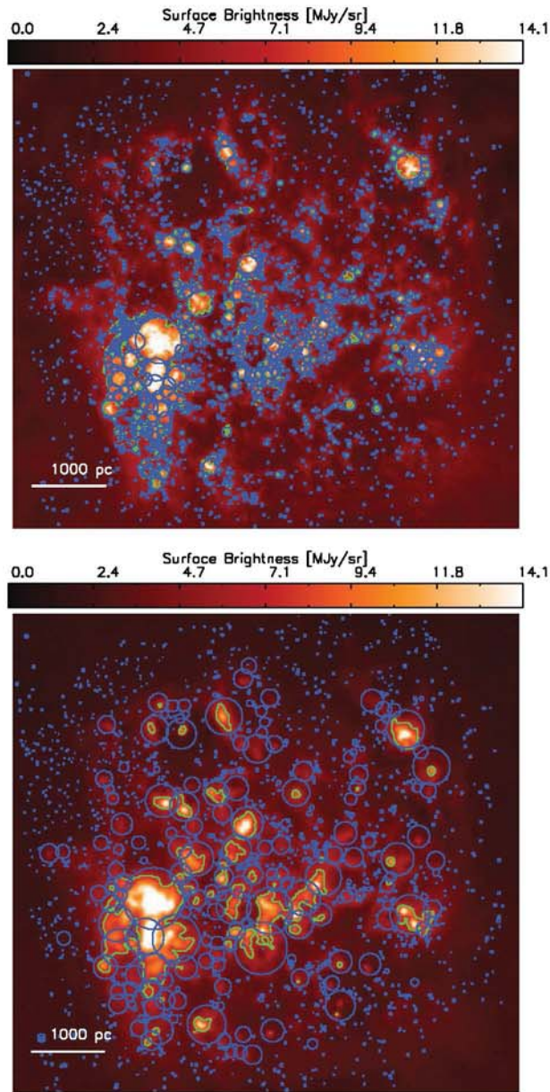
Figure 4. Spitzer MIPS 160\ \mu\text{m} (top) and IRAS 100\ \mu\text{m} (bottom) maps of the LMC. The masks used to interpolate the PACS timelines inside bright or compact sources in the LMC during the baseline estimate are overlaid as blue circles. The 50\ \text{Mly}\ \text{sr}^{-1} surface brightness contour, corresponding to the transition to the nonlinear regime of MIPS 160\ \mu\text{m} is shown in green in the MIPS image.
