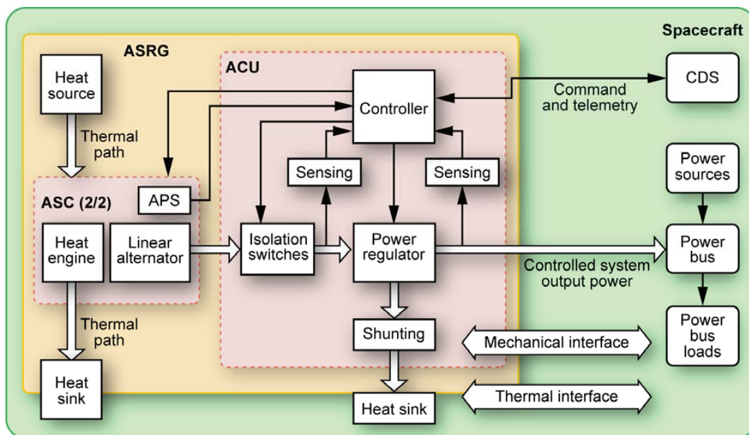
Figure 3.—Advanced Stirling Radioisotope Generator (ASRG) interfaces. APS is ASC (Advanced Stirling Converter) position sensor; ACU is ASC Controller Unit; and CDS is command and data subsystem.
