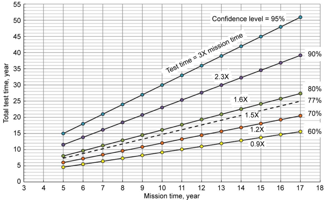
Figure 7.—Total test time without failures for mean time to failure (MTTF) is equal to mission time.
