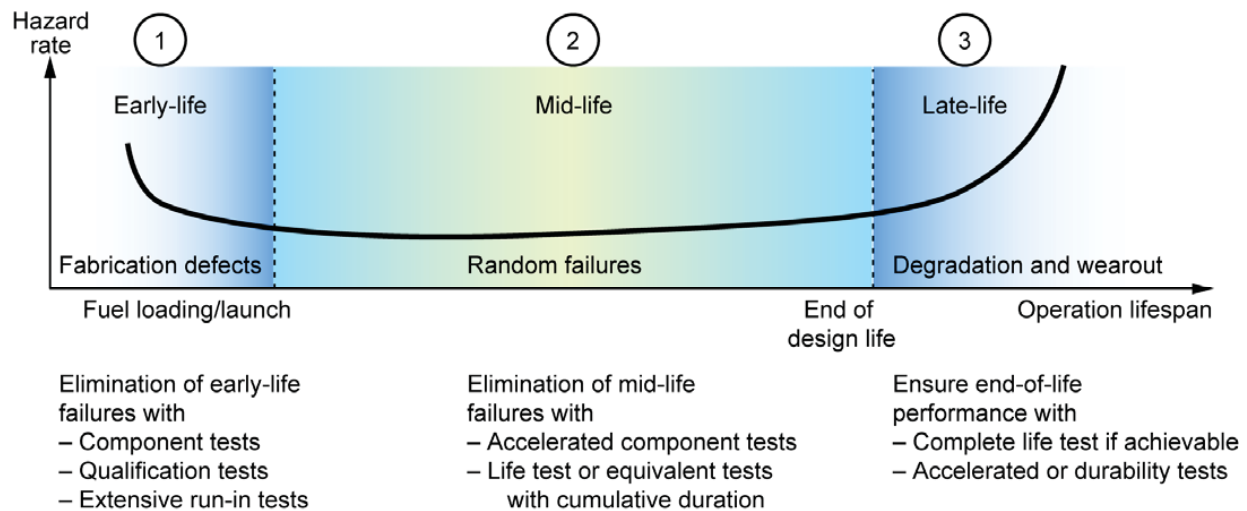
Figure 5.—System life phases.
