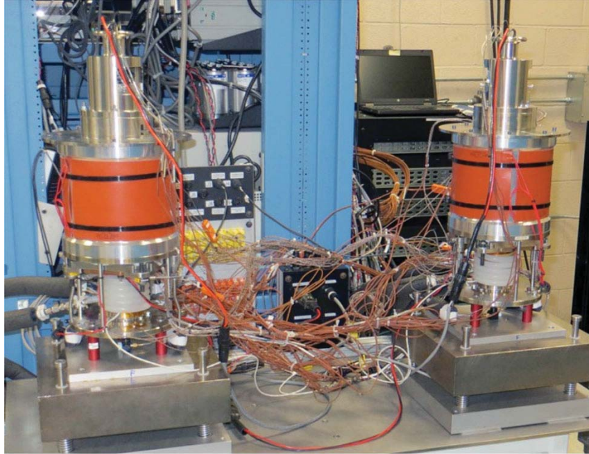
Figure 4.—Advanced Stirling Convertor (ASC)—E3 #3 and #4 under test in NASA Glenn Research Center Stirling Research Laboratory.
