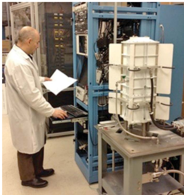
Figure 2.—Advanced Stirling Radioisotope Generator Engineering Unit 2 (EU2) generator housing assembly being set up for test in the Stirling Research Laboratory.
