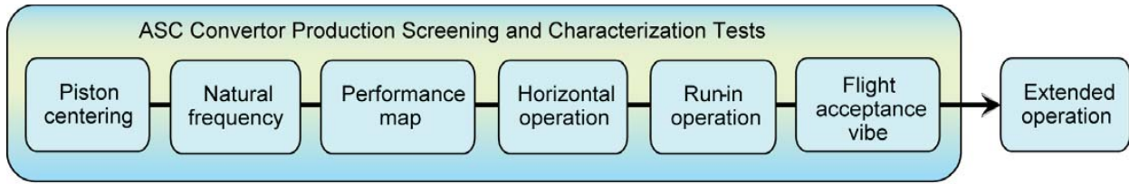
Figure 6.—Advanced Stirling Converter (ASC) screen and characterization tests preceding extended operation.
