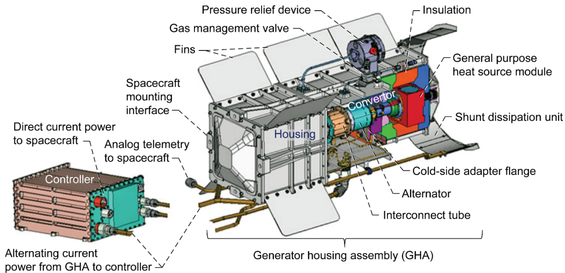
Figure 1.—Advanced Stirling Radioisotope Generator system.
