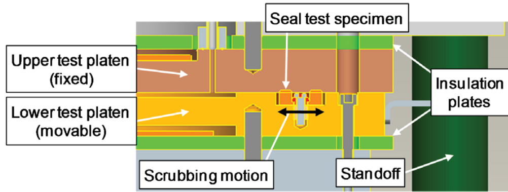
Figure 18.—Cross section through seal durability test apparatus showing seal test specimen and scrubbing motion.
