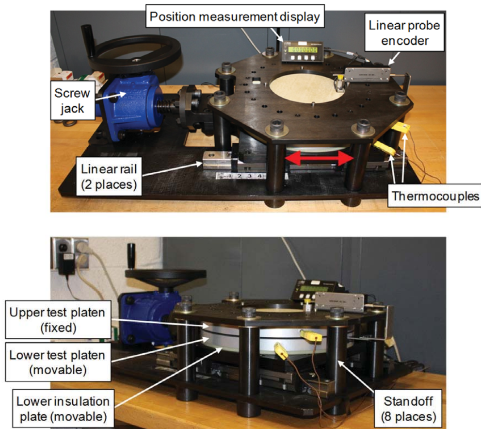
Figure 17.—Main components of seal durability test apparatus.
