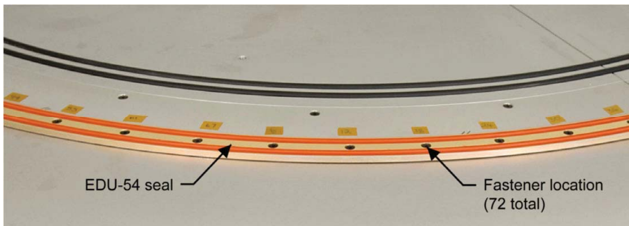
Figure 4.—Photograph of 54-in. diameter (EDU-54) Gask-O-seal installed in test apparatus showing dual front seal bulbs and fastener holes.
