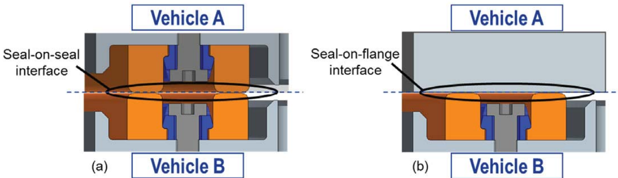
Figure 7.—Cross sections through the interface between two mated systems showing (a) seal-on-seal mating and (b) seal-on-flange mating.
