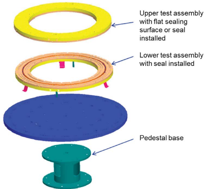
Figure 20.—Exploded view of full-scale seal leak test fixture showing main elements.
