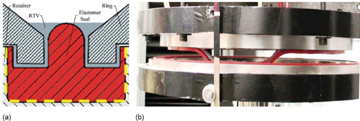
Figure 16.—Test fixture used to perform seal pull-out/bond strength tests including (a) cross section through model of test fixture showing how ring is bonded to top surface of Gask-O-seal bulb and (b) photo during a test.
