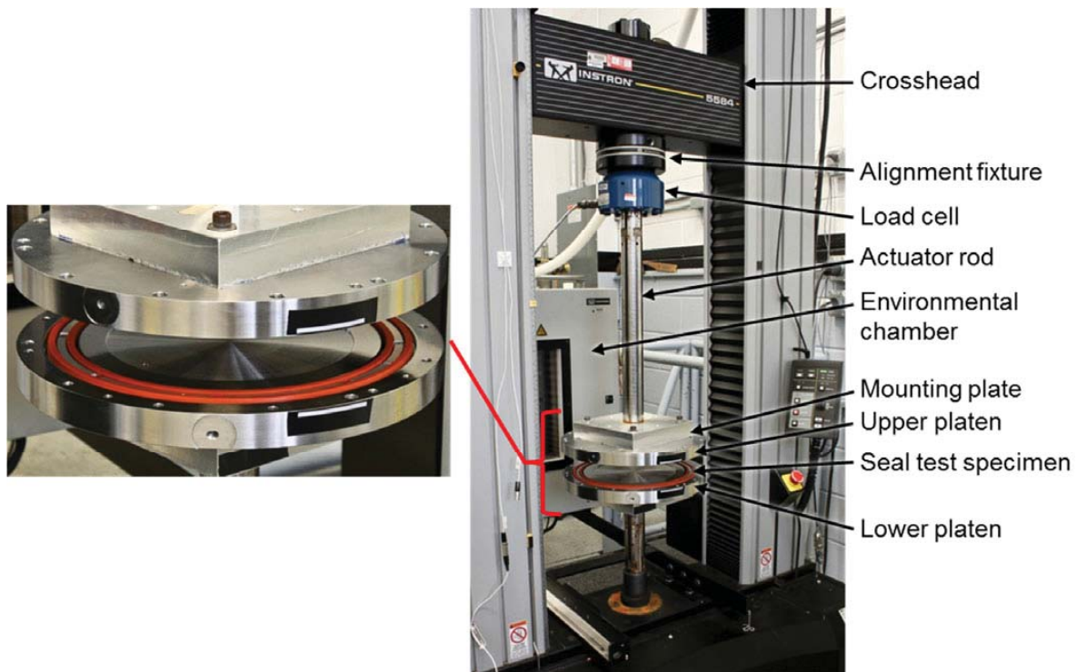
Figure 14.—Test apparatus used for medium-scale seal compression and adhesion tests.
