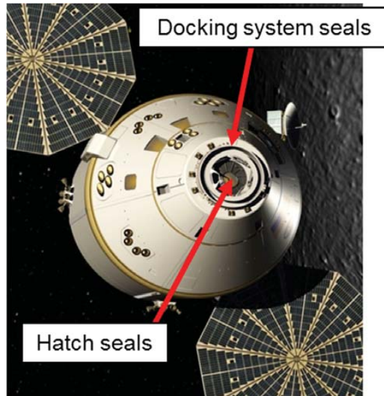
Figure 1.—Locations for advanced seal designs on the Orion spacecraft.
