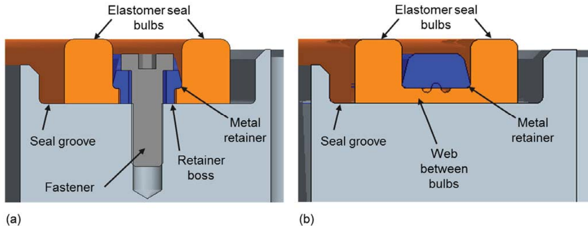
Figure 5.—Cross section through multi-piece seal assembly (a) at fastener location and (b) at location between fasteners.
