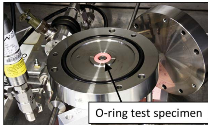
Figure 8.—O-ring test specimen installed in leak test fixture.
