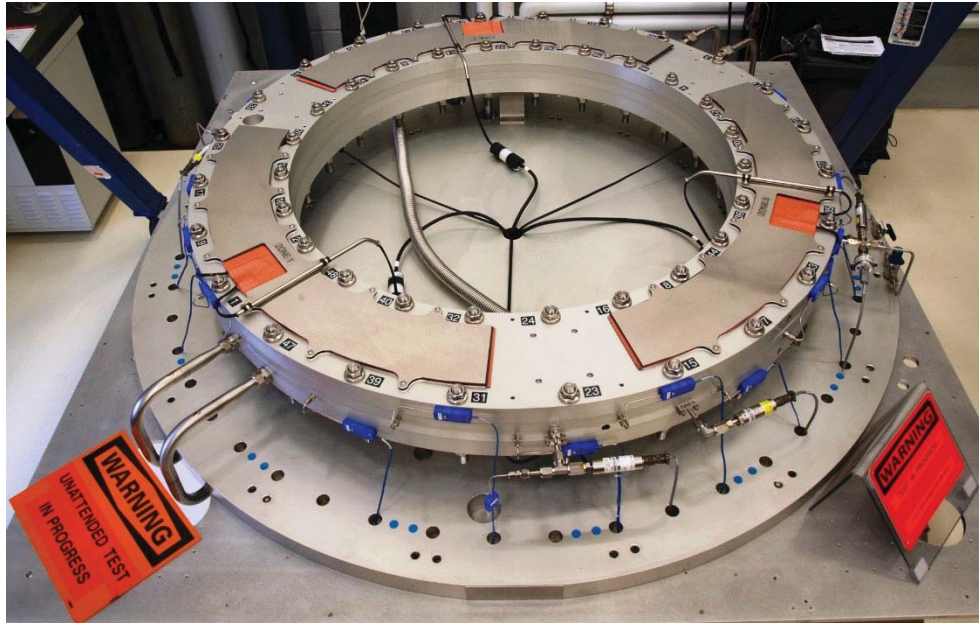
Figure 19.—Full-scale seal leak test fixture.
