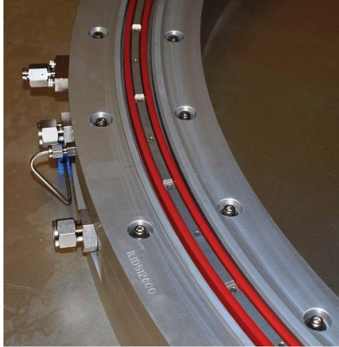
Figure 21.—Full-scale seal installed in lower test assembly of full-scale seal leak test fixture.
