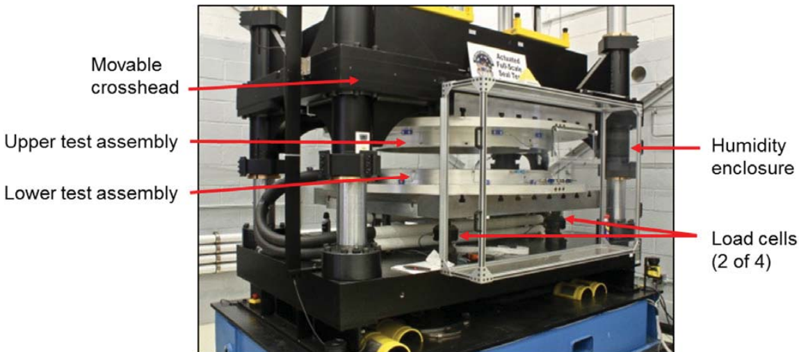
Figure 22.—Full-scale seal compression/adhesion test fixture.
