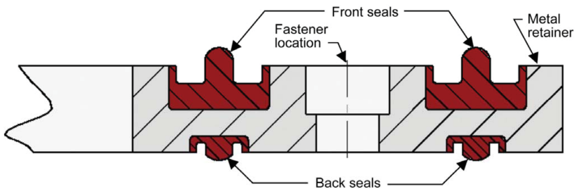
Figure 3.—Cross section through Gask-O-seal showing silicone seals molded into grooves on front and back surfaces of metal retainer.
