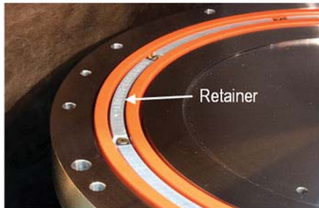
Figure 6.—Photograph of subscale multi-piece seal installed in groove in test apparatus.
