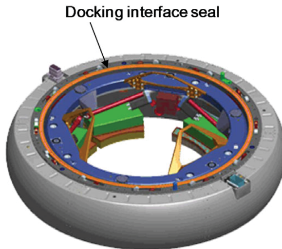
Figure 2.—Docking interface seal location.
