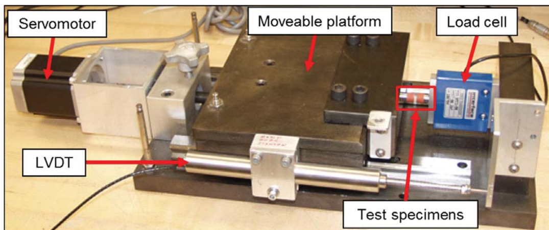
Figure 11.—Small-scale compression/adhesion test fixture.
