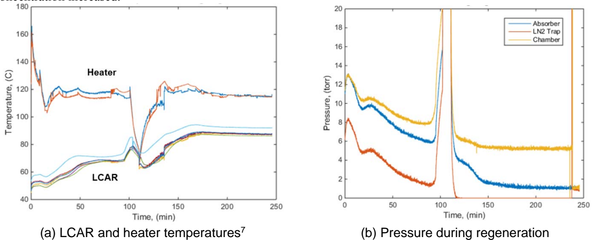
Figure 13. Honeycomb LCAR Regeneration
