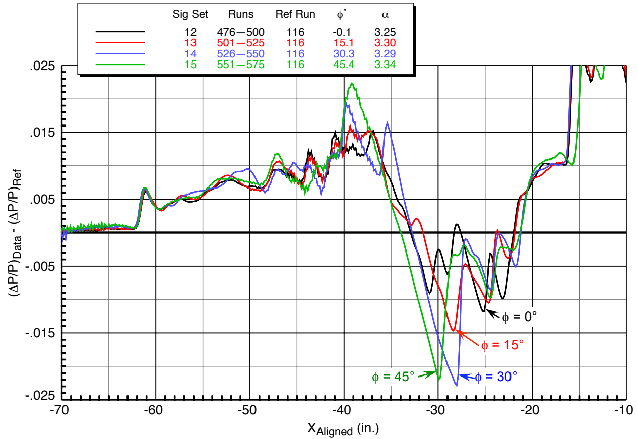
Figure 7–47. Effect of off-track angle for Performance sting+contour model, Z sweeps (59” to 65”) 9x7 TBC4 test, 14-in. aft rail, M = 1.80 , HumidAvg = 237 ppm
