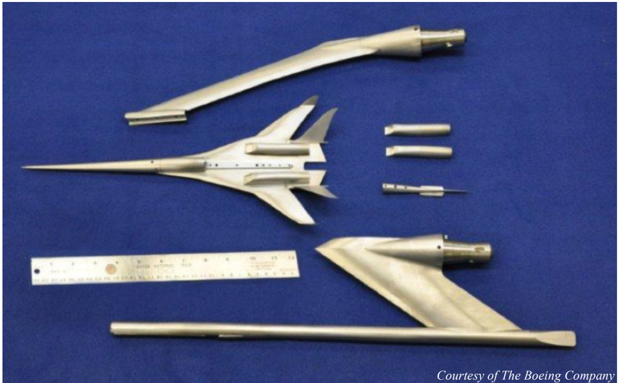
Figure 4–18. Photograph of Boom3 model, interchangeable parts, and VS3 and VS4 struts
