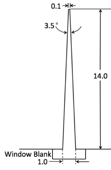
Figure 5–1. Cross section of RF1 rail (dimensions in inches)
