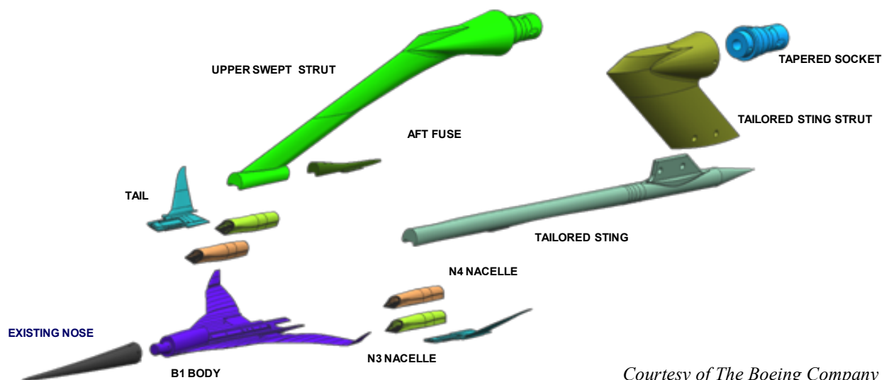
Figure 4–17. CAD views of Boom3 model, interchangeable parts, and VS3 and VS4 struts
