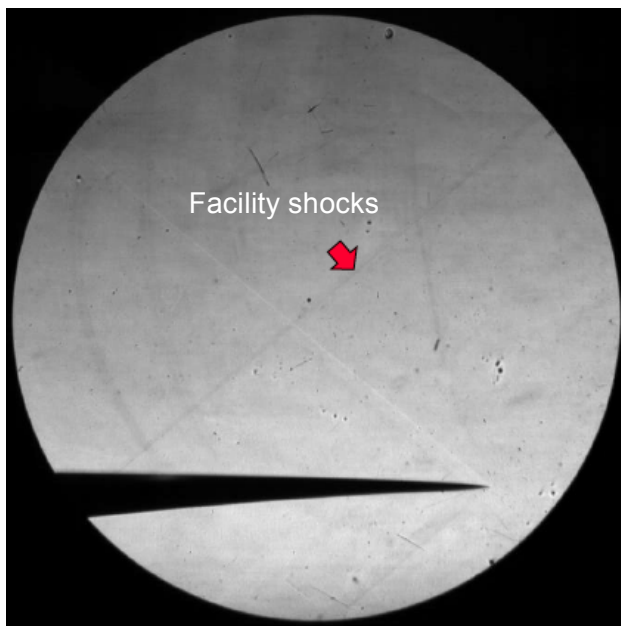
(c) Performance model, Mach 1.6
