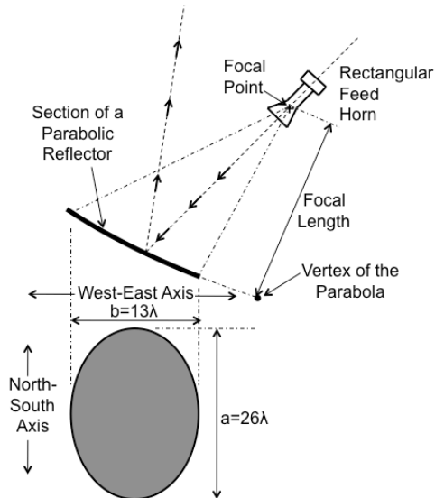
Figure 2. Schematic illustrating the geometry and layout of the beacon antenna. At 39 GHz, a = 200 mm & b = 100 mm.
