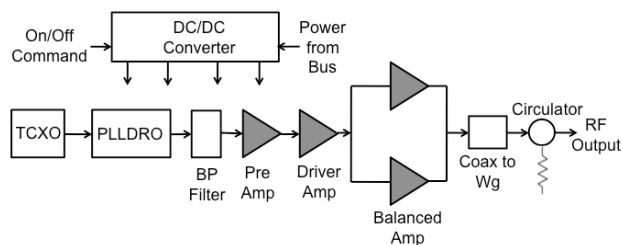
Figure 1. Q-band satellite beacon transmitter block diagram.
