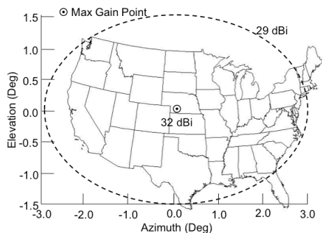
Figure 3. Satellite beacon antenna notional far-field contoured radiation pattern with gain >29 dBi over the coverage area.
