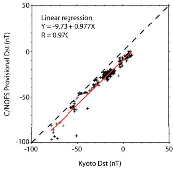
Figure 11. Comparison between the Kyoto Dst index and the provisional Dst index determined from the C/NOFS magnetic field data for the July 22, 2009 magnetic storm. (Adapted from Le et al. [2011])
