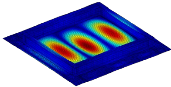
(3,1) 486 Hz FE / 487 Hz Exp
