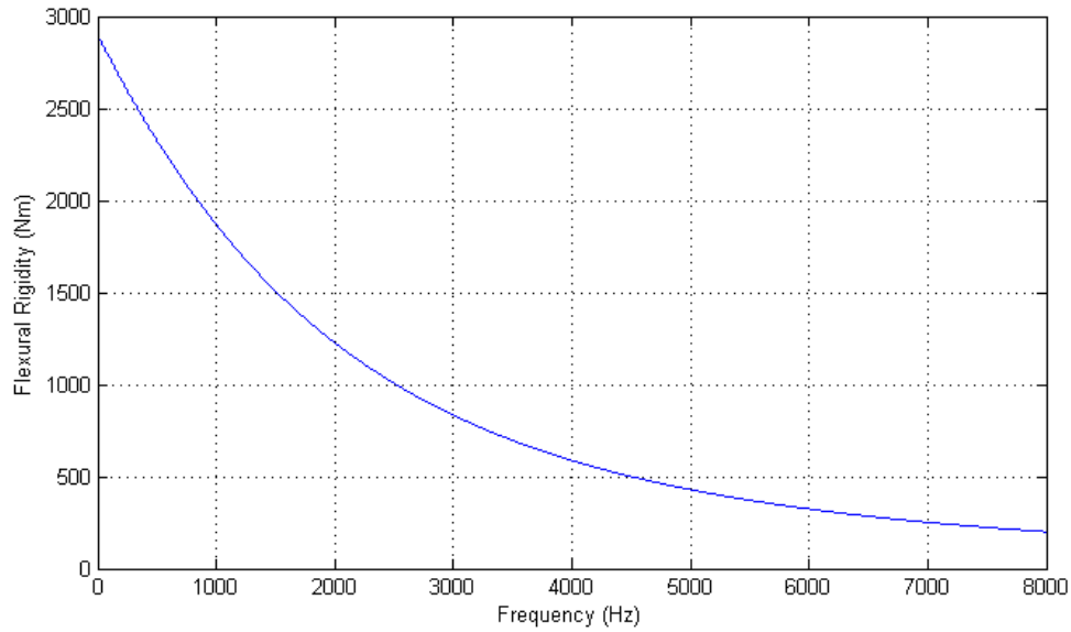
Figure 54: Equivalent flexural rigidity from the wave speed based on a thick-plate model.
