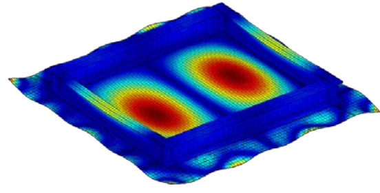
(2,1) 251 Hz FE / 247 Hz Exp
