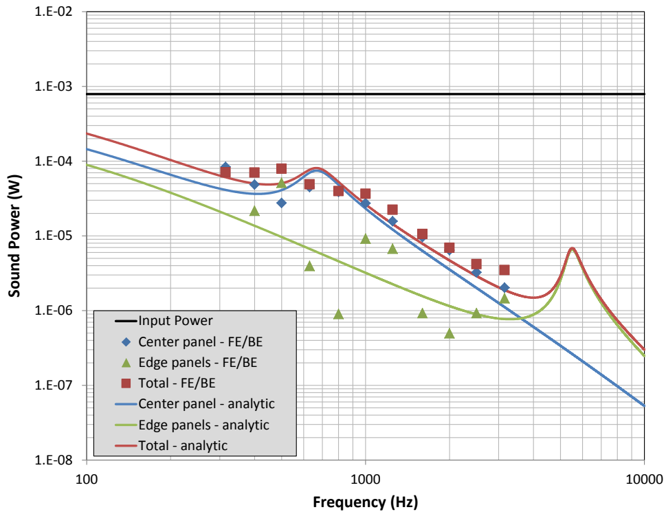
Figure 31. Simulated input and radiated sound power.
