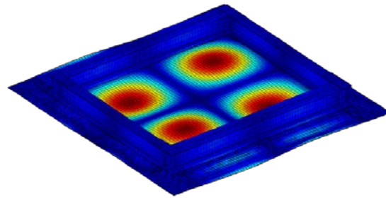
(2,2) 426 Hz FE / 438 Hz Exp
