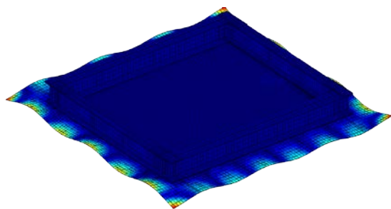
Figure 18. Example of mode shapes in edge material; left image zooms on edge material.
