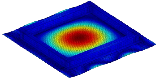
(1,1) 127 Hz FE / 122 Hz Exp
