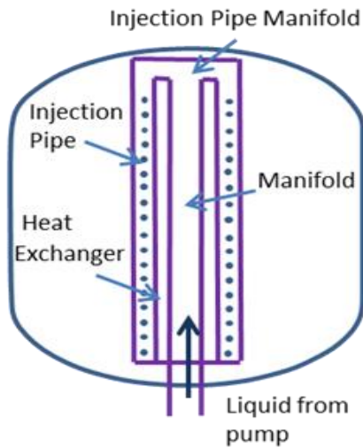
Spray Bar
