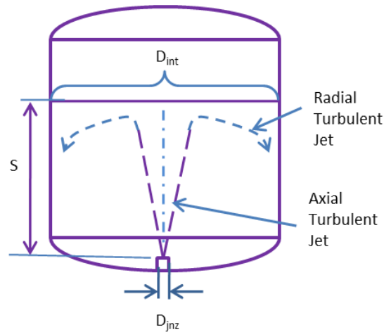
Axial Jet
