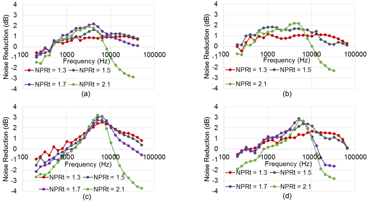
Figure 7.—The noise reduction for NPR_c = NPR_b = 1.8 , NTR_c = 3.0 and M_{ij} = 0.3 at an observation angle of 140^\circ . The data are for (a) A_b/A_c = 2.5 and A_i/A_c = 1.0 , (b) A_b/A_c = 2.5 and A_i/A_c = 0.6 , (c) A_b/A_c = 1.0 and A_i/A_c = 1.0 , and (d) A_b/A_c = 1.0 and A_i/A_c = 0.6 .
