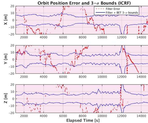
Figure 11. Orbit Position Performance
