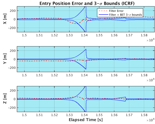
Figure 15. Entry Position Performance
