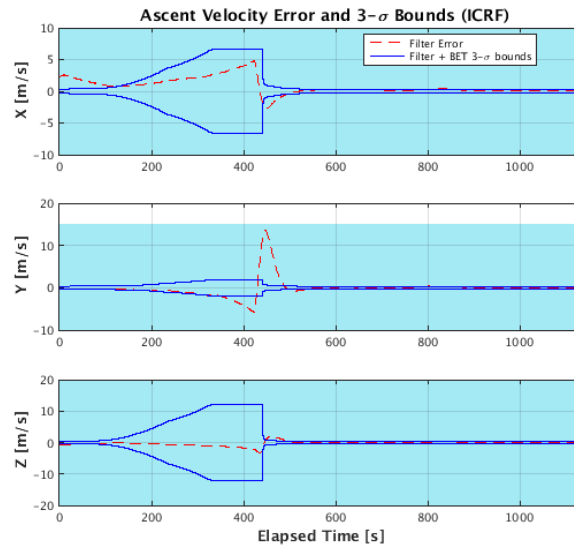
Figure 7. Ascent Velocity Performance
