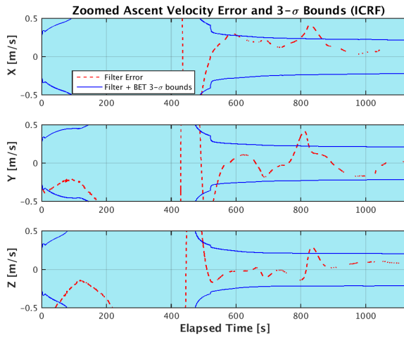
Figure 8. Zoomed Ascent Velocity Performance
