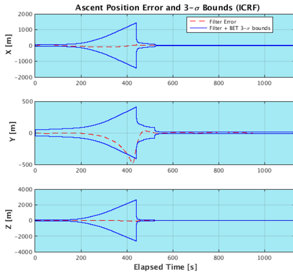
Figure 5. Ascent Position Performance
