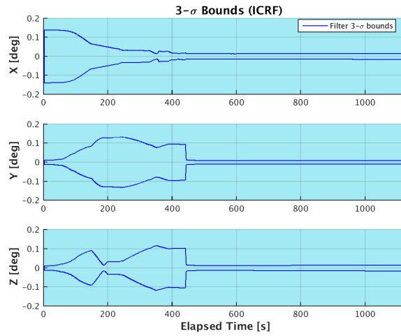
Figure 9. Ascent Attitude Performance
