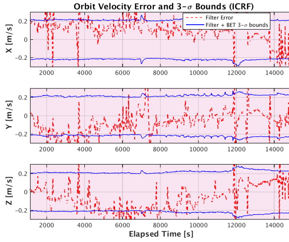
Figure 12. Orbit Velocity Performance
