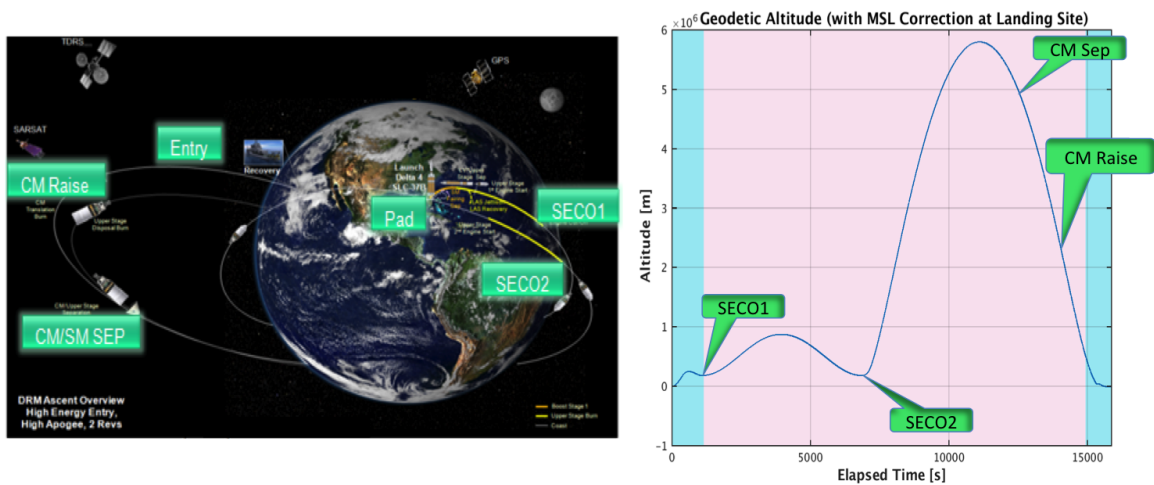
Figure 1. Orion EFT-1 Trajectory Overview and Flight Altitude Profile
