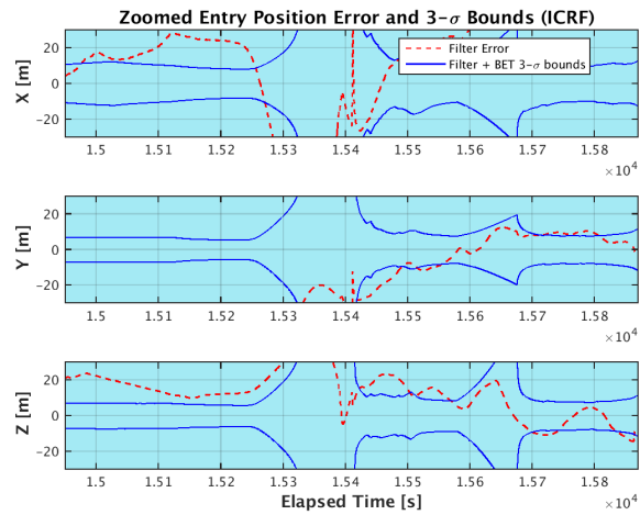
Figure 16. Zoomed Entry Position Performance
