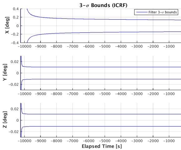
Figure 4. Ground Align Attitude Performance
