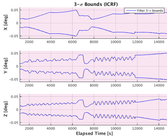
Figure 14. Orbit Attitude Performance
