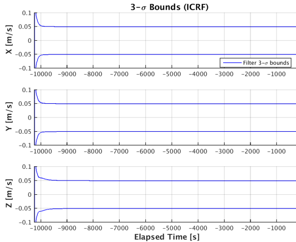
Figure 3. Ground Align Velocity Performance
