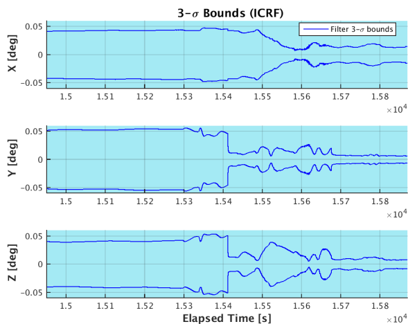
Figure 19. Entry Attitude Performance
