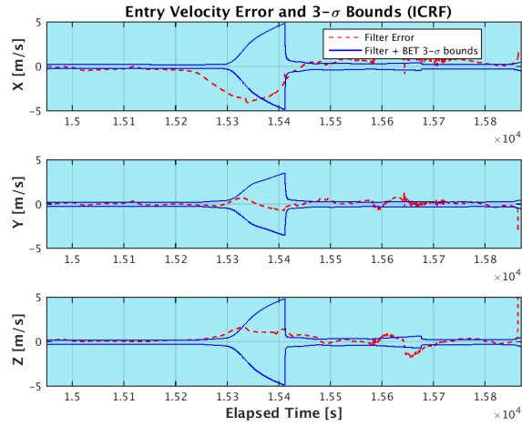
Figure 17. Entry Velocity Performance
