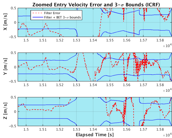
Figure 18. Zoomed Entry Velocity Performance
