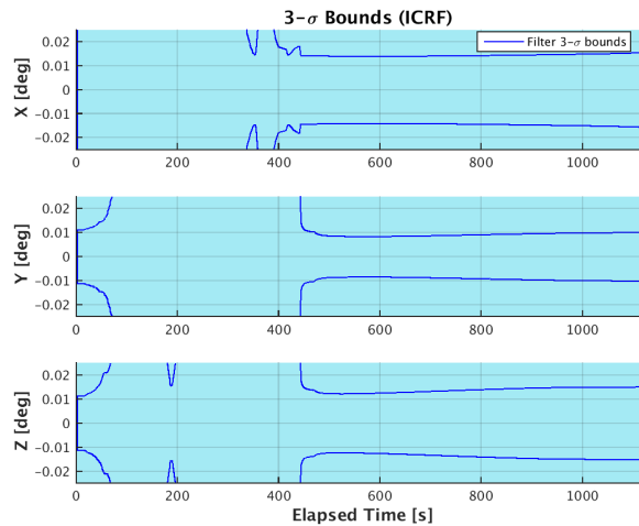
Figure 10. Zoomed Ascent Attitude Performance
