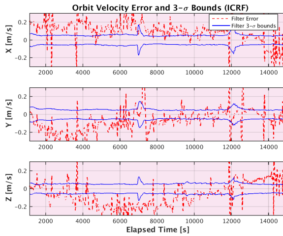
Figure 13. Orbit On-board Filter Velocity Uncertainty
