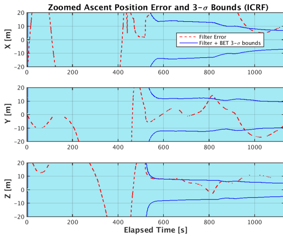
Figure 6. Zoomed Ascent Position Performance
