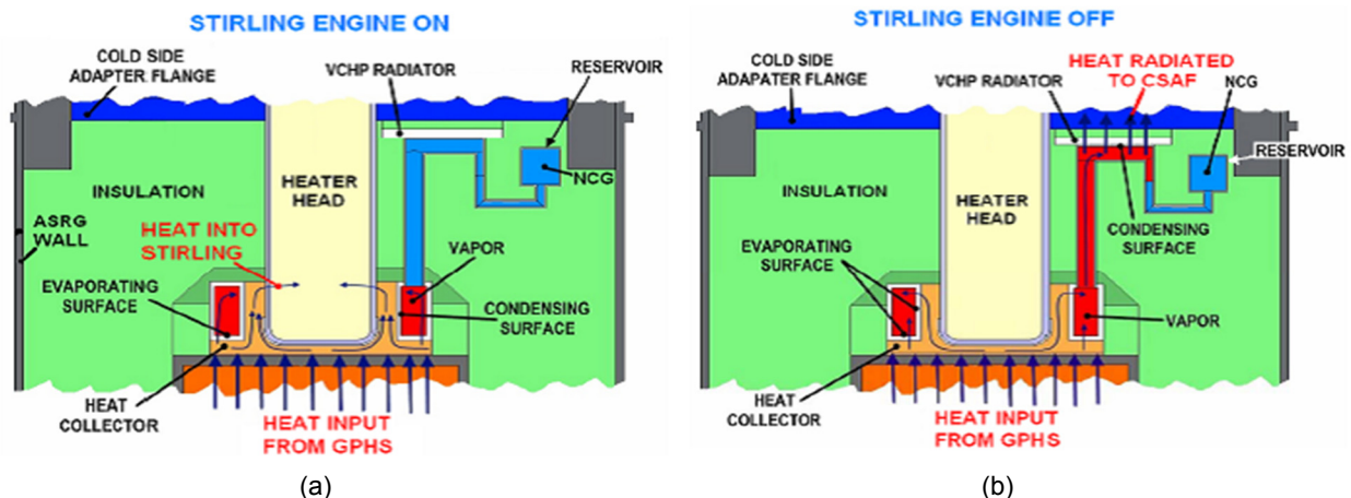
Figure 1.—Advanced Stirling Radioisotope Generator (ASRG) backup cooling concept. The front location is depicted for an operating convertor (a) and a nonoperating convertor (b) (Ref. 3).
