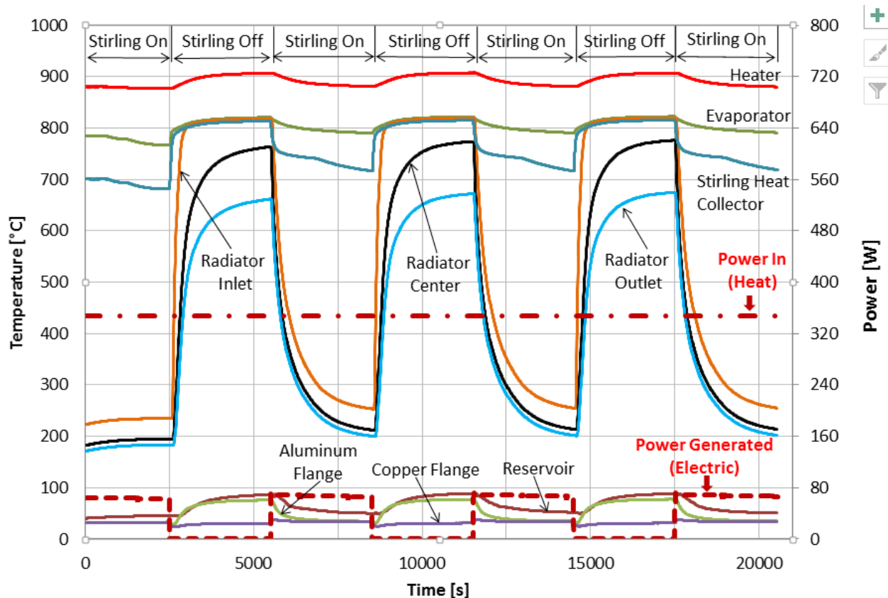
Figure 13.—Experimental results for the multiple short-duration stoppages testing of the Stirling convertor with variable conductance heat pipe (VCHP).
