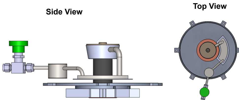
Figure 5.—Variable conductance heat pipe (VCHP) layout side and top views.
