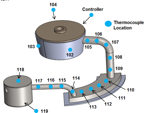
Figure 8.—Variable conductance heat pipe (VCHP) thermocouple (TC) map.
