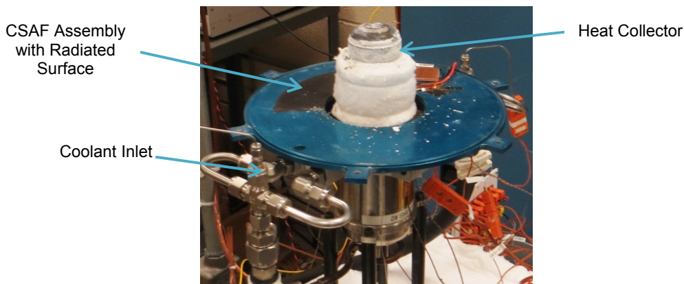
Figure 2.—Stirling convertor used for evaluating the variable conductance heat pipe (VCHP) performance. CSAF is cold-side adaptor flange.
