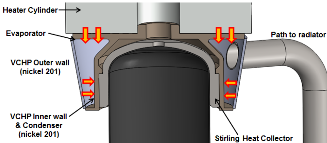
Figure 3.—Cross section of the Stirling hot end, variable conductance heat pipe (VCHP) annulus, and heater cylinder after assembly.
