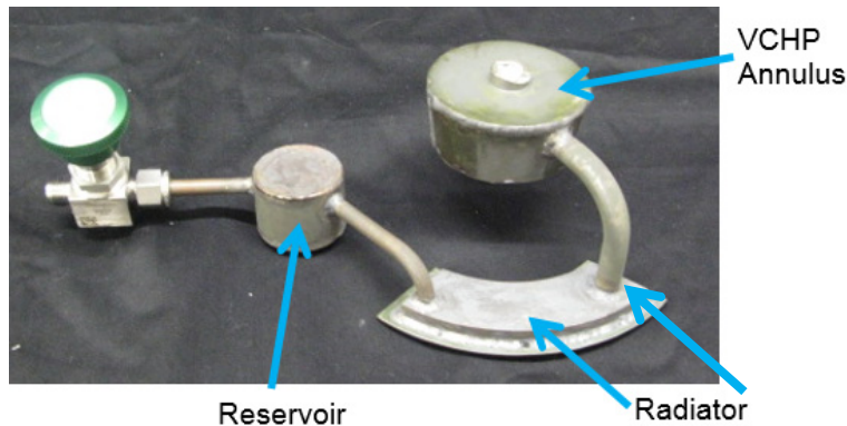
Figure 6.—Variable conductance heat pipe (VCHP) as constructed after heat cycling.
