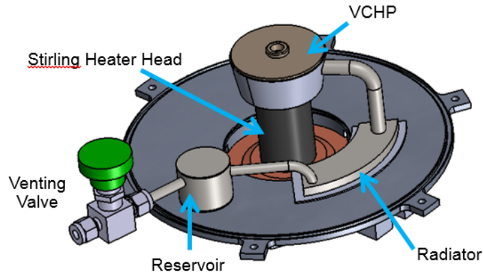
Figure 4.—Variable conductance heat pipe (VCHP) installed on the Stirling converter.
