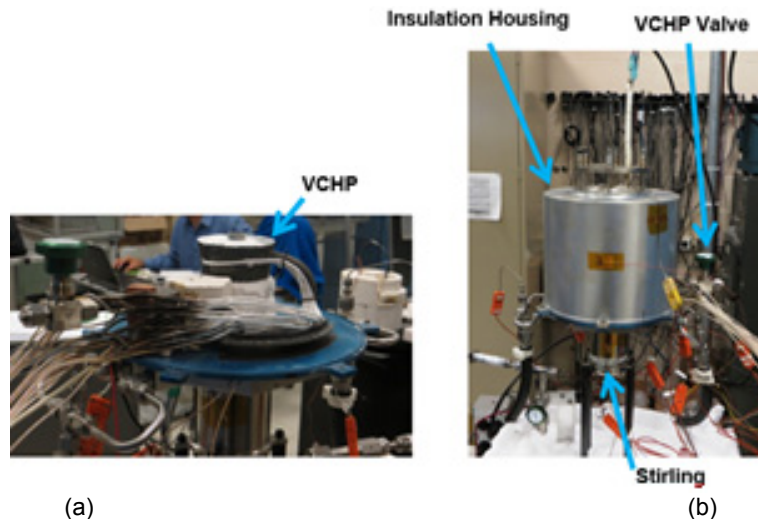
Figure 7.—Testing setup with variable conductance heat pipe (VCHP) and Stirling convertor assembled. (a) VCHP installed on Stirling convertor. (b) VCHP and insulation housing installed on the Stirling convertor.
