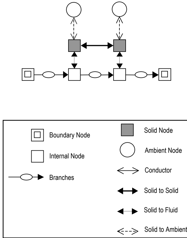
Figure 14. GFSSP network for conjugate heat transfer.
