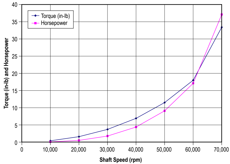
Figure 148. Parametric study results: turbopump torque and horsepower.
