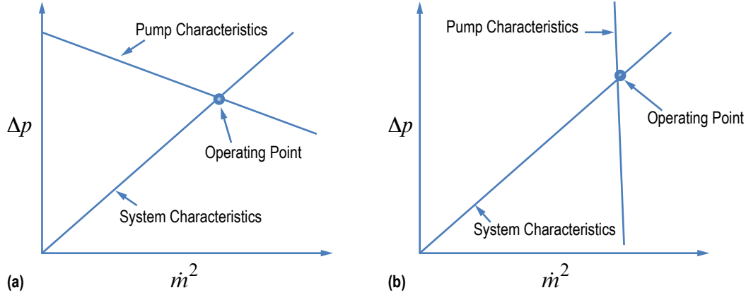
Figure 37. Implementation of fixed flow rate in a branch using pump characteristics: (a) Centrifugal pump and (b) positive displacement pump.
