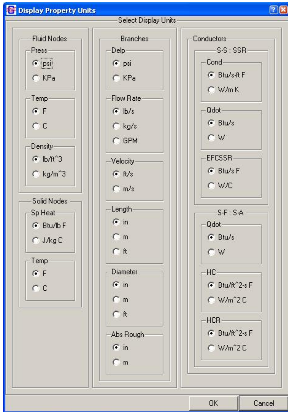
Figure 97. Display Property Units dialog.
