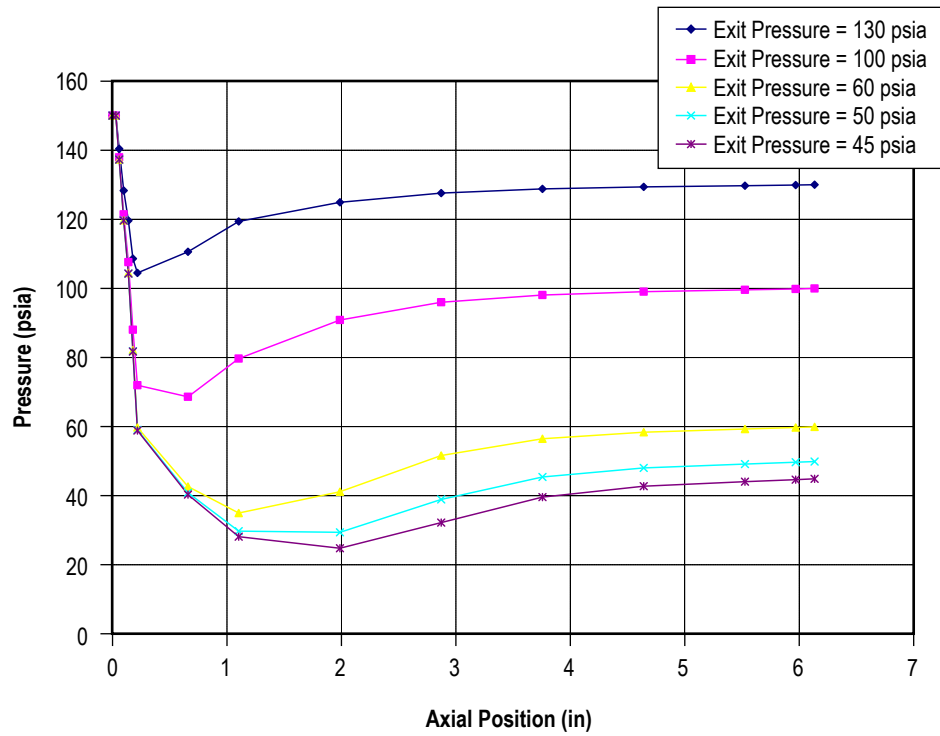
Figure 108. Predicted pressures for the isentropic steam nozzle.
