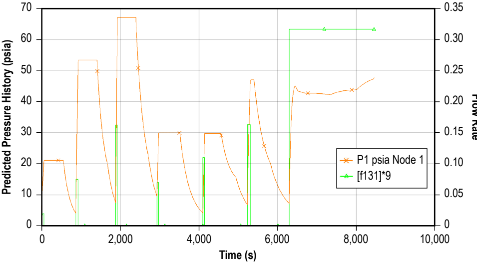
Figure 241. Specified inlet flow rate and predicted pressure history.
