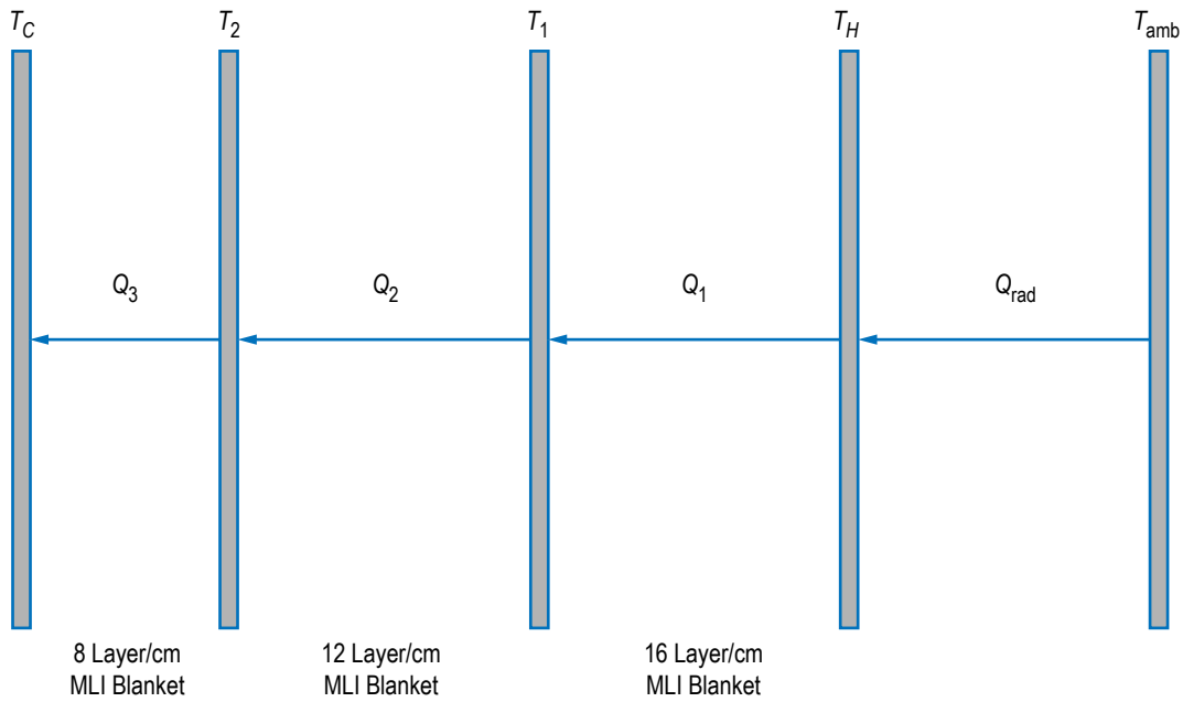
Figure 249. MLI modeling methodology.
