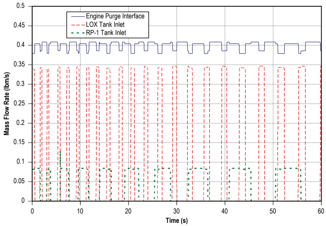
Figure 159 Helium flow rate history.
