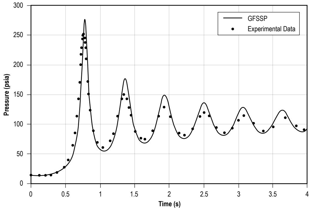
Figure 231. Comparison of GFSSP and experimental data.
