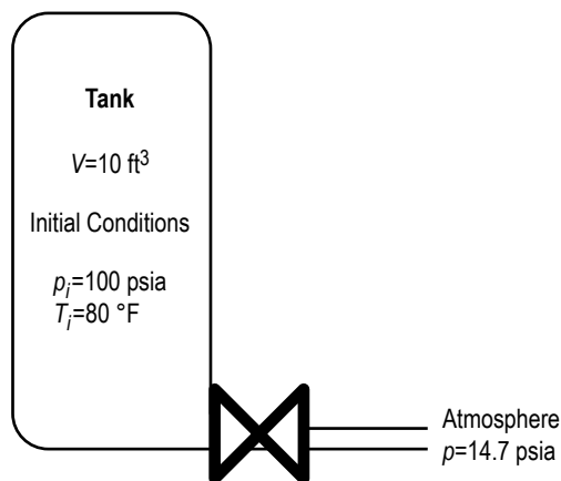
Figure 182. Tank blowdown with flow regulator schematic (example 17).
