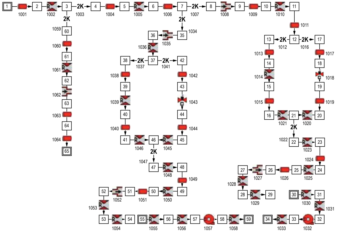
Figure 150. GFSSP model of the pressurization system of example 12: (a) Detailed model schematic and (b) VTASC model.
