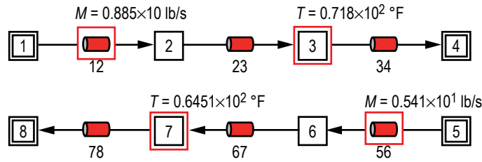
Figure 116. Temperature and flow rate predictions in heat exchanger.
