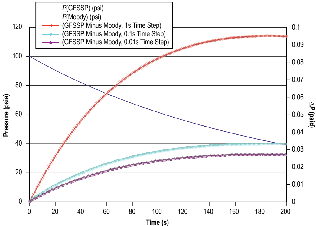
Figure 127. Comparison of the predicted pressure history by GFSSP and the analytical solution.
