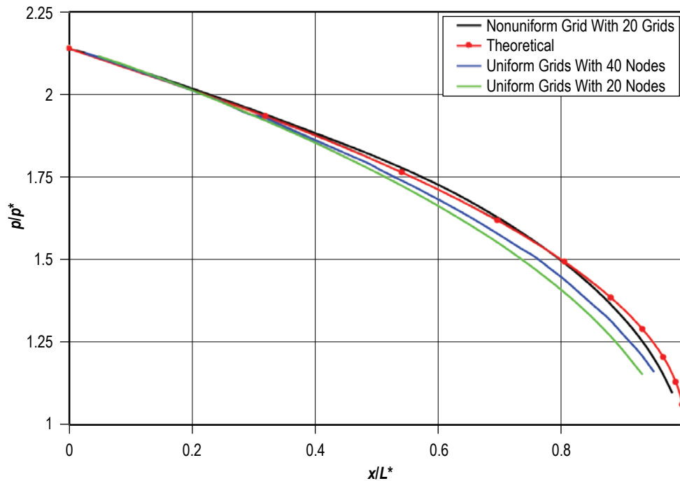
Figure 192. Pressure distribution for Fanno flow with various grid distributions.
