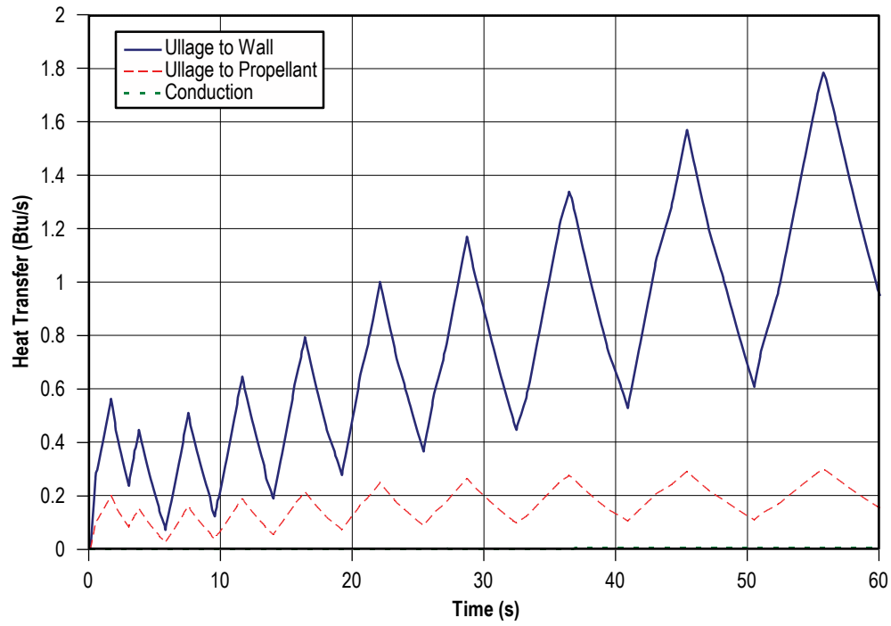
Figure 153. RP-1 heat transfer history.
