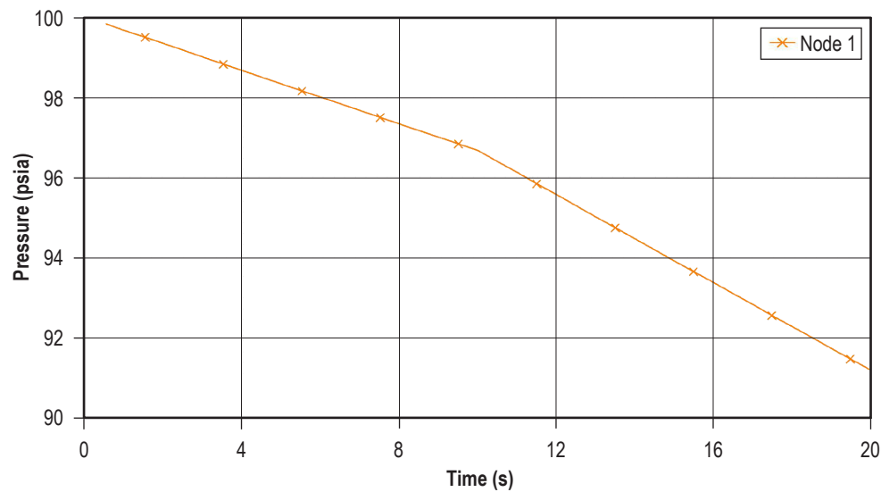
Figure 185. Tank pressure history (example 17).
