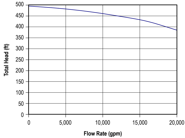
Figure 99. Manufacturer-supplied pump head-flow characteristics.
