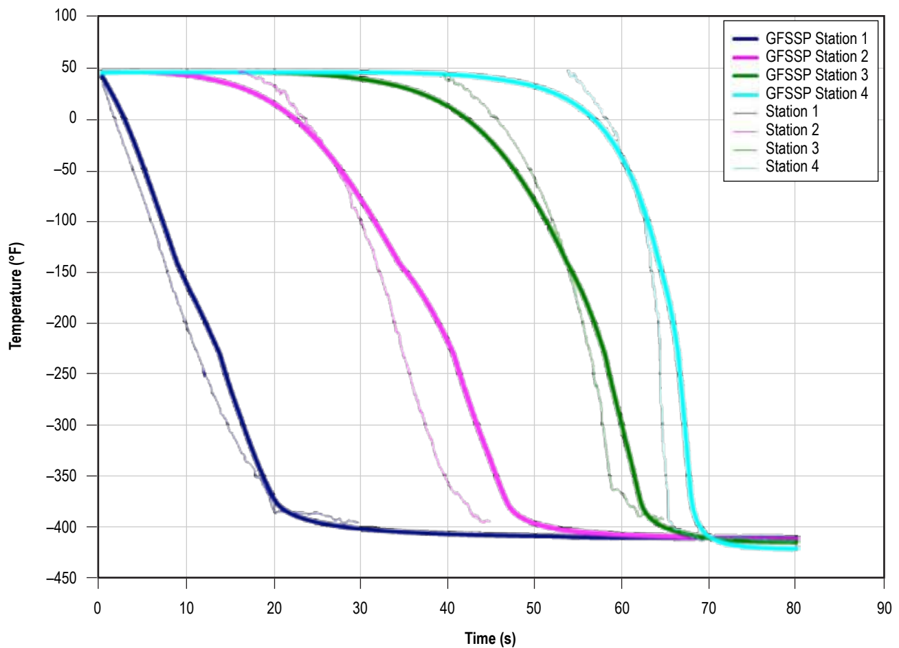
Figure 165. NBS chilldown comparison—GFSSP's predicted solid temperatures (°F) compared to measurements.
