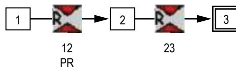
Figure 176. Tank blowdown with pressure regulator VTASC model (example 16).
