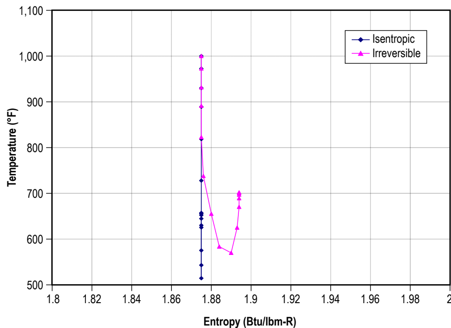
Figure 110. Temperature/entropy plot comparing the isentropic steam nozzle with an irreversible process.
