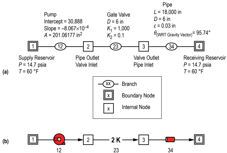
Figure 100. GFSSP model of pumping system and reservoirs: (a) Detailed schematic and (b) VTASC model.
