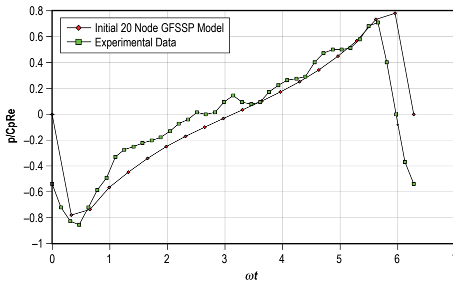
Figure 125. Comparison of GFSSP model results with experimental data or squeeze film damper.
