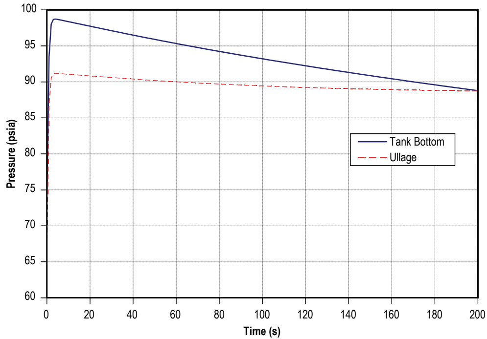
Figure 136. Ullage and tank bottom pressure history.
