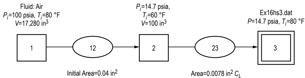
Figure 175. Tank blowdown with pressure regulator detailed model (example 16).
