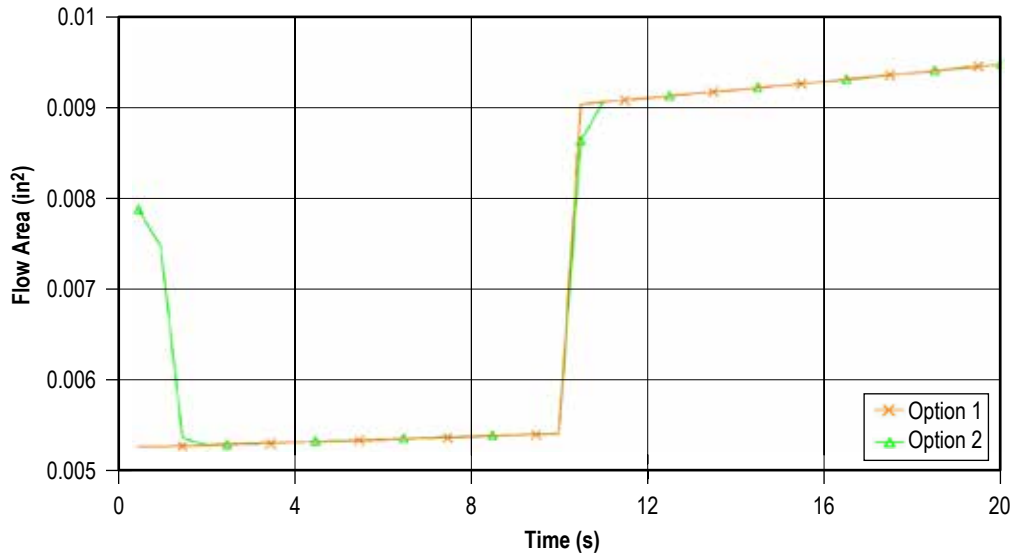
Figure 187. Flow regulator area history (example 17).
