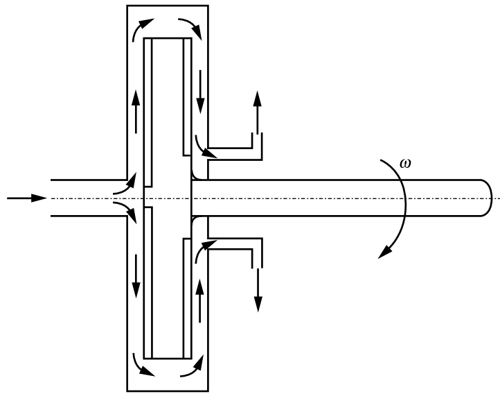
Figure 117. Flow schematic of a rotating radial disk (example 6).
