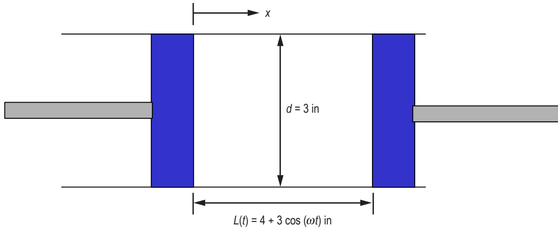
Figure 129. Coordinate transformed piston-cylinder configuration.
