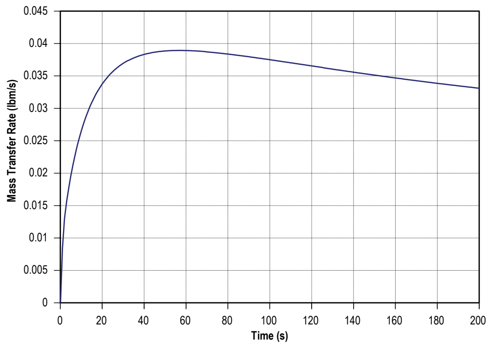
Figure 140. GOX mass transfer rate history.
