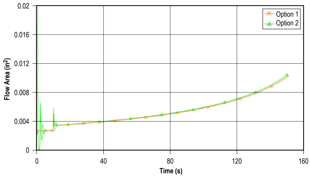
Figure 180. Pressure regulator flow area history (example 16, restrict 12).
