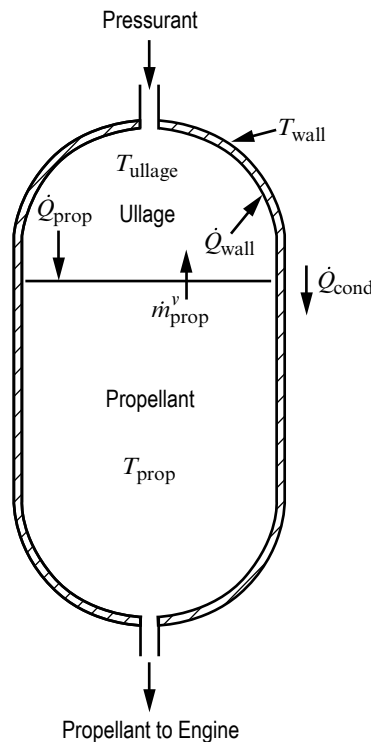
Figure 133. Schematic of propellant tank pressurization system.
