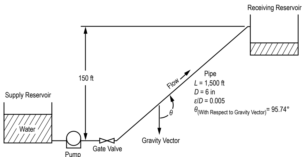
Figure 98. Schematic of pumping system and reservoirs (example 1).
