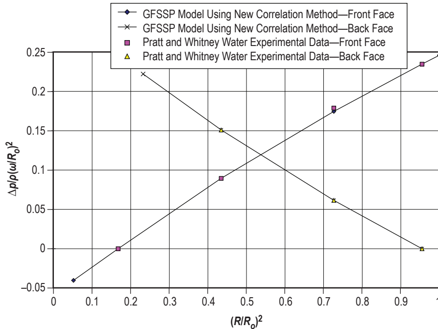
Figure 119. Comparison of GFSSP model results with experimental data.
