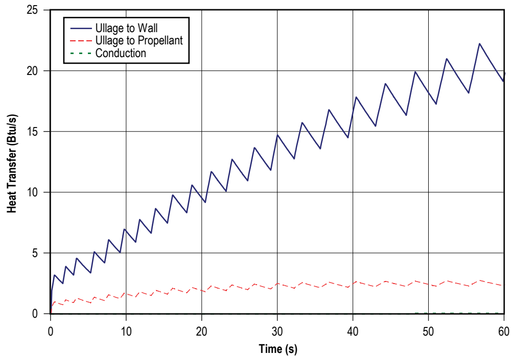
Figure 155. LOX tank heat transfer history.
