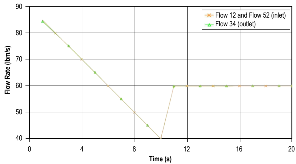
Figure 213. Comparison of inlet and outlet flow rates.
