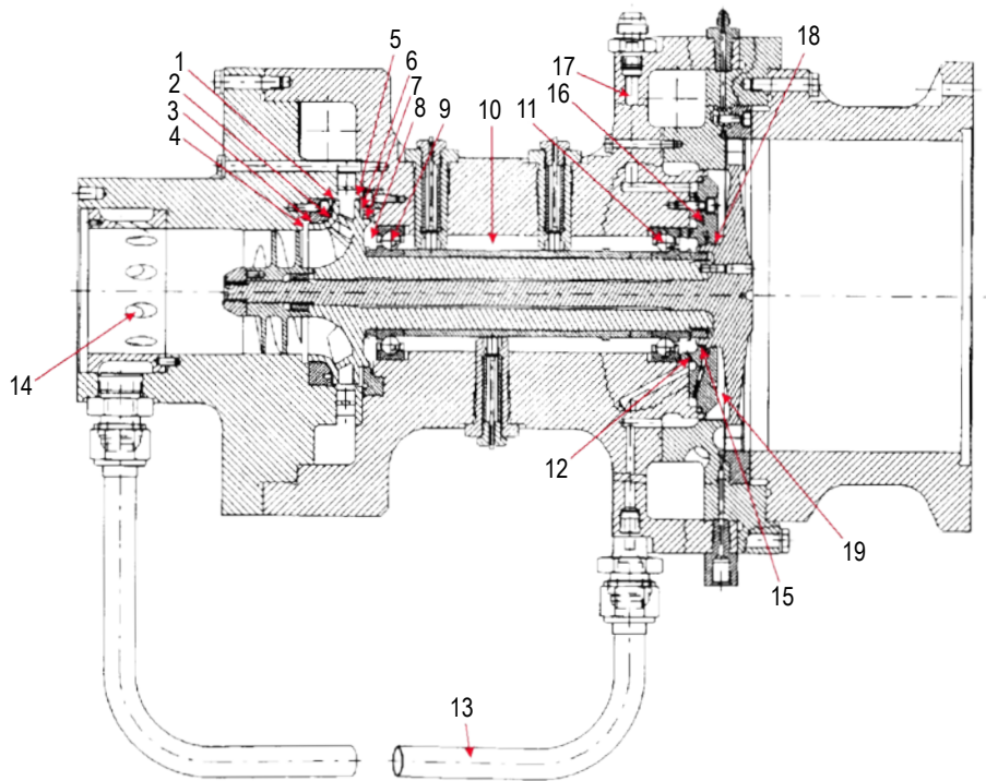
Figure 206. Schematic of the simplex turbopump with secondary flow passages indicated.
