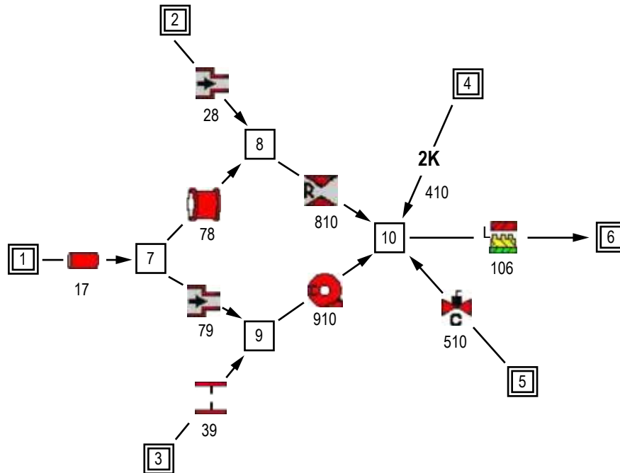
Figure 69. Example fluid circuit with Resistance options.
