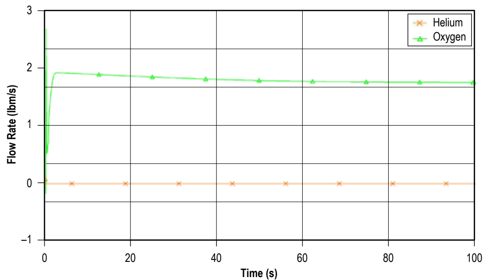
Figure 217. Helium and mixture flow rates.
