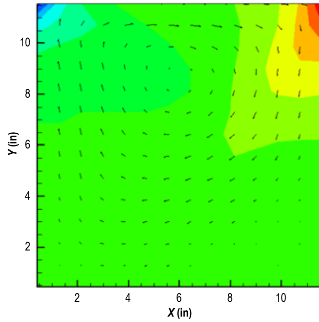
Figure 227. Predicted velocity field and pressure contours.
