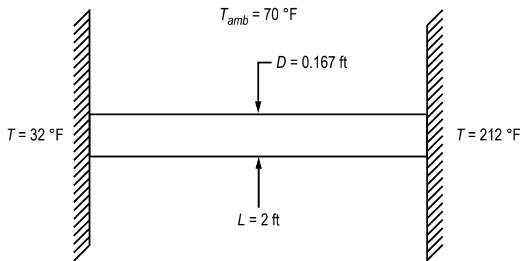
Figure 160. Schematic of circular rod connected to walls at different temperatures.
