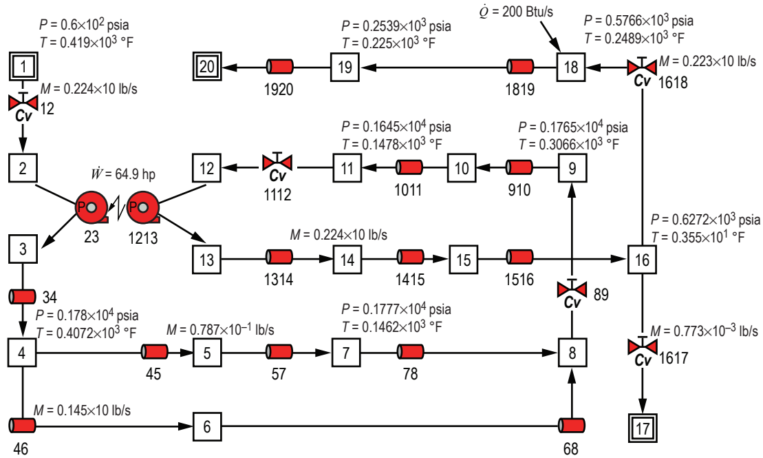
Figure 145. GFSSP RCS model results.
