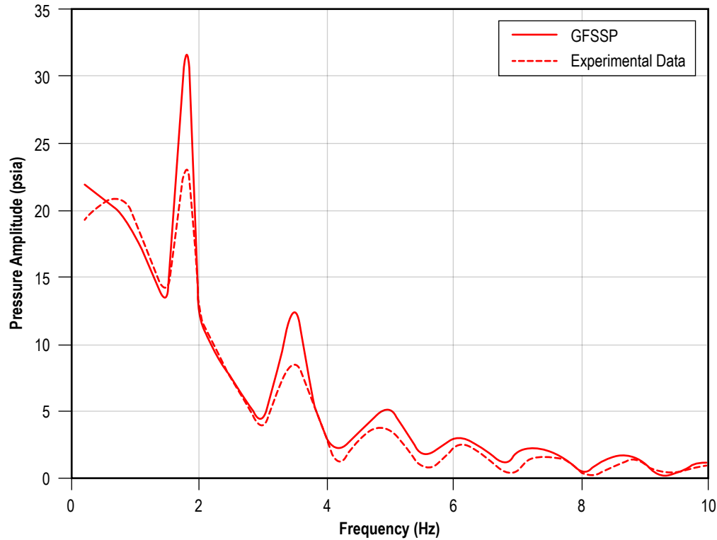
Figure 232. Fast Fourier transform for modal frequencies.
