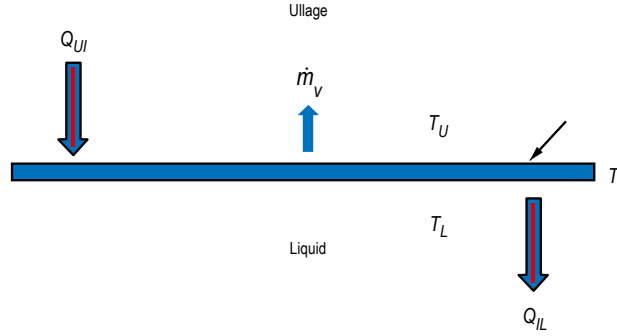
Figure 248. Schematic of evaporative mass transfer process at liquid-vapor interface.
