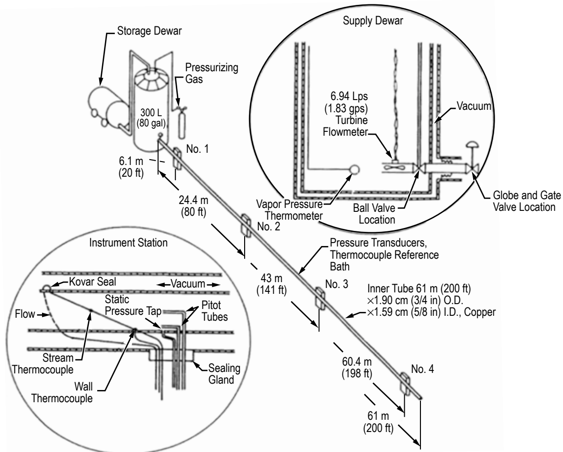
Figure 163. NBS test set-up of cryogenic transfer line.
