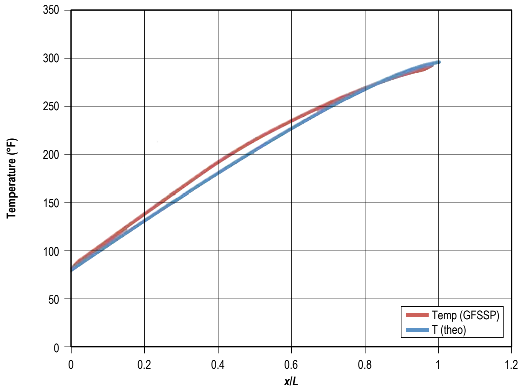
Figure 198. Temperature distribution for Rayleigh flow ( Q = 1,800 Btu/s).
