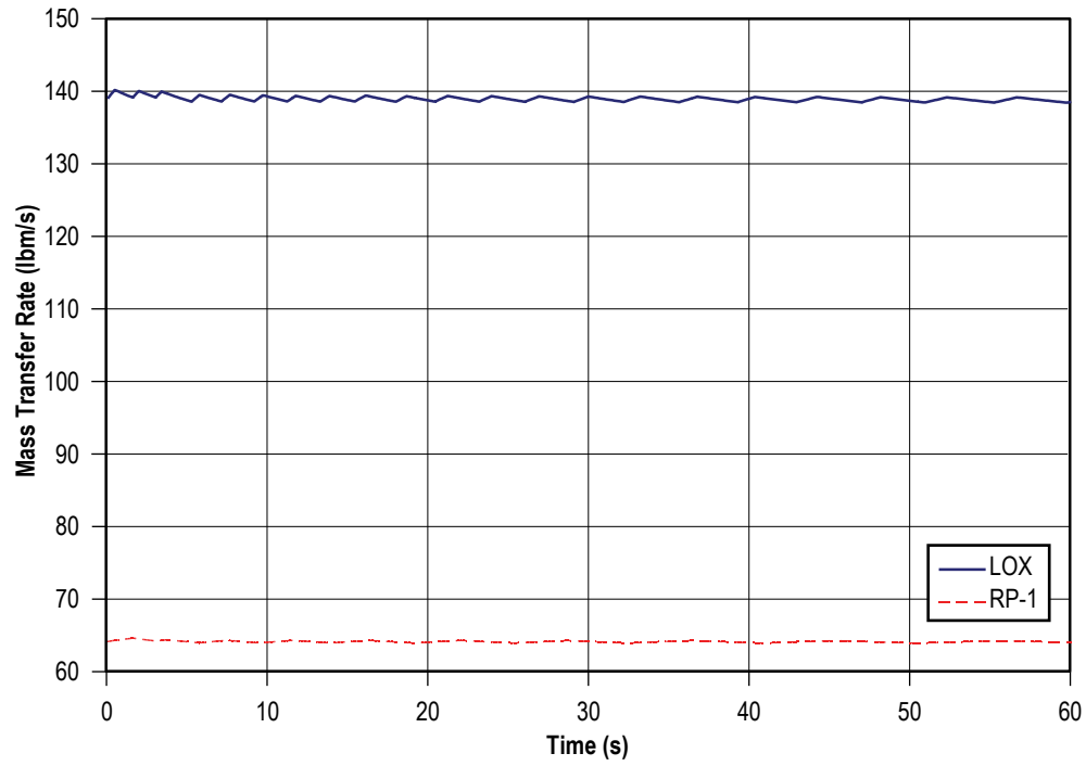
Figure 157. Propellant flow rate history.
