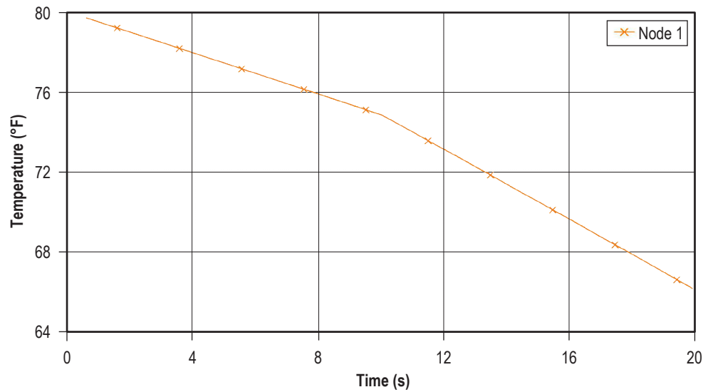
Figure 186. Tank temperature history (example 17).
