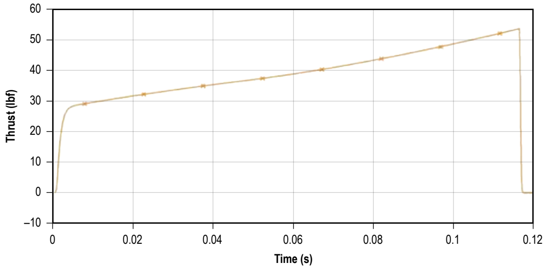
Figure 257. History of thrust during propellant burn and tail-off.
