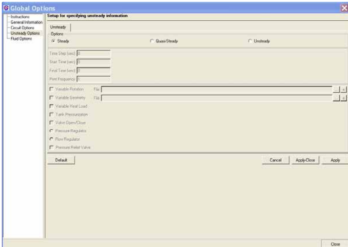
Figure 53. Unsteady Options dialog.
