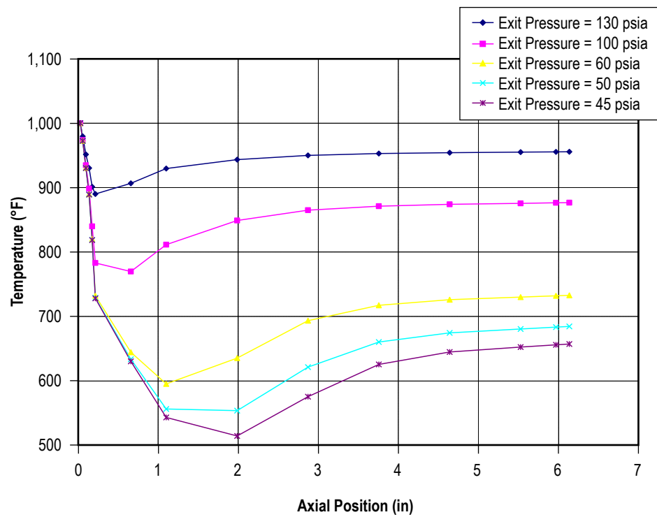
Figure 109. Predicted temperatures for the isentropic steam nozzle.
