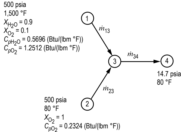
Figure 111. Mixing problem schematic (example 4).
