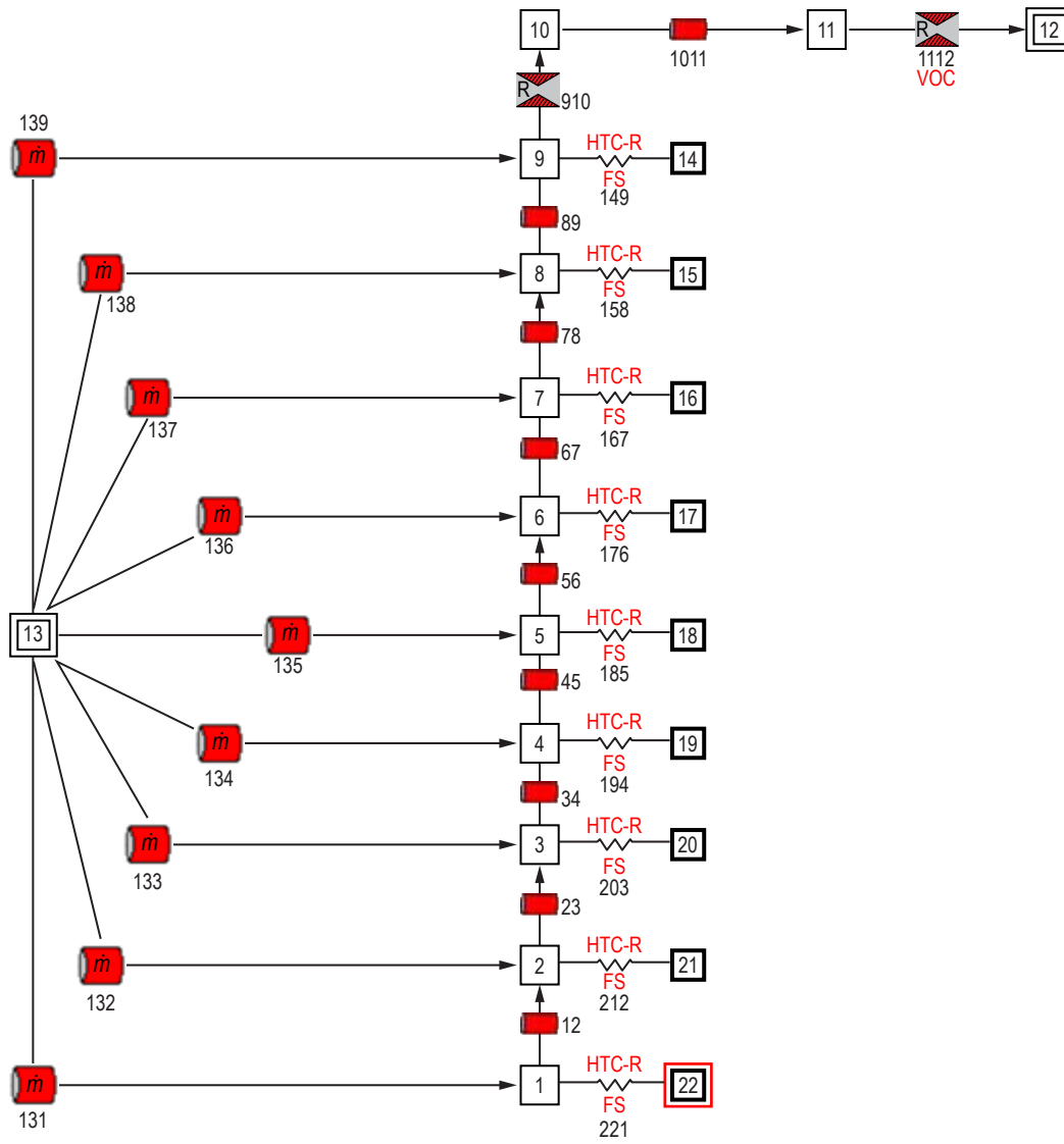
Figure 239. GFSSP nine node tank model.
