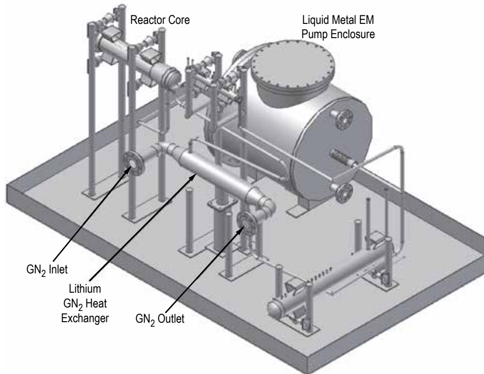
Figure 200. Lithium loop model schematic (example 20).
