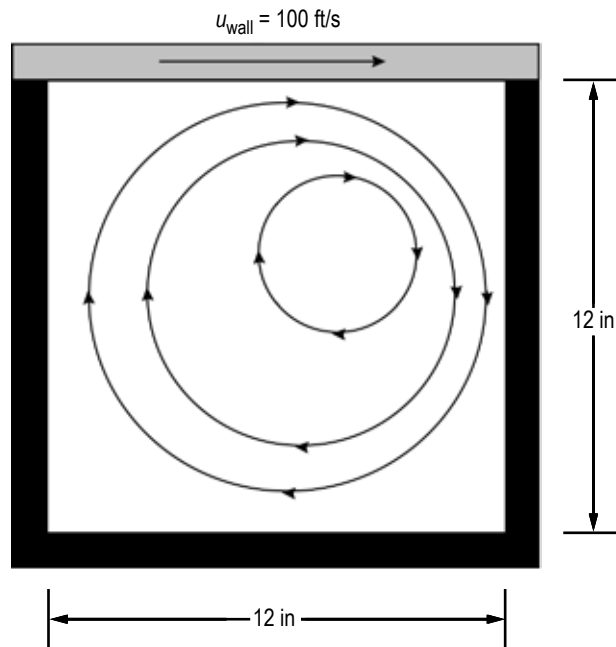
Figure 224. Flow in a shear driven square cavity.
