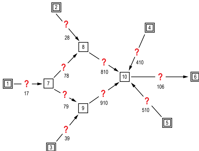
Figure 64. Example fluid circuit with complete branch connections.
