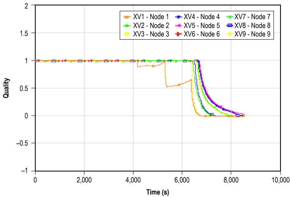
Figure 244. Predicted vapor quality during tank chilldown.
