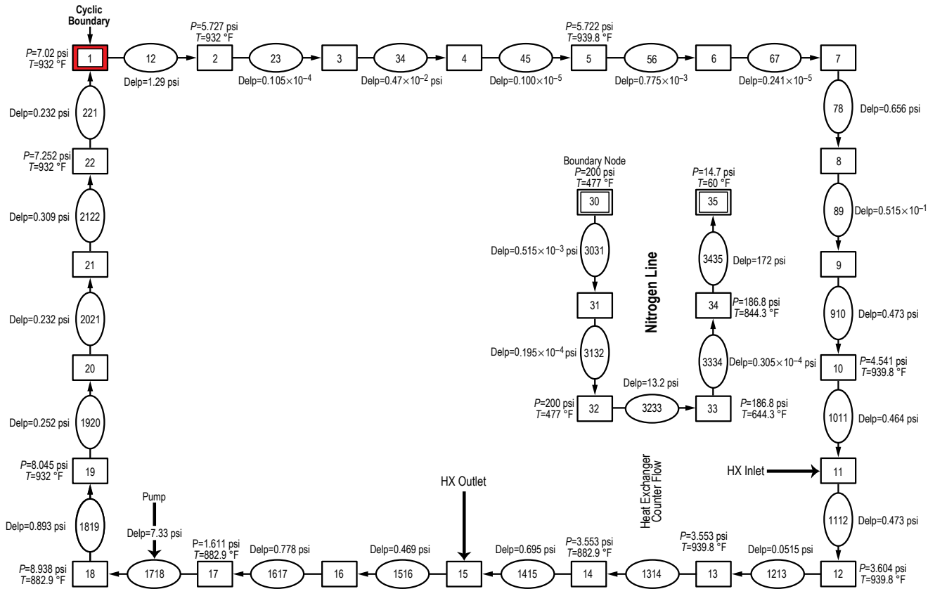
Figure 204. Model results of example 20.
