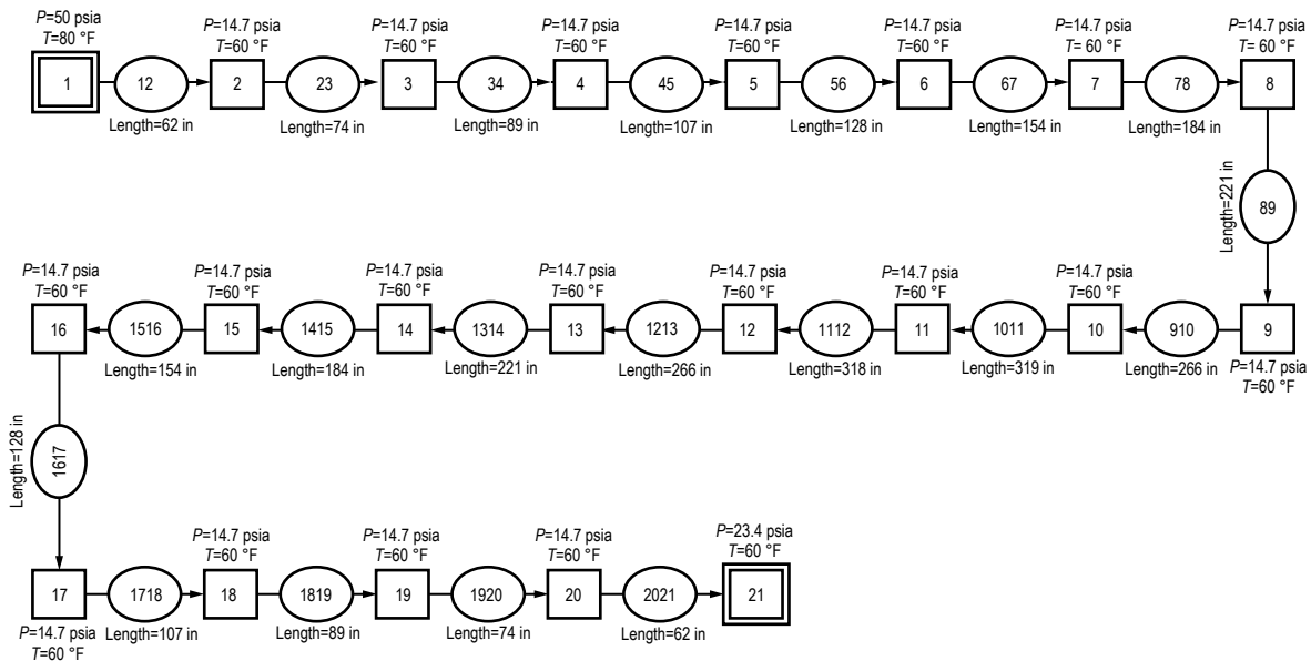
Figure 190. Fanno flow model schematic—fluid: nitrogen.
