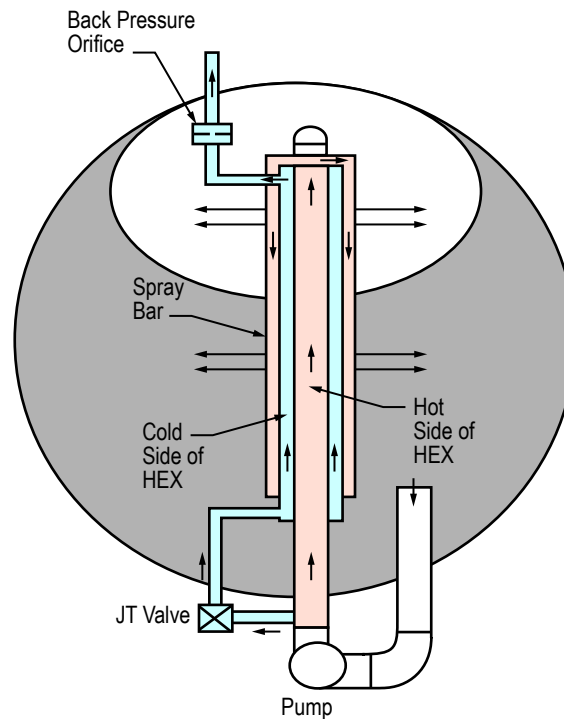
Figure 245. TVS in MHTB tank.
