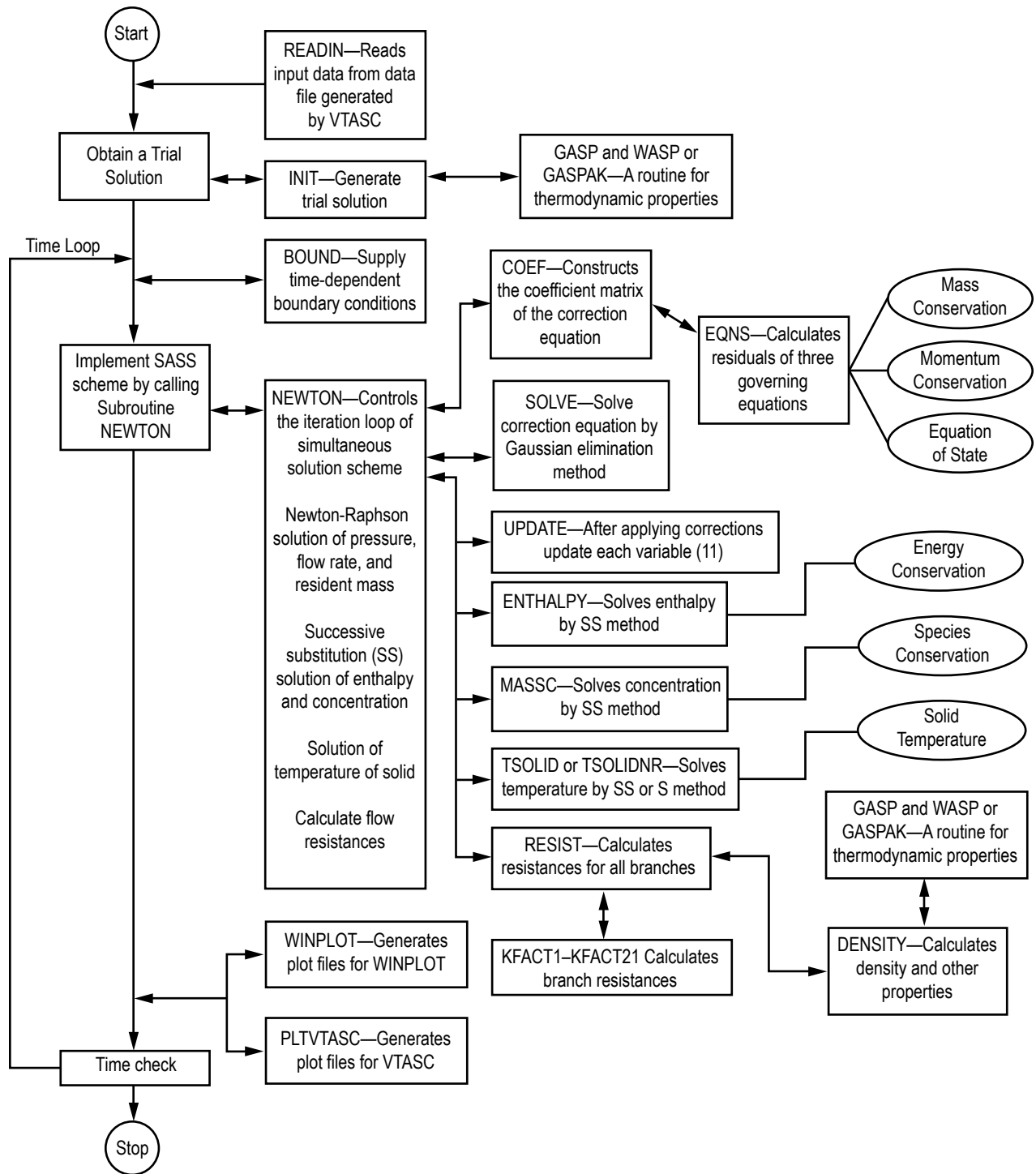
Figure 41. Flowchart of simultaneous solution algorithm in SP module.
