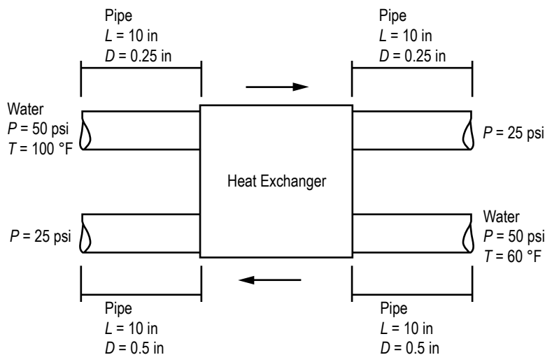
Figure 113. Flow system schematic of a heat exchanger (example 5).
