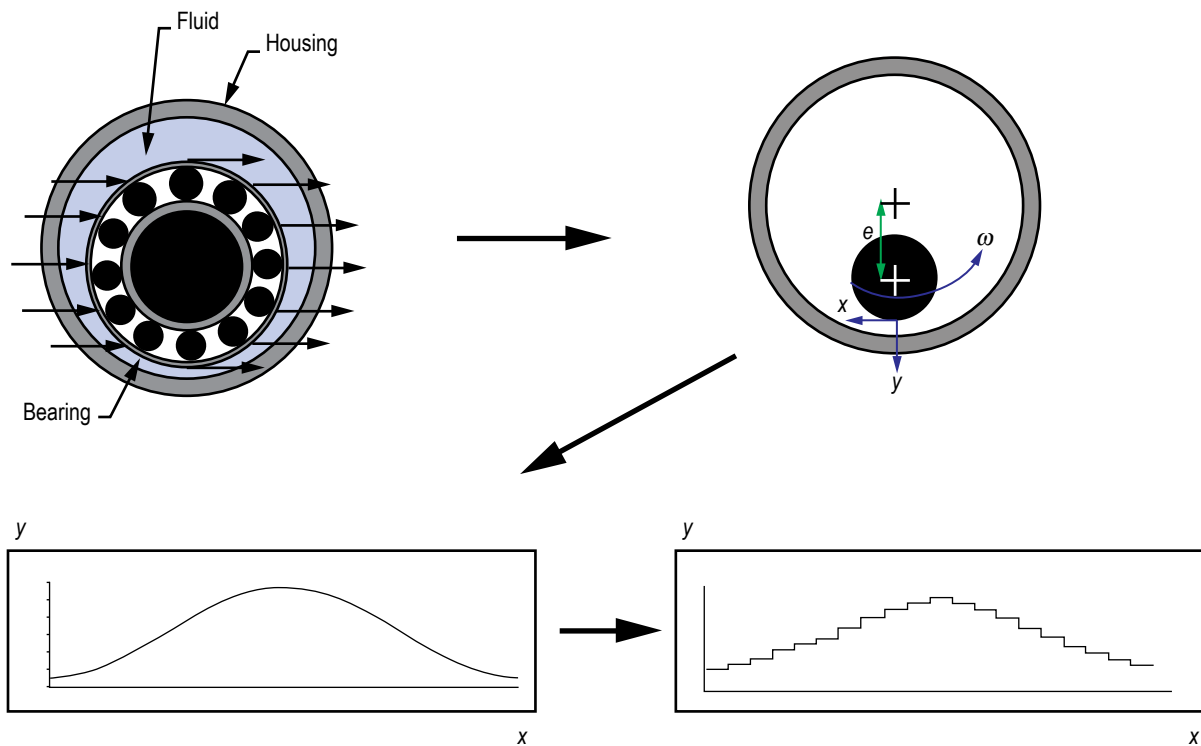
Figure 122. Unwrapping and discretization of squeeze film damper.
