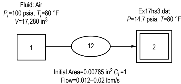
Figure 183. Tank blowdown with flow regulator detailed model (example 17).
