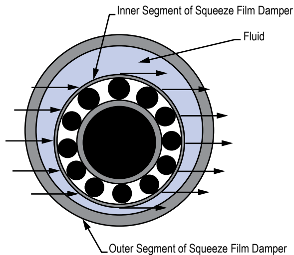
Figure 121. Squeeze film damper schematic (example 7, view 2).
