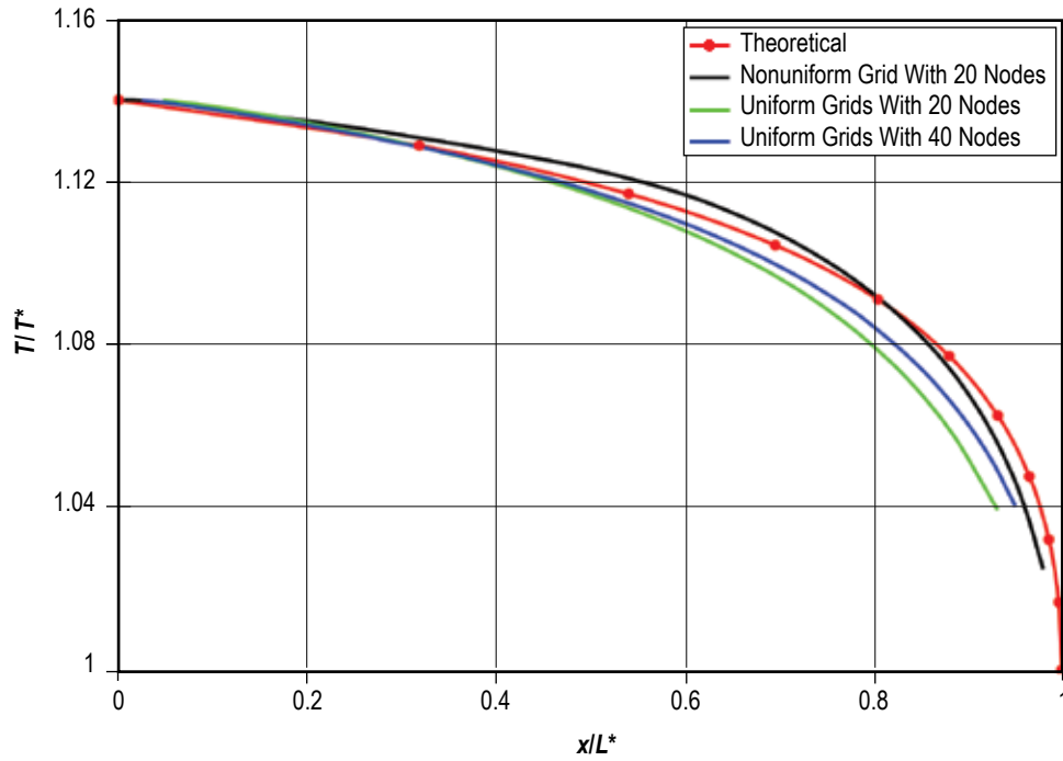
Figure 193. Temperature distribution for Fanno flow with various grid distributions.
