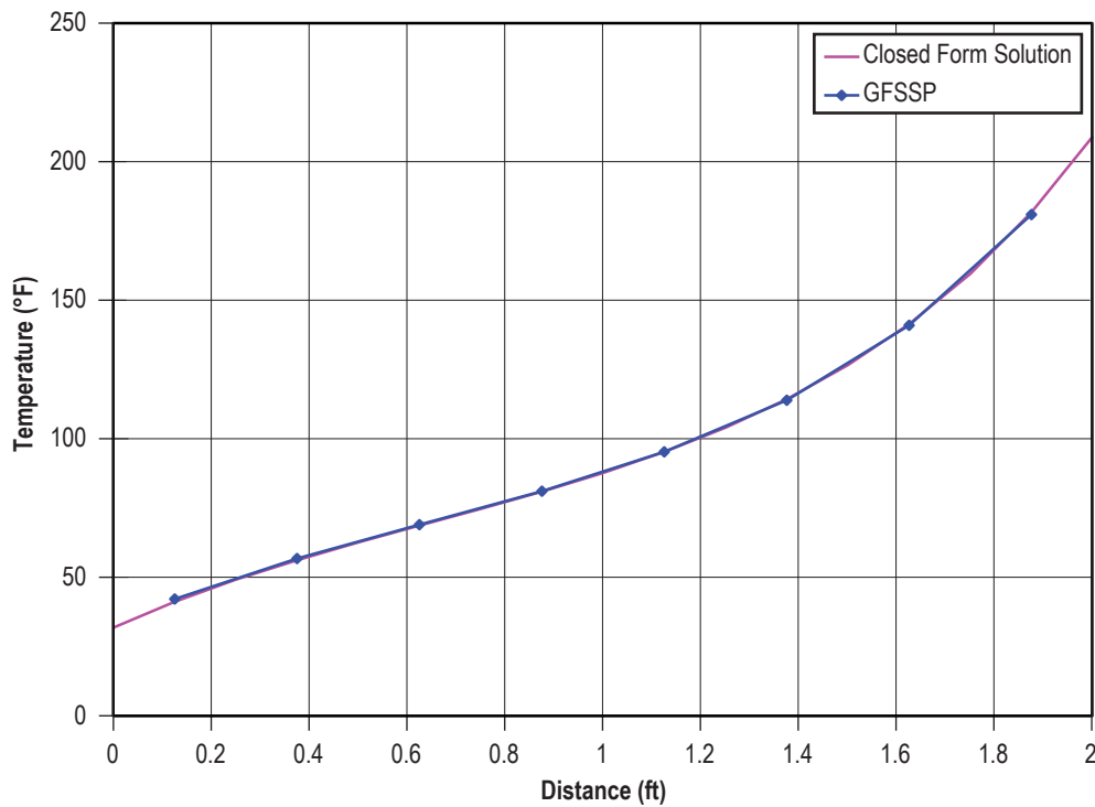
Figure 162. Comparison of GFSSP temperature prediction and closed form solution.
