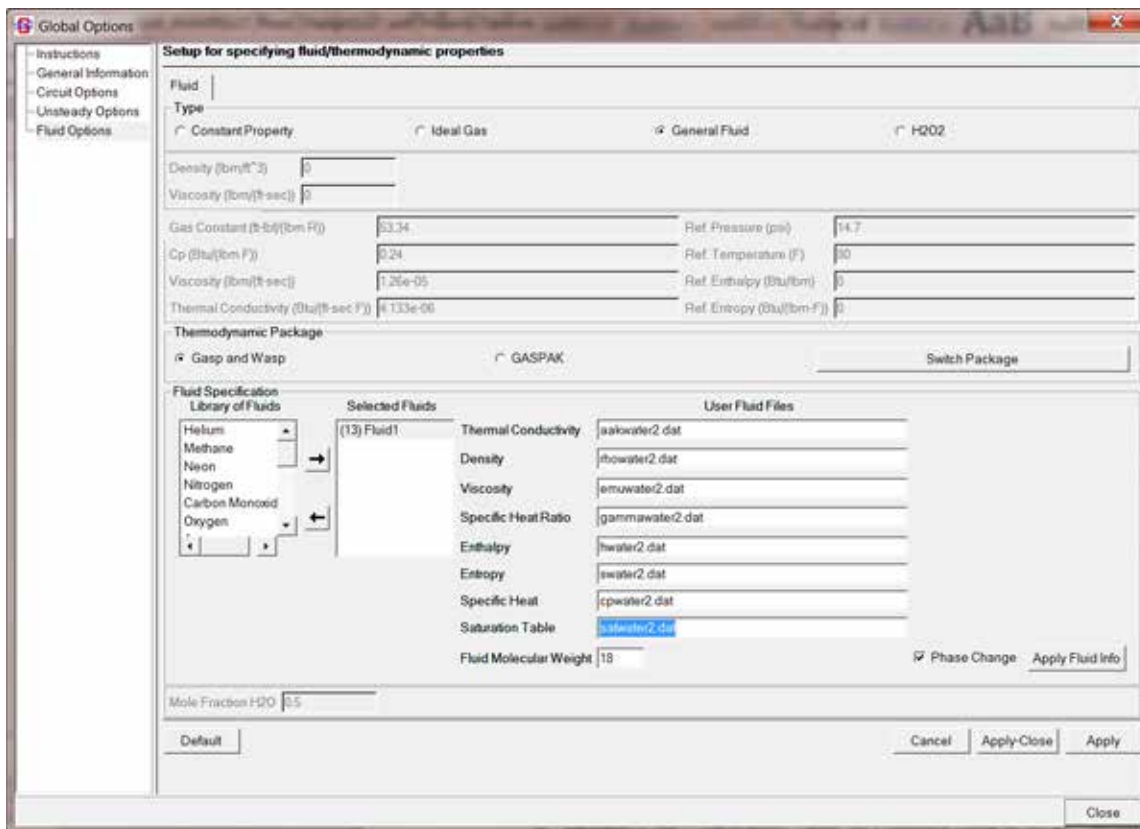
Figure 55. Defining a user fluid in the VTASC Fluid Options dialog.
