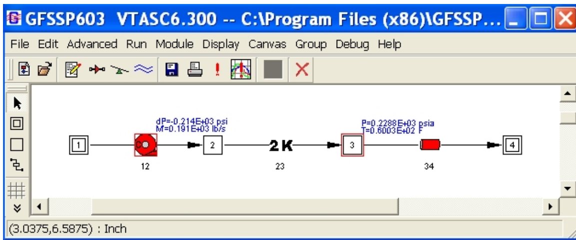
Figure 95. Display results in flow circuit example.
