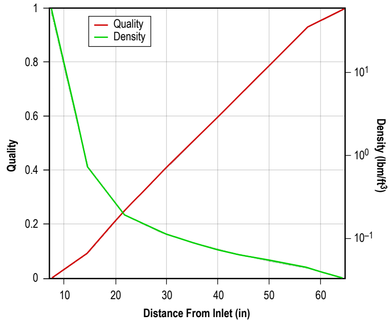
Figure 236. Distribution of quality and density in the vertical tube.
