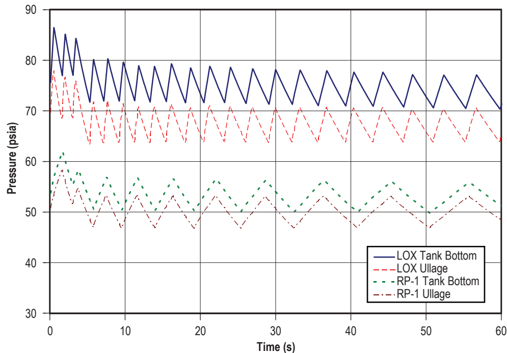
Figure 151. Propellant tank pressure history.
