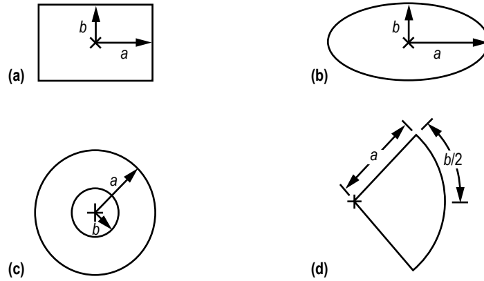
Figure 24. Noncircular duct cross section: (a) Rectangle, (b) ellipse, (c) concentric annulus, and (d) circular sector.
