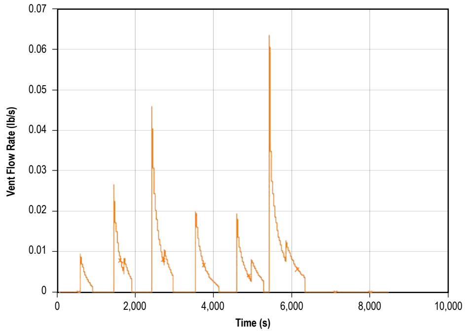
Figure 243. Predicted vent flow rate history during tank chilldown.
