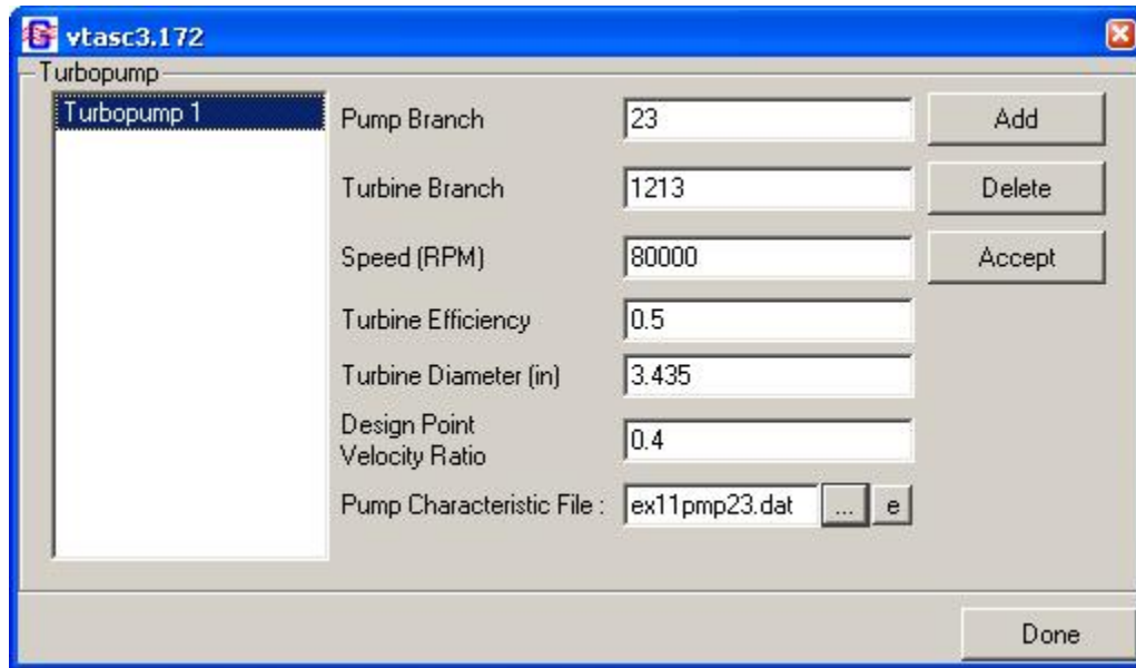
Figure 79. Turbopump option dialog.
