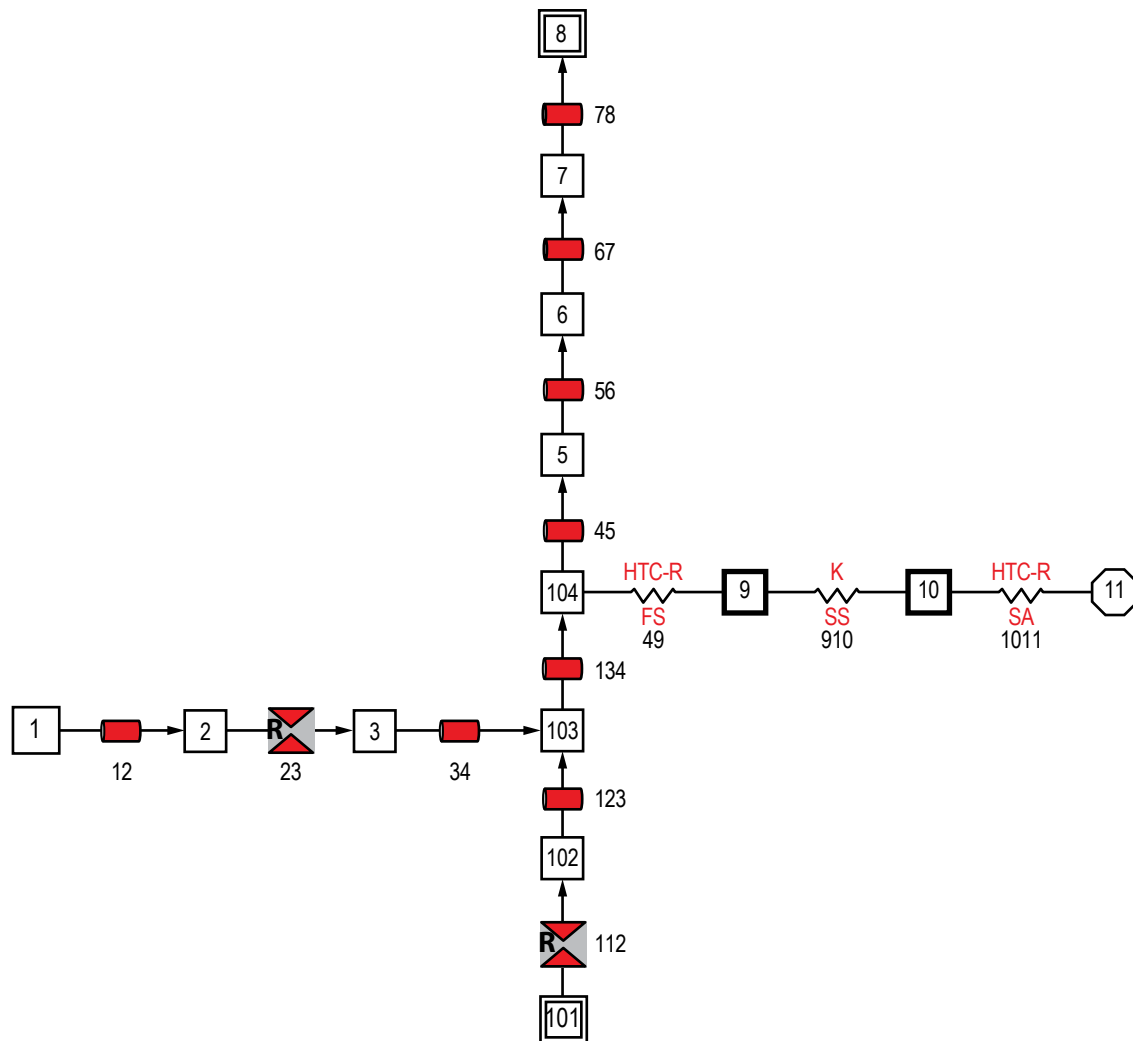
Figure 216. Combined VTASC model of LOX Recirculation Line model imported into Helium Injector model.
