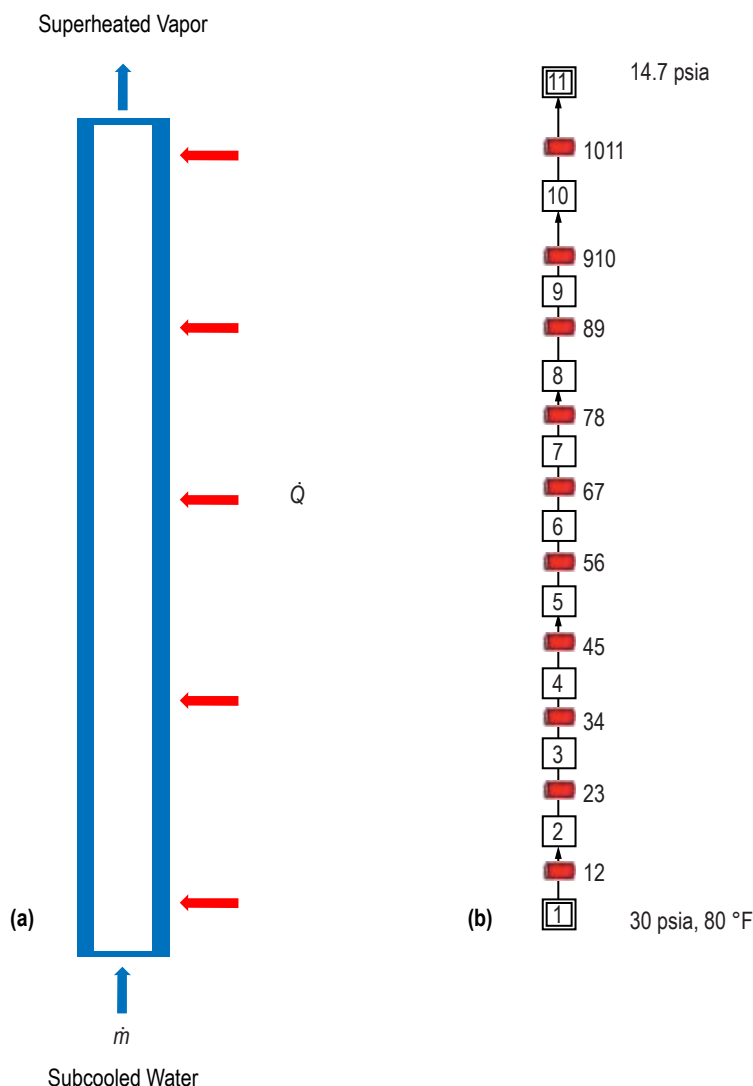
Figure 233. Boiling water reactor: (a) Problem schematic and (b) GFSSP model.
