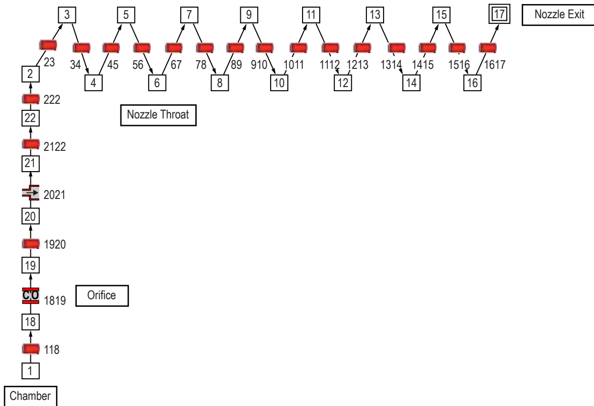
Figure 253. GFSSP model of solid propellant rocket motor.
