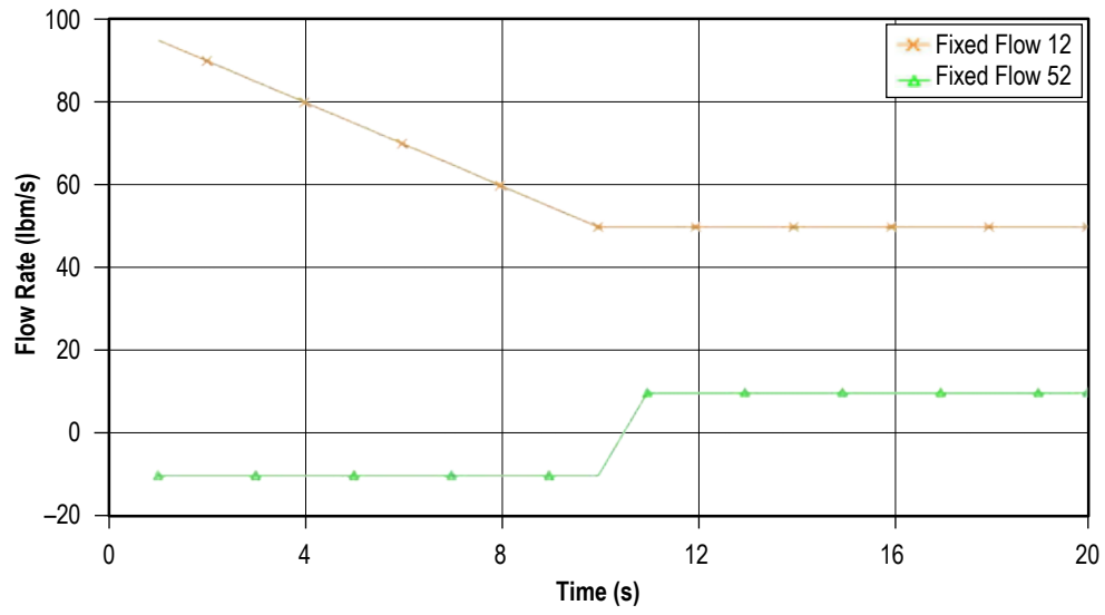
Figure 212. Flow rates in fixed flow branches.
