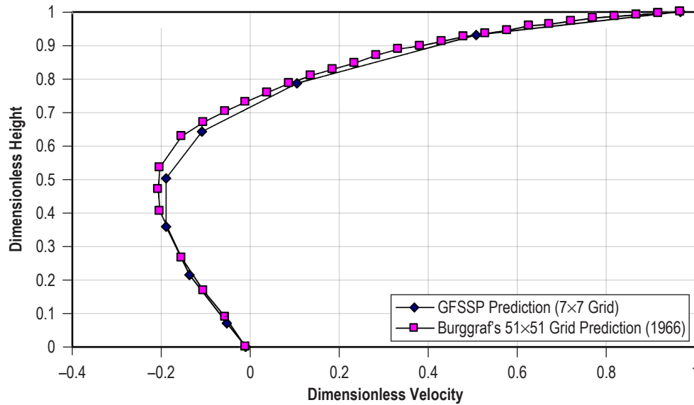
Figure 226. Shear driven square cavity centerline velocity distribution.
