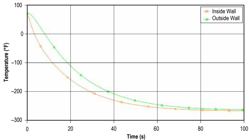
Figure 219. Inside and outside temperature of pipe wall.
