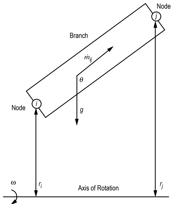
Figure 21. Schematic of a branch showing gravity and rotation.
