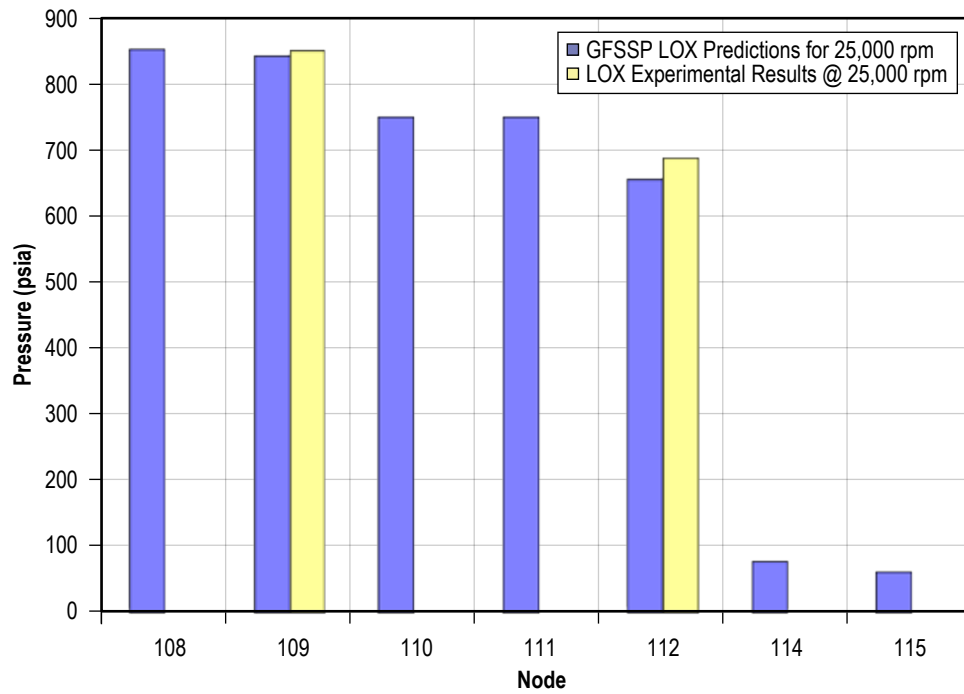
Figure 209. Simplex pressure predictions compared to experimental data.
