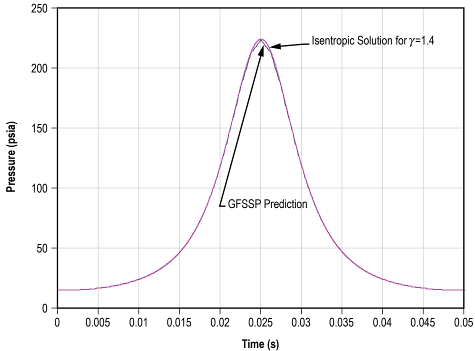
Figure 132. Predicted pressure history of piston-cylinder model.
