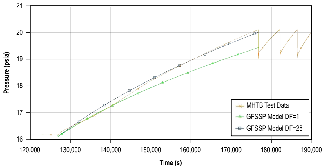
Figure 251. Application results for MHTB self-pressurization model.
