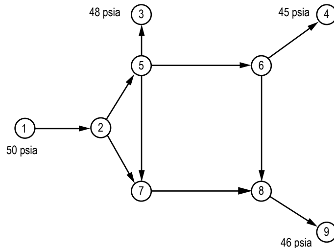
Figure 103. Water distribution network schematic (example 2).
