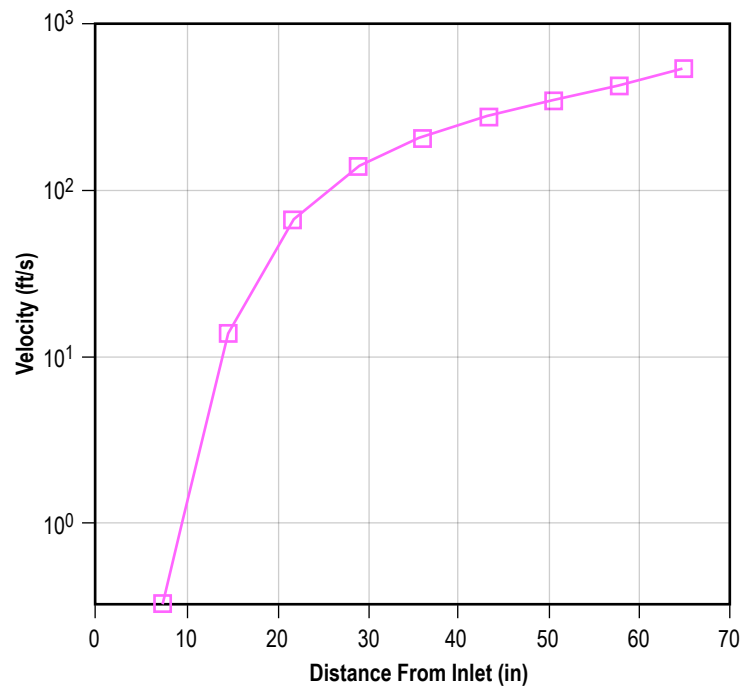
Figure 237. Distribution of velocity in the vertical tube.
