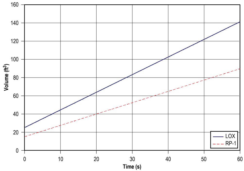
Figure 158. Ullage volume history in propellant tanks.
