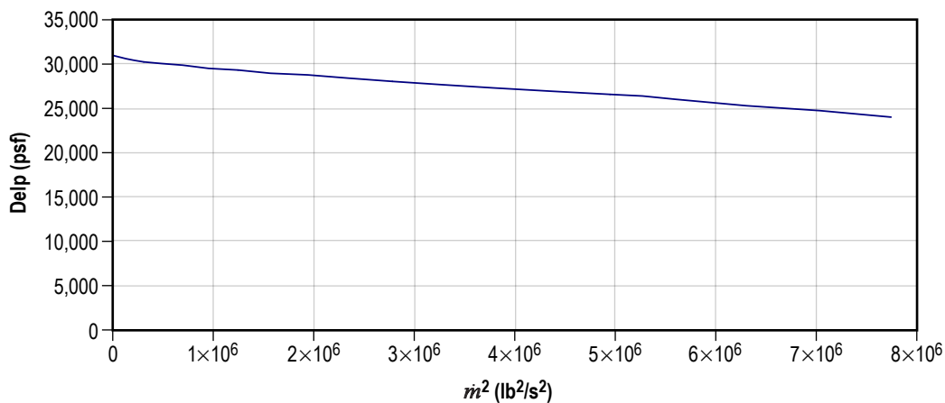
Figure 101. Pump characteristics curve in GFSSP format.
