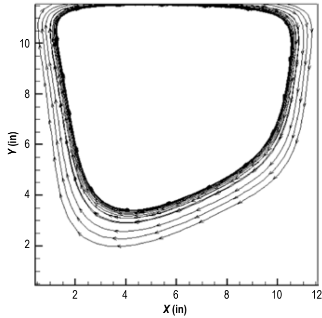
Figure 228. Predicted stream traces in the driven cavity.
