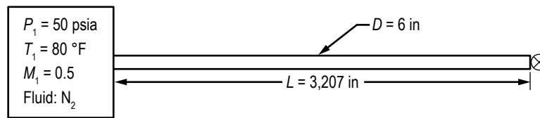
Figure 189. Fanno flow schematic (example 18).
