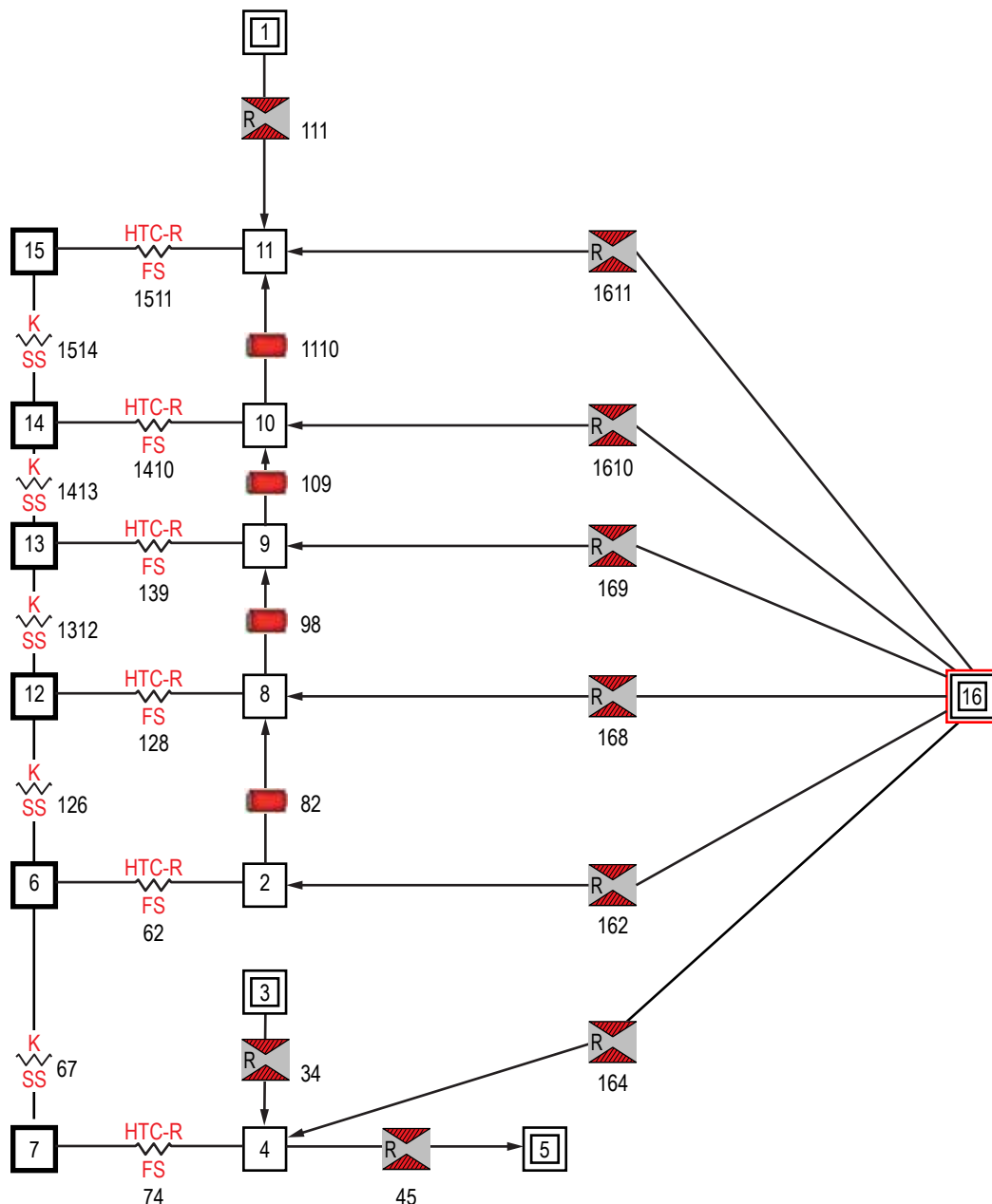
Figure 247. GFSSP model of MHTB test tank.
