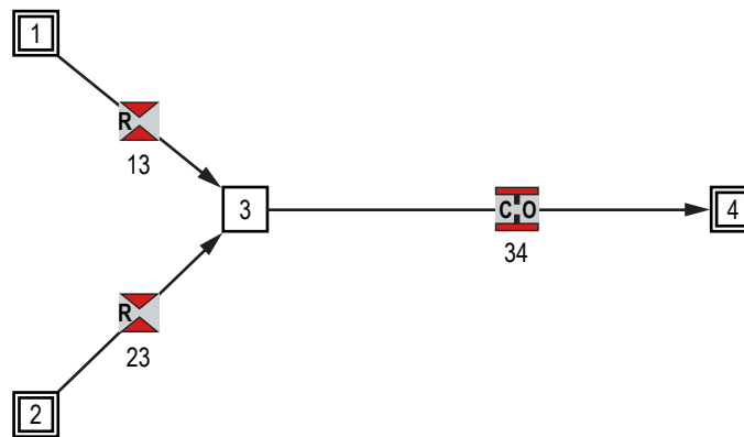
Figure 112. GFSSP model of mixing problem.
