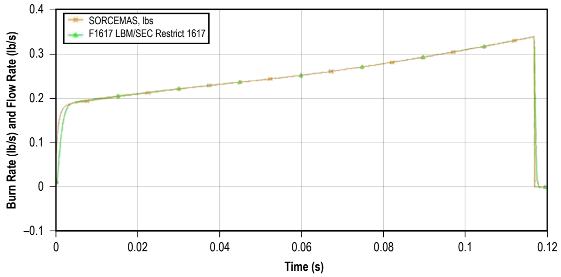
Figure 255. History of burning rate and flow rate at nozzle exit.
