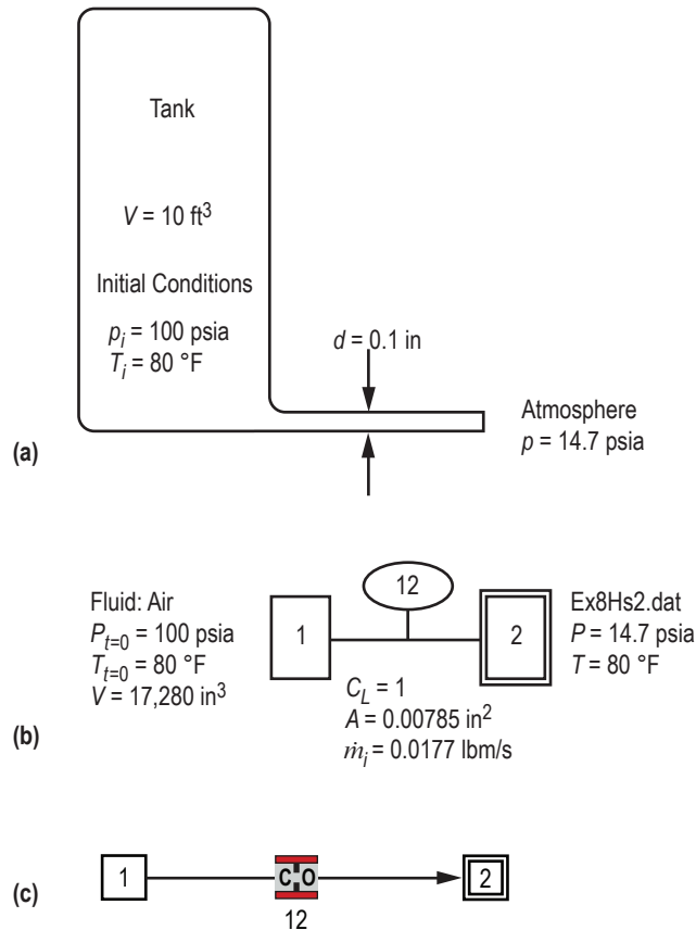
Figure 126. Venting air tank schematics: (a) Physical schematic, (b) detailed model schematic, and (c) VTASC model.
