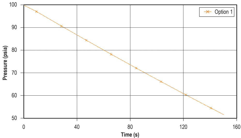
Figure 177. Tank pressure history (example 16).
