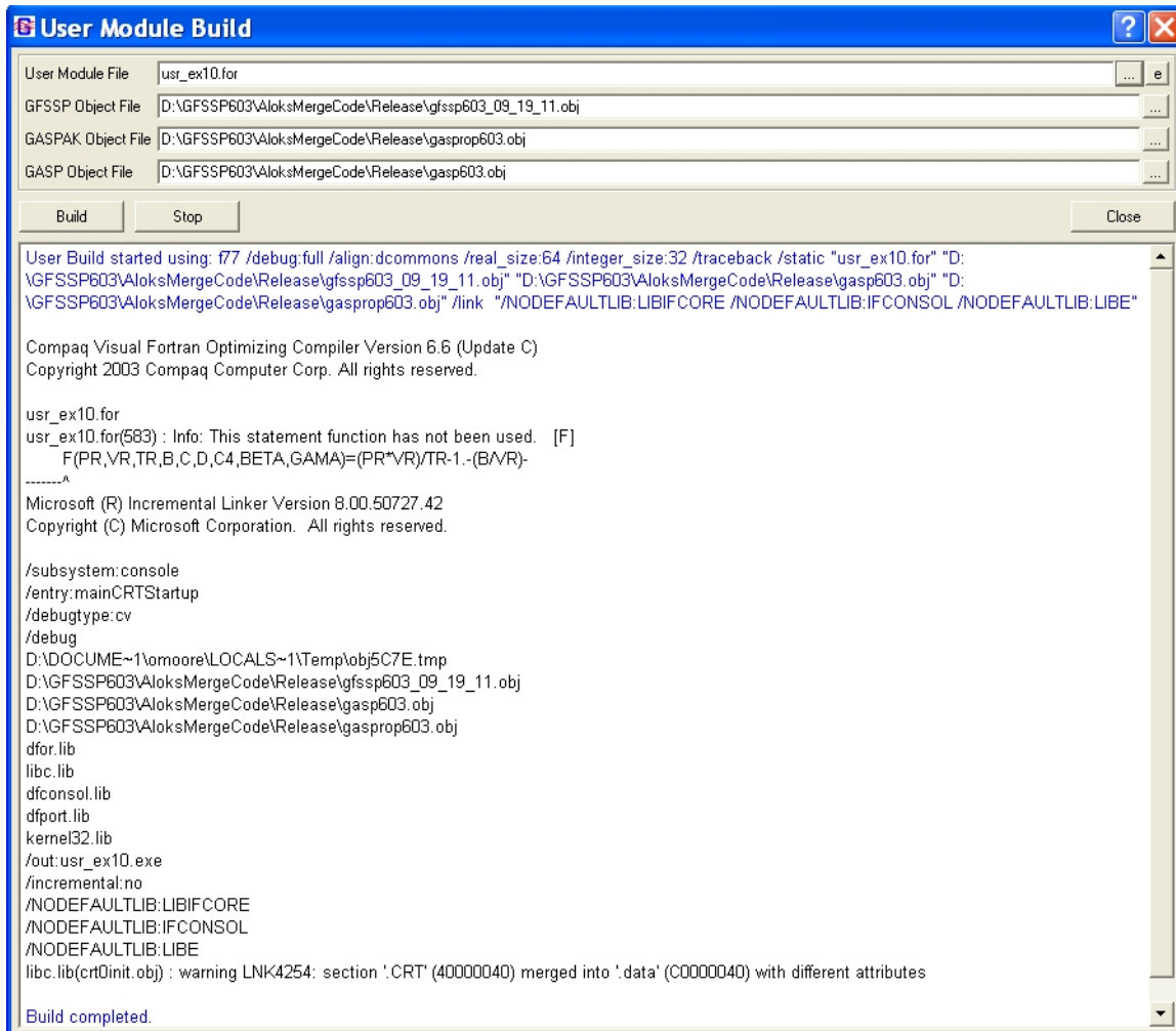
Figure 89. User Executable Build dialog.
