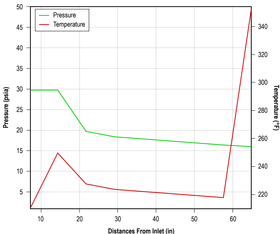
Figure 235. Pressure and temperature distribution in the vertical tube.
