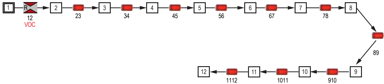
Figure 230. GFSSP model of sudden valve opening experiment of Lee and Martin. 52
