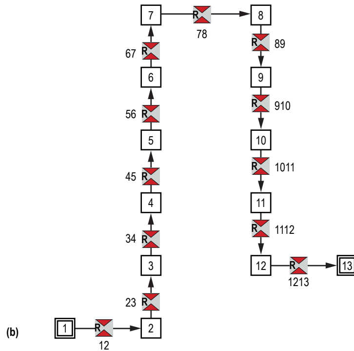
Figure 118. GFSSP model of the rotating radial disk: (a) Detailed schematic and (b) VTASC model.
