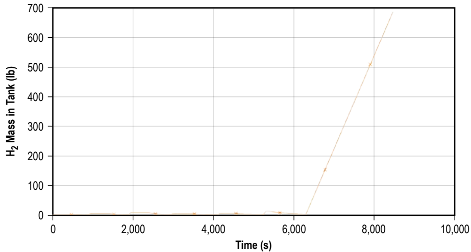
Figure 242. Predicted hydrogen mass history in the tank.
