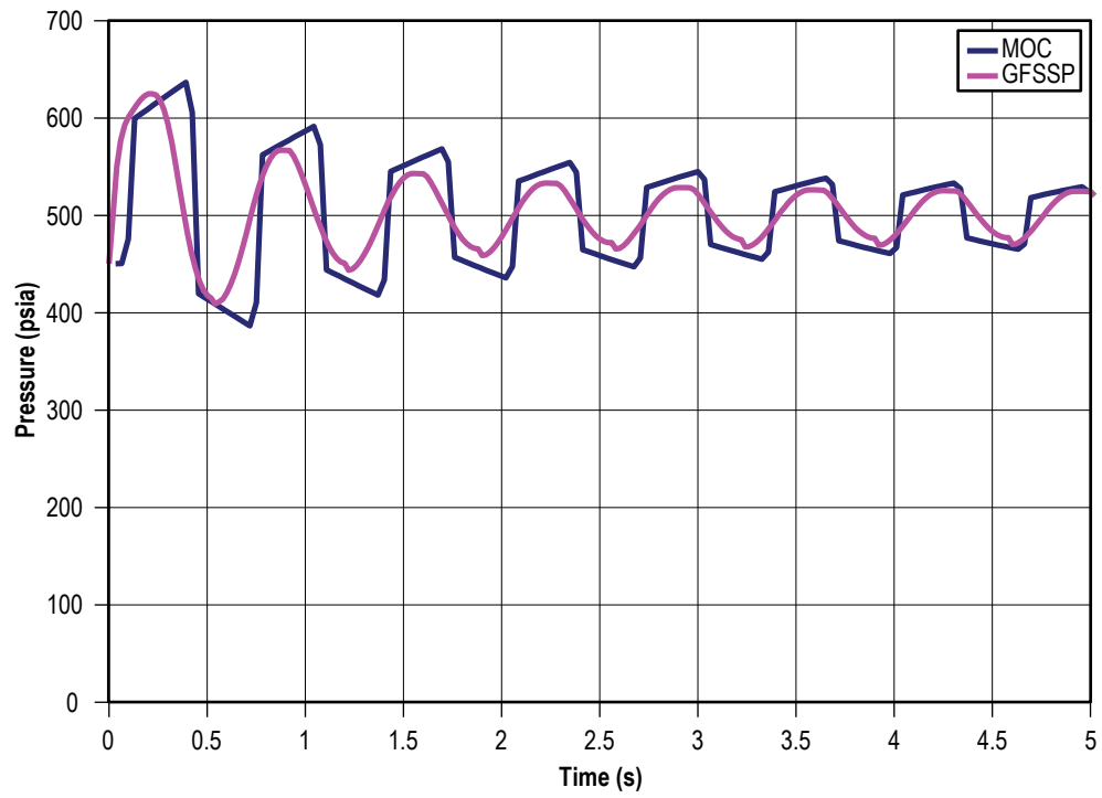
Figure 173. Comparison of GFSSP and MOC predicted pressure oscillations.
