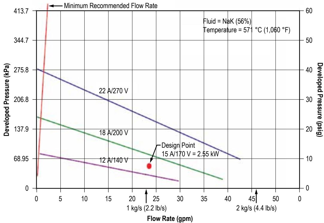
Figure 202. Style-IV ac conduction pump performance curve (reproduced from MSA Research Corp. dwg. No. C-510356).
