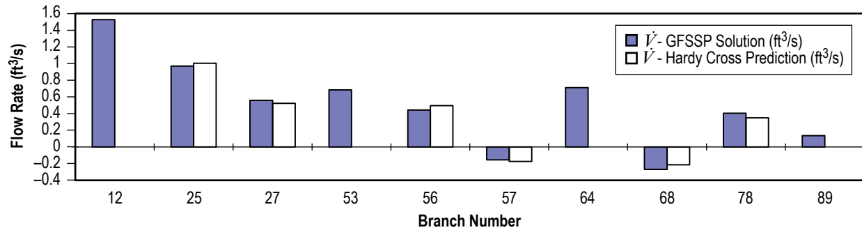
Figure 105. Flow rate comparison between GFSSP and Hardy Cross method predictions.
