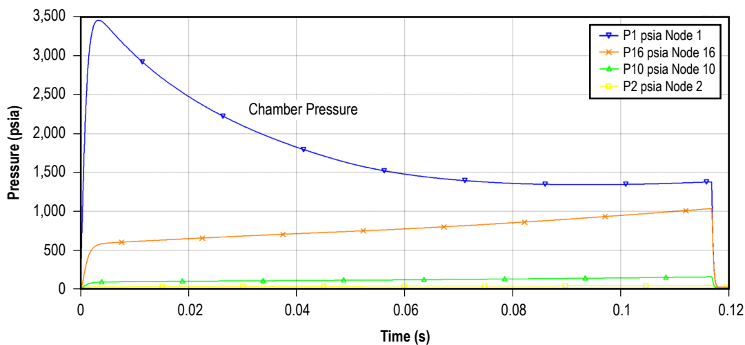
Figure 254. Pressure history during the propellant burn and tail-off.
