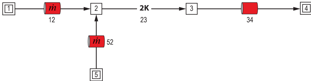
Figure 211. VTASC model of a fluid network with fixed flow rate option.
