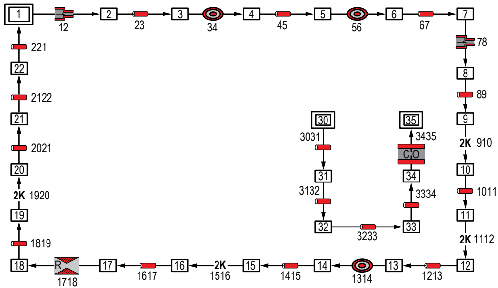
Figure 203. VTASC model of lithium loop with Heat Exchanger (example 20).
