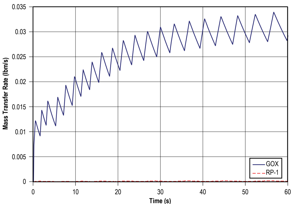
Figure 156. Mass transfer history of propellant.
