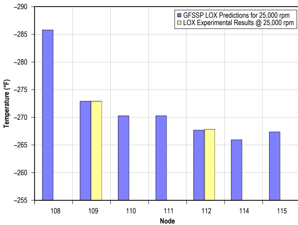
Figure 210. Simplex temperature predictions compared to experimental data.
