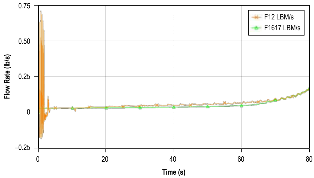
Figure 166. Predicted flow rate (lb/s) at the pipe entrance and middle.
