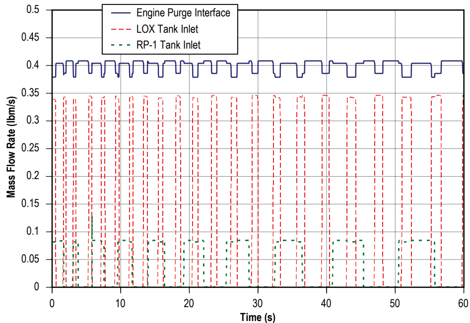
Figure 138. Helium mass flow rate history.
