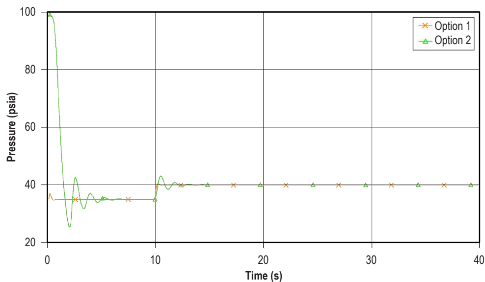
Figure 178. Pressure history downstream of pressure regulator (example 16).
