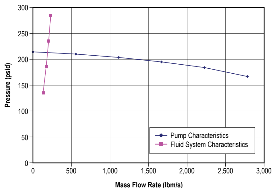
Figure 102. Fluid system operating point.
