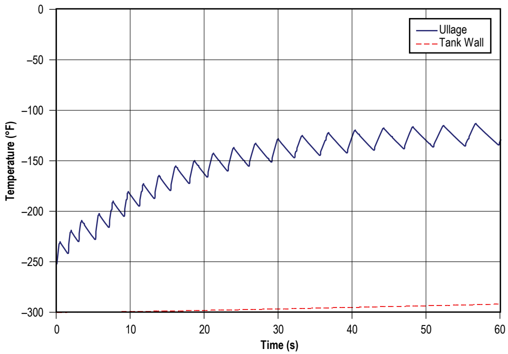
Figure 154. LOX temperature history.
