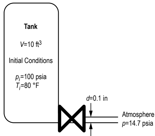
Figure 174. Tank blowdown with pressure regulator VTASC model (example 16).
