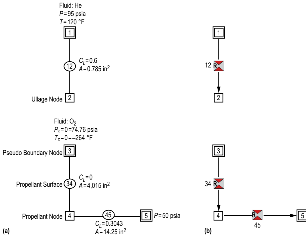
Figure 134. Simple pressurization system test model: (a) Detailed model schematic and (b) VTASC model.
