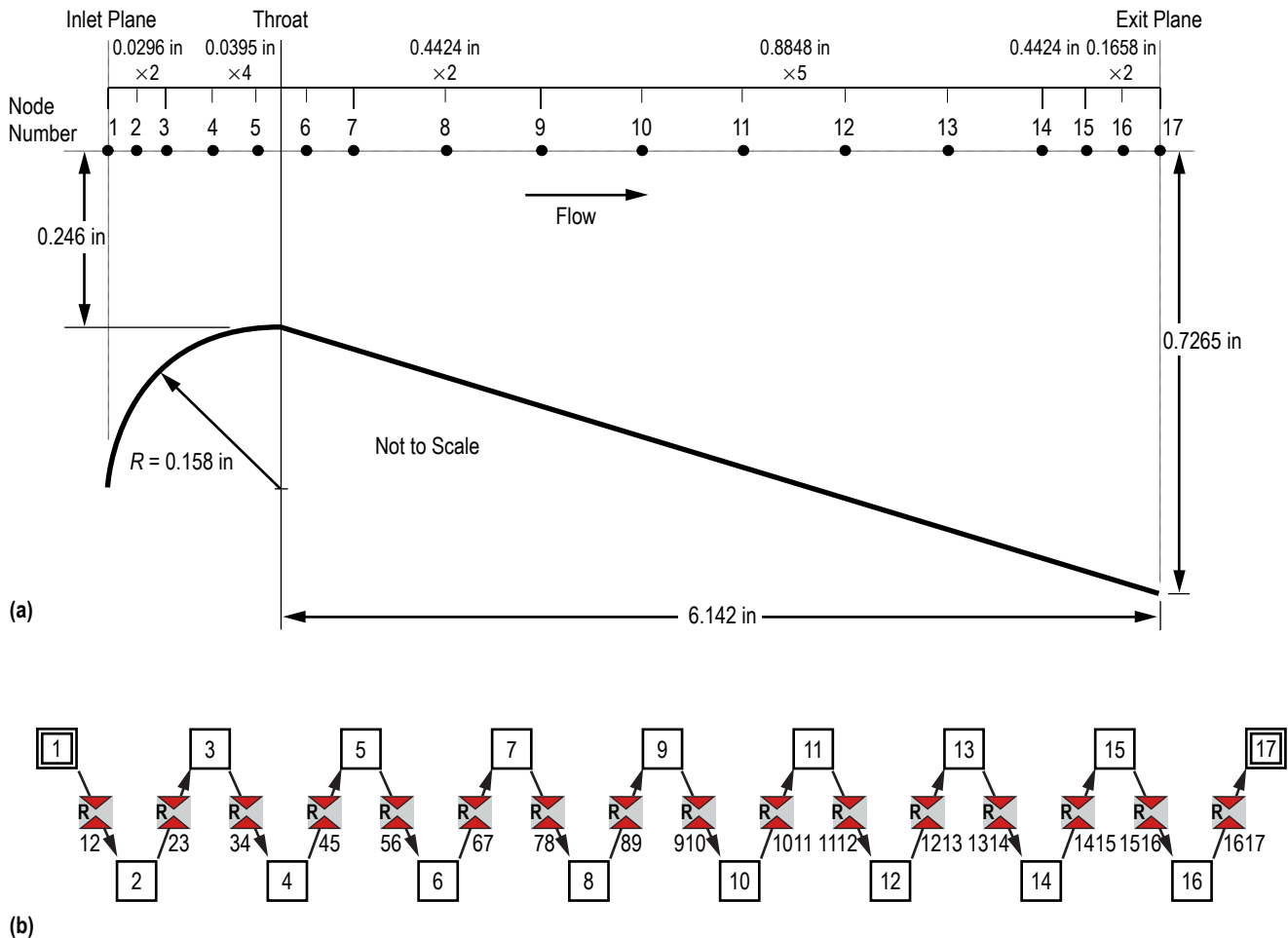
Figure 107. Converging-diverging steam nozzle model: (a) Detailed schematic and (b) VTASC model.
