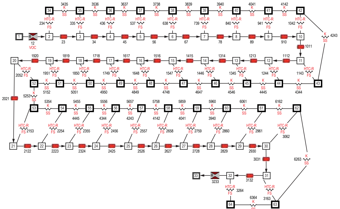
Figure 164. GFSSP model of the cryogenic pipe line.
