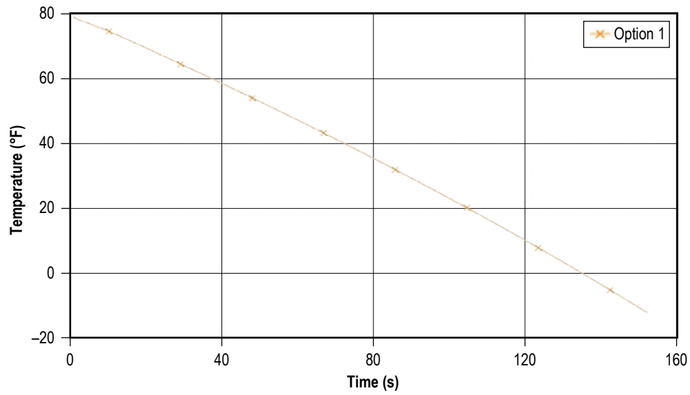
Figure 179. Tank temperature history (example 16).
