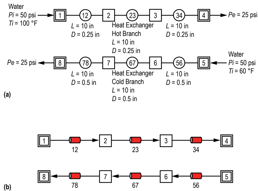
Figure 114. GFSSP model of the heat exchanger: (a) Detailed schematic and (b) VTASC model.
