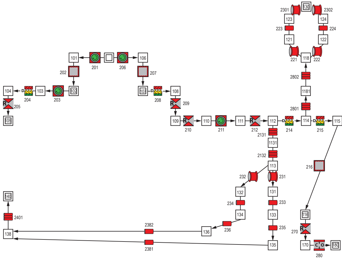
Figure 208. Simplex turbopump VTASC model.
