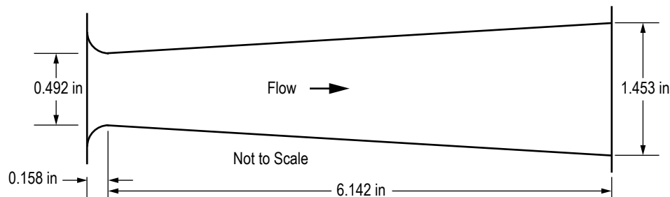
Figure 106. Converging-diverging steam nozzle schematic.
