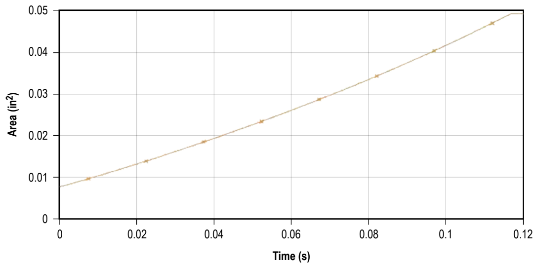
Figure 256. History of area change during propellant burn.
