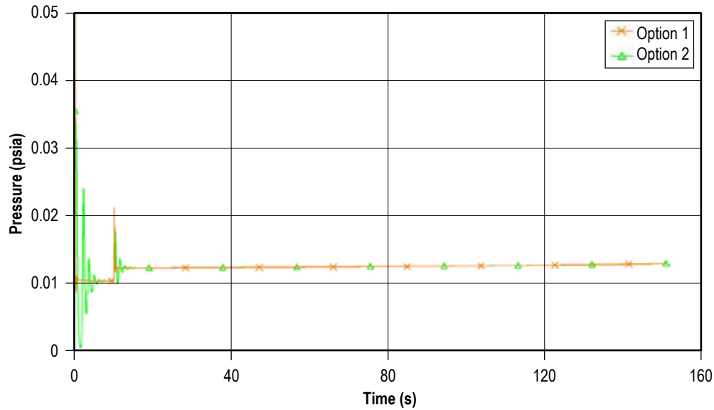
Figure 181. Pressure regulator flow rate history (example 16, restrict 12).
