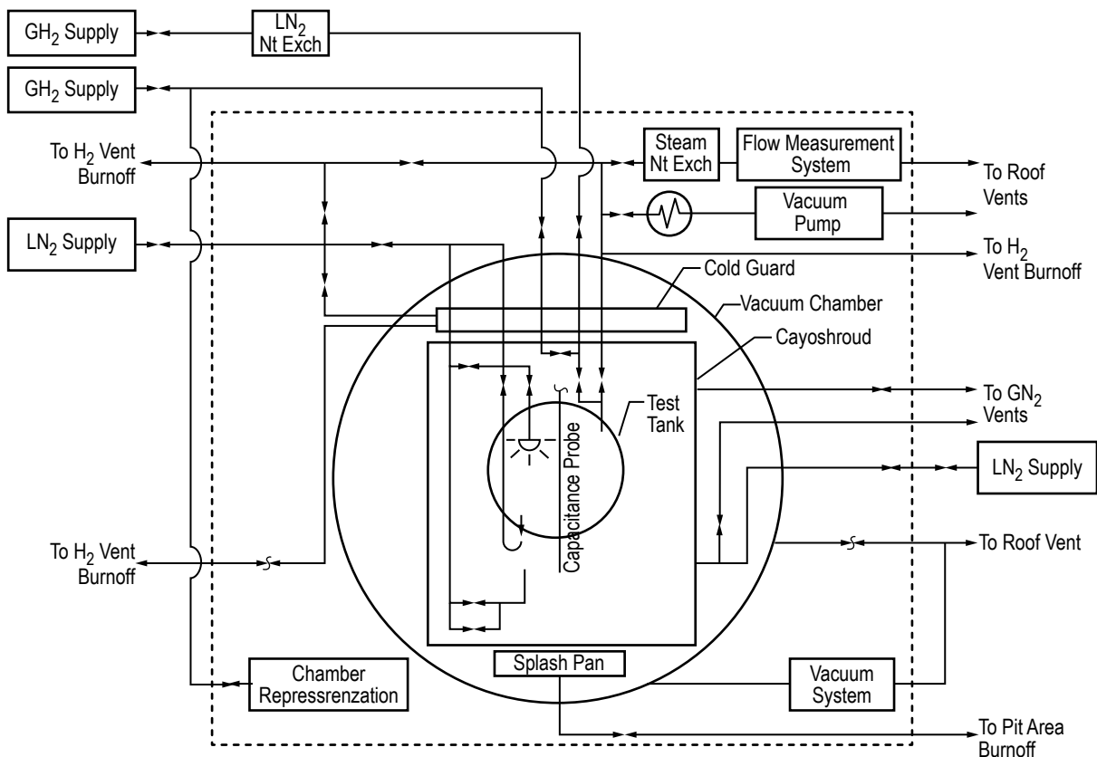
Figure 238. K-site test set-up for no-vent fill experiment.
