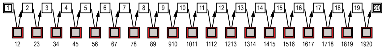
Figure 123. GFSSP model of squeeze film damper.
