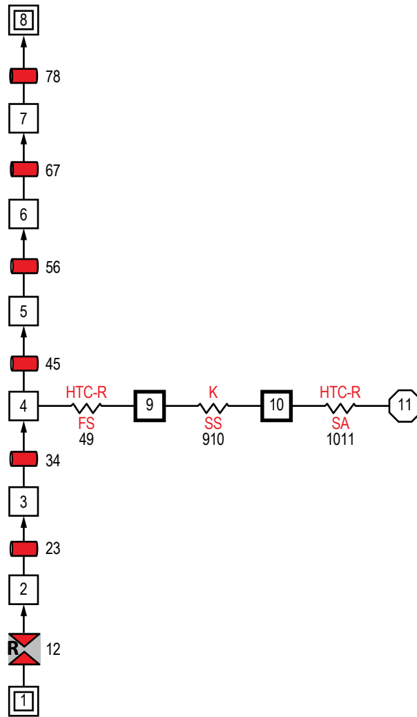
Figure 214. VTASC model of LOX recirculation line with heat transfer.
