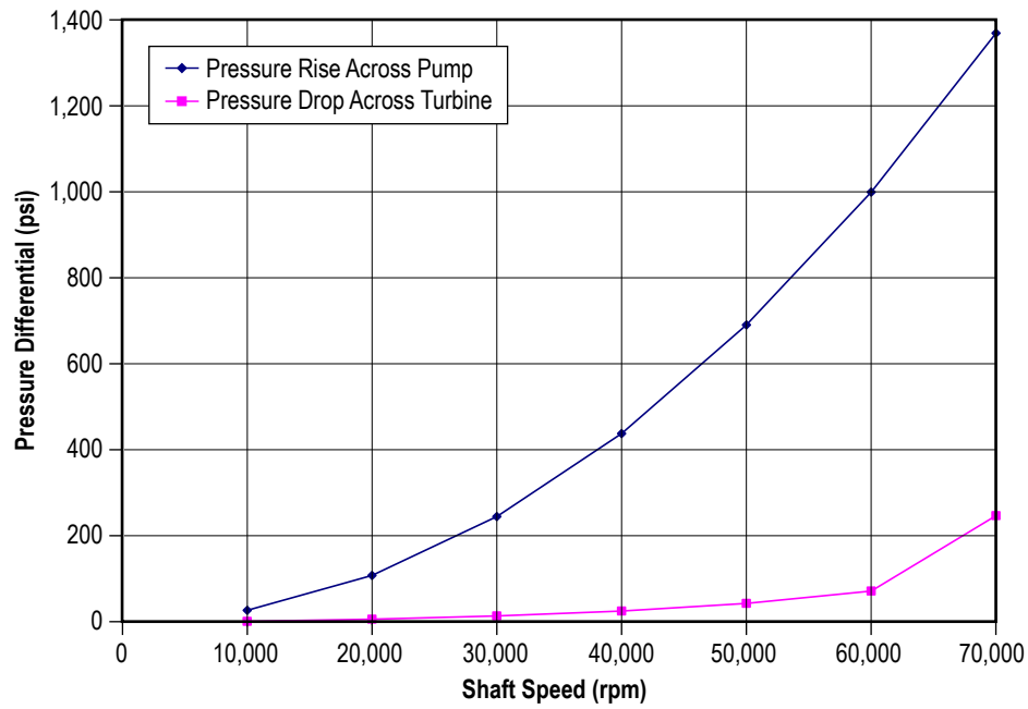
Figure 146. Parametric study results: turbopump pressure differential.
