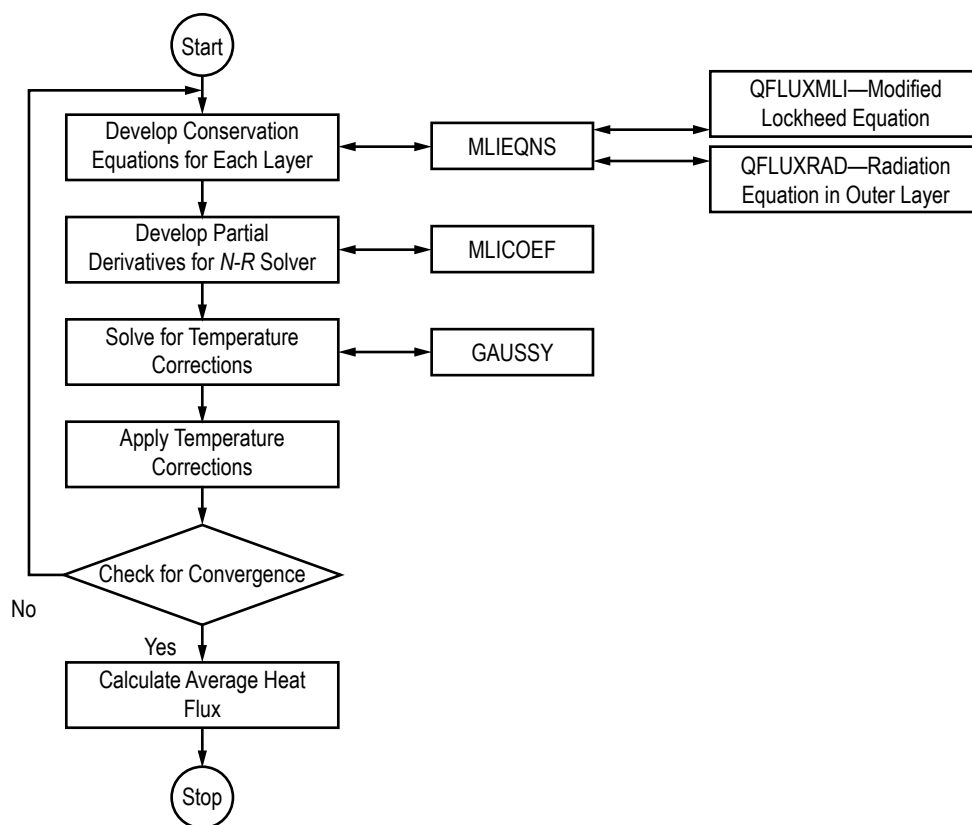
Figure 250. Flowchart of MLI_HEAT_RATE Subroutine.
