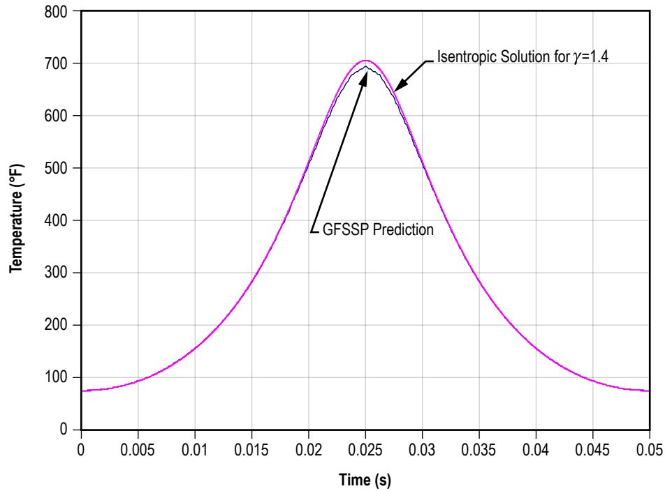
Figure 131. Predicted temperature history of piston-cylinder mode model.
