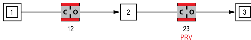
Figure 221. Example 24 relief valve VTASC model.
