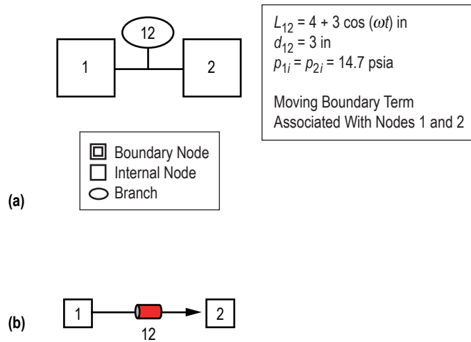
Figure 130. GFSSP model of the piston-cylinder: (a) Detailed model schematic and (b) VTASC model.
