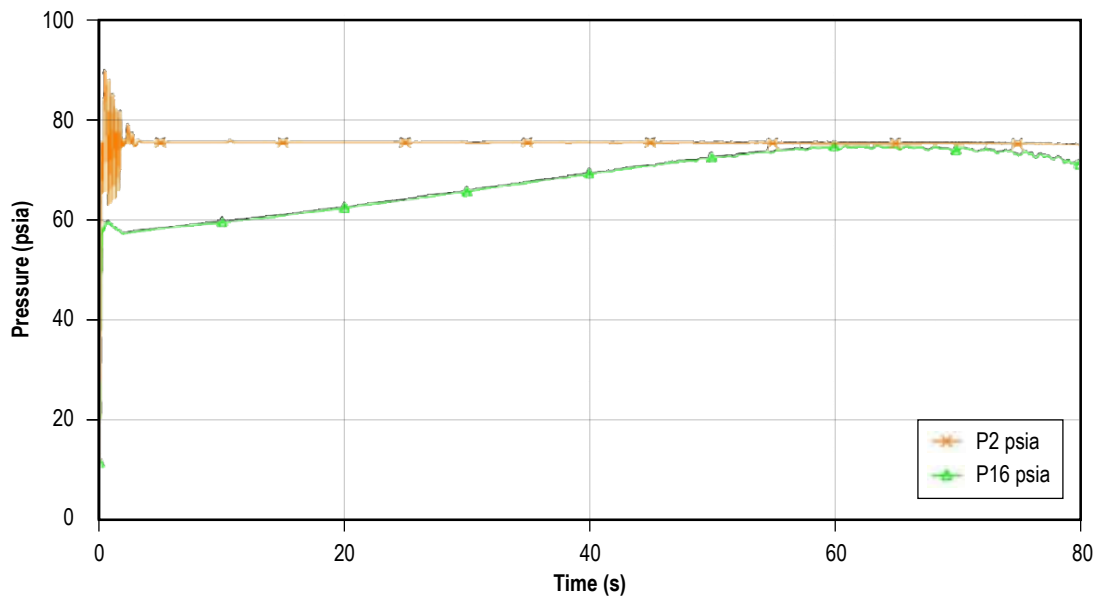
Figure 167. Predicted pressure (psia) near the pipe entrance and middle.
