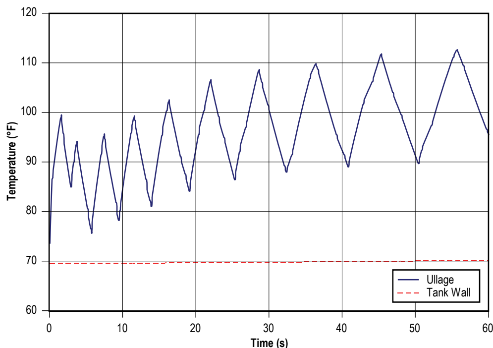
Figure 152. RP-1 temperature history.
