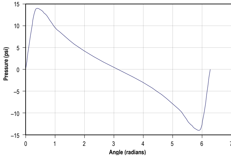
Figure 124. Predicted circumferential pressure distributions in the squeeze film damper.
