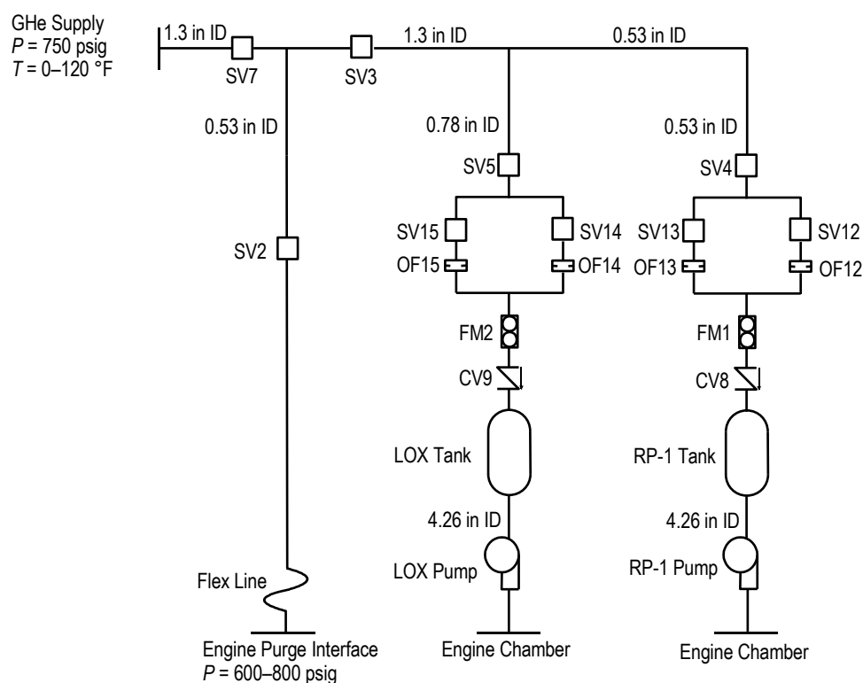
Figure 149. PTA1 helium pressurization system schematic.
