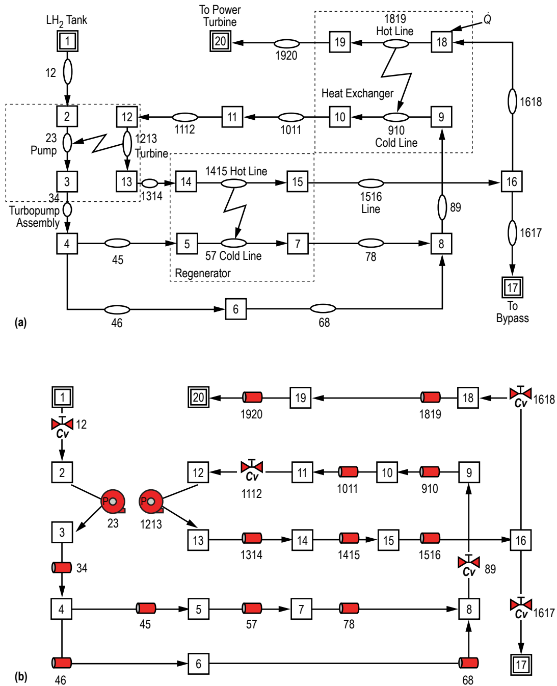
Figure 142. A flow circuit containing turbopump assembly: (a) Detailed model schematic and (b) VTASC model.
