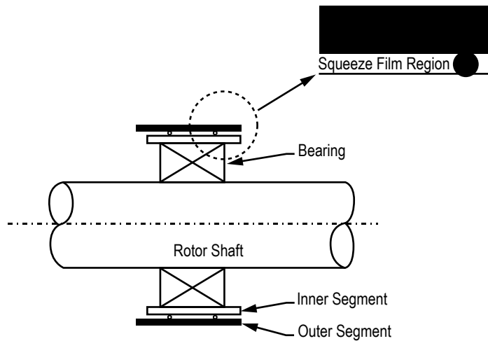
Figure 120. Squeeze film damper schematic (example 7, view 1).
