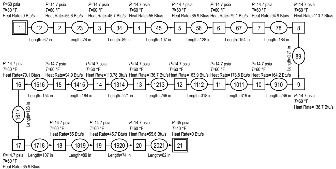
Figure 196. Pressurized tank detailed model schematic (example 19)—fluid: nitrogen.
