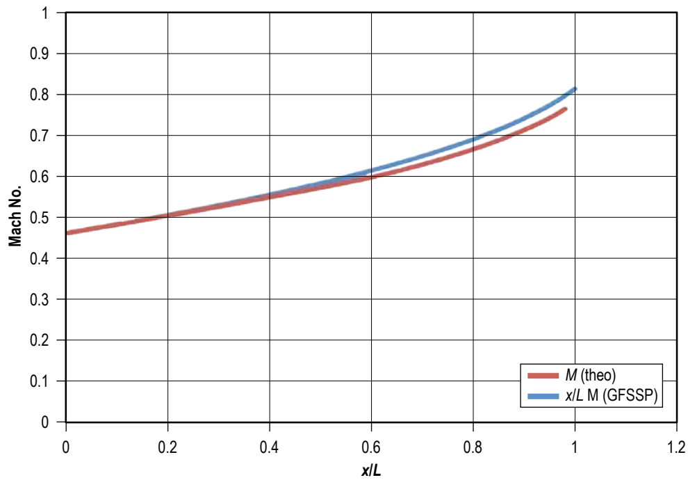
Figure 199. Mach No. distribution for Rayleigh flow ( Q = 1,800 Btu/s).
