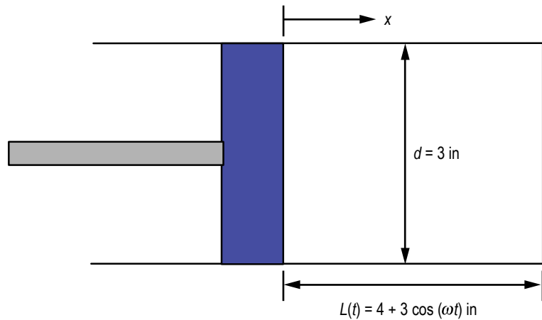
Figure 128. Piston-cylinder configuration.
