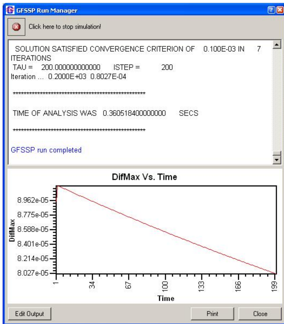
Figure 91. GFSSP Run Manager—unsteady simulation.
