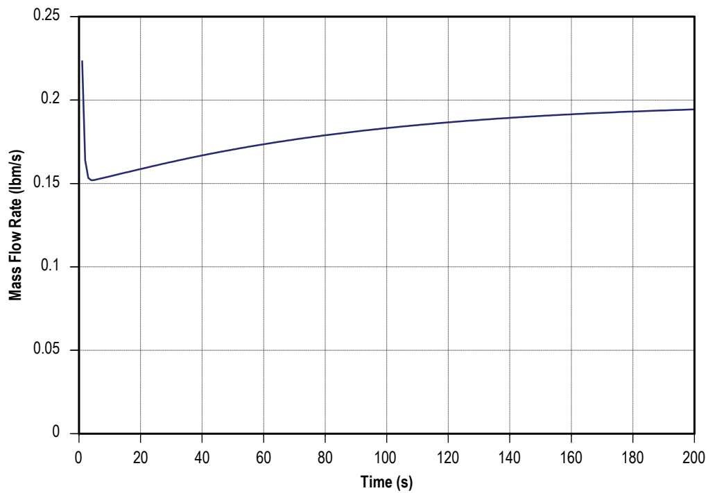
Figure 147. Parametric study results: turbopump hydrogen mass flow rate.
