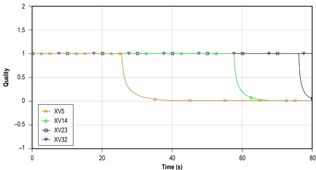
Figure 168. Predicted quality (vapor mass fraction) at the four measurement stations.
