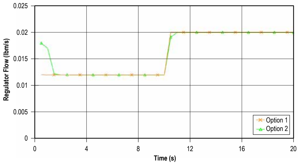
Figure 188. Flow regulator flow rate history (example 17).
