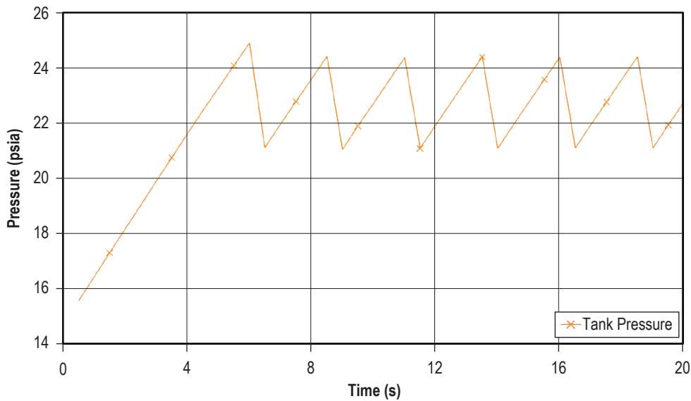
Figure 222. Pressure inside tank.
