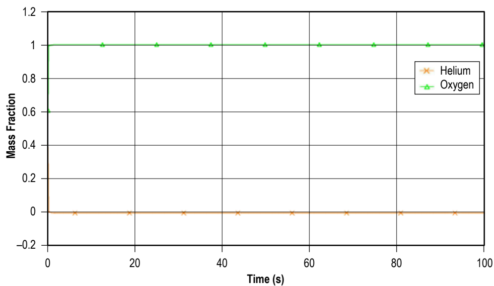
Figure 218. Mass fractions of He and O 2 at node 7.
