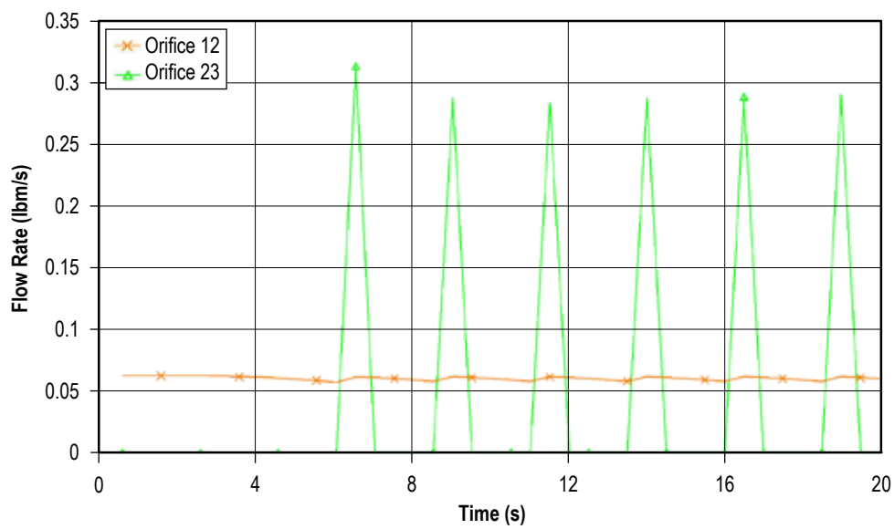
Figure 223. Flow in and out of tank.
