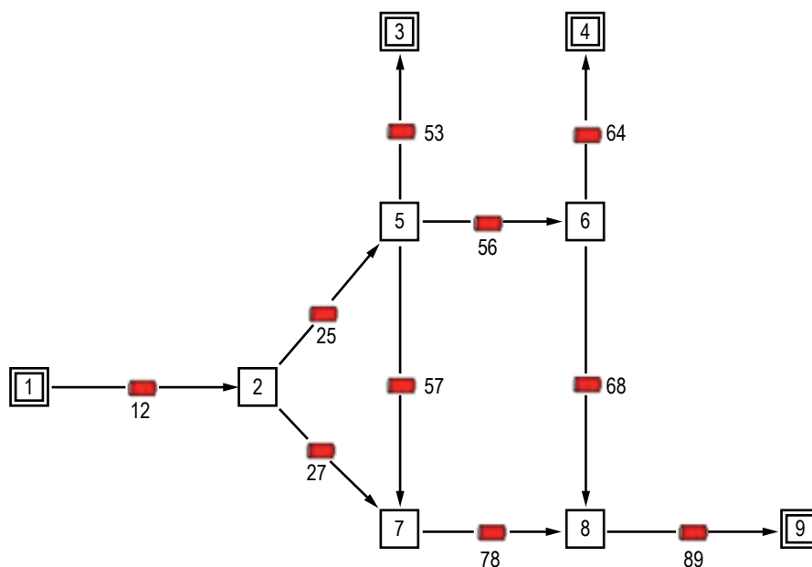
Figure 104. GFSSP model of the water distribution network.
