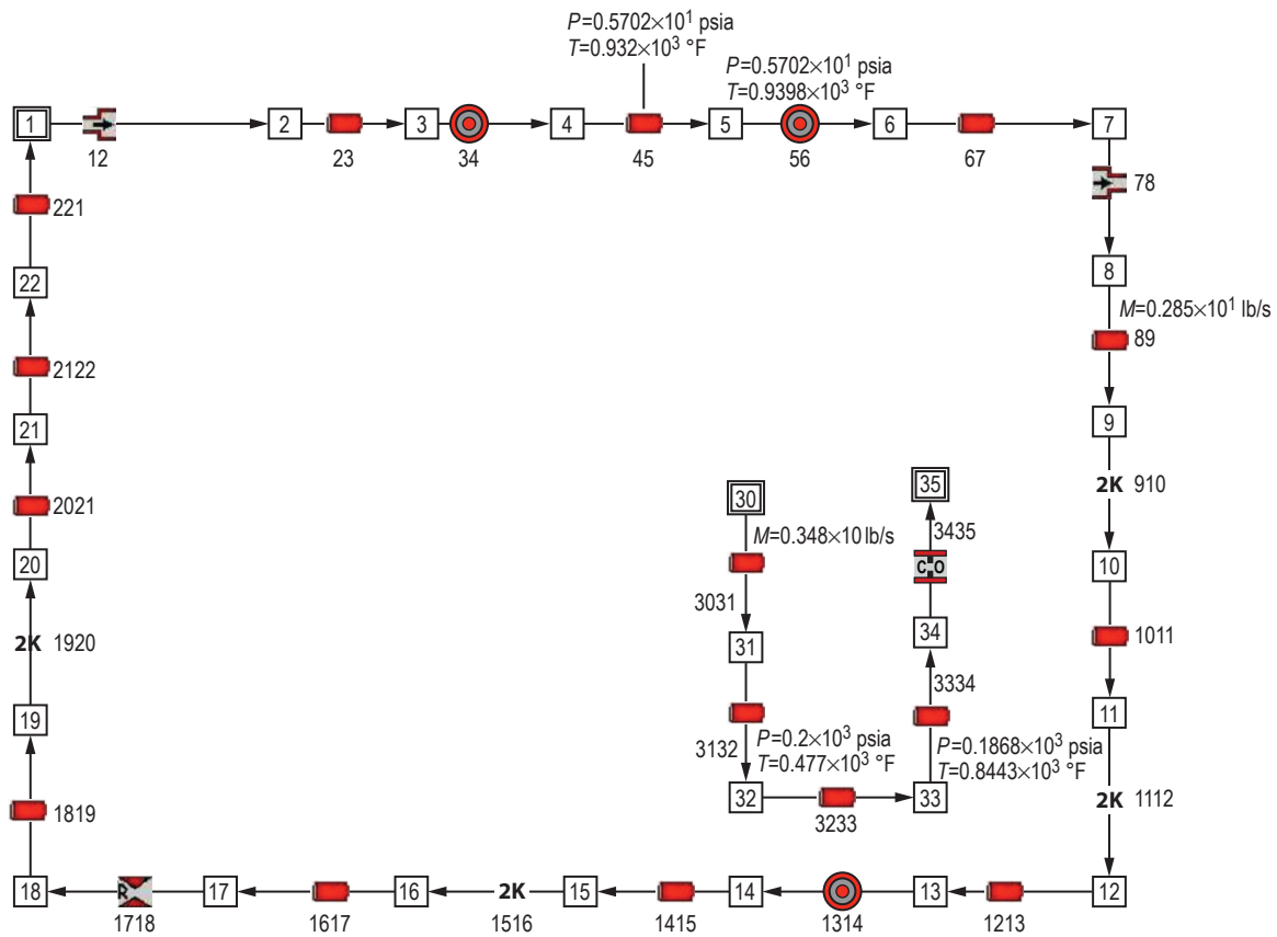
Figure 205. Sample results of example 20 is displayed in the flow circuit.
