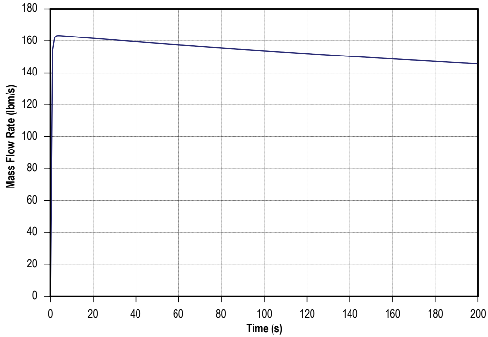
Figure 139. LOX mass flow rate history.
