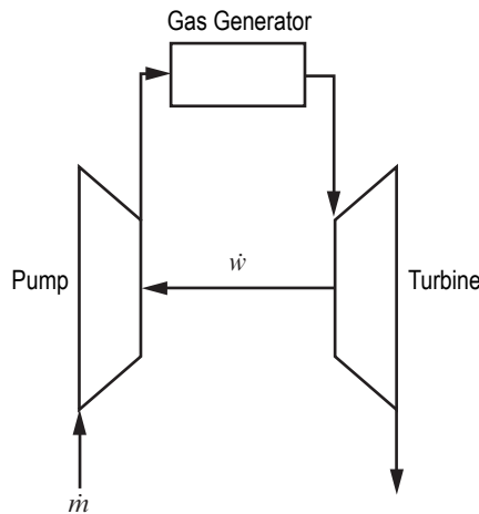
Figure 141. Simplified turbopump assembly.
