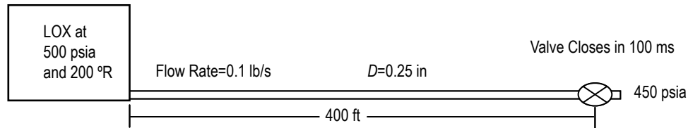
Figure 170. Schematic of a propellant tank, pipe line, and valve.
