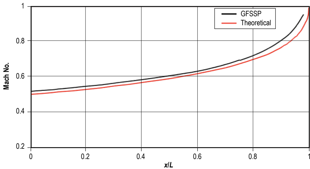
Figure 194. Fanno flow plot of Mach number along the pipe length.
