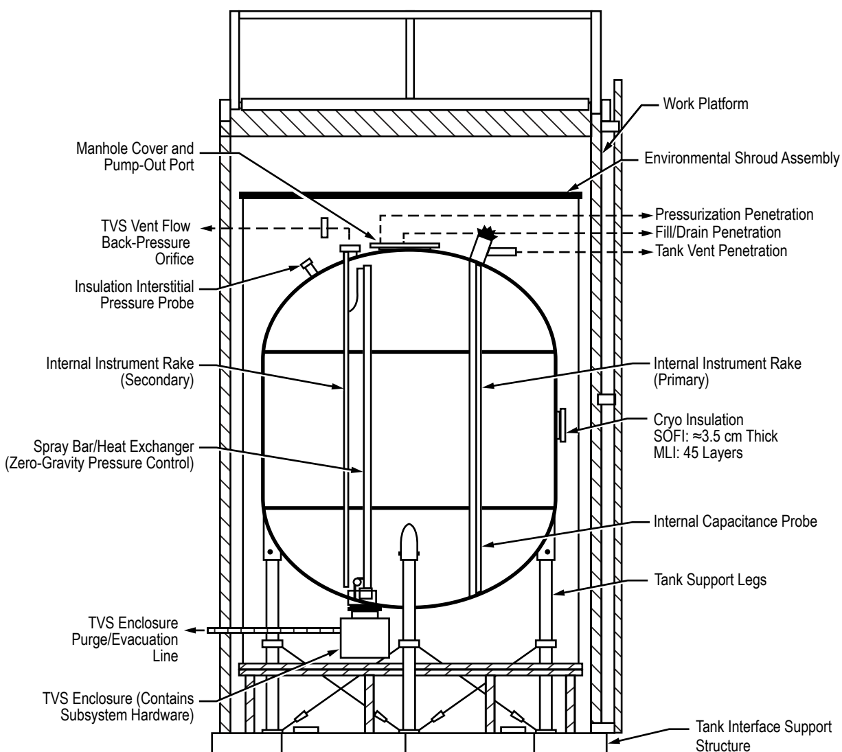
Figure 246. MHTB test tank and supporting hardware schematic.
