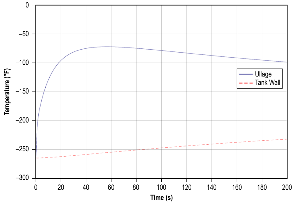
Figure 137. Ullage and tank wall temperature history.
