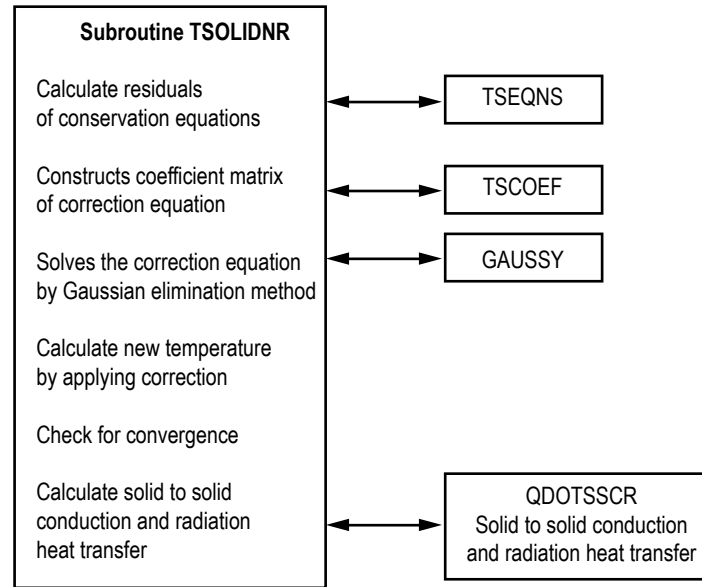
Figure 43. Solid temperature calculation by Newton-Raphson method.
