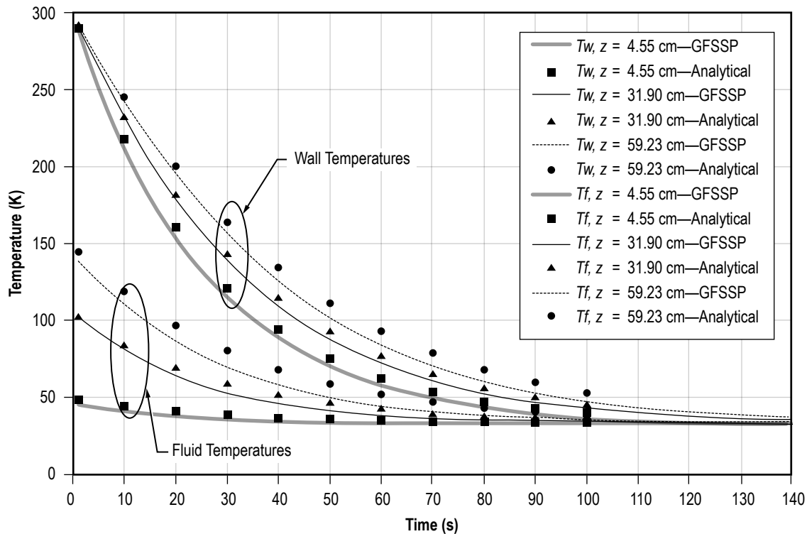
Figure 169. GFSSP's predicted wall and fluid temperatures compared to analytical solution by Cross et al. 33
