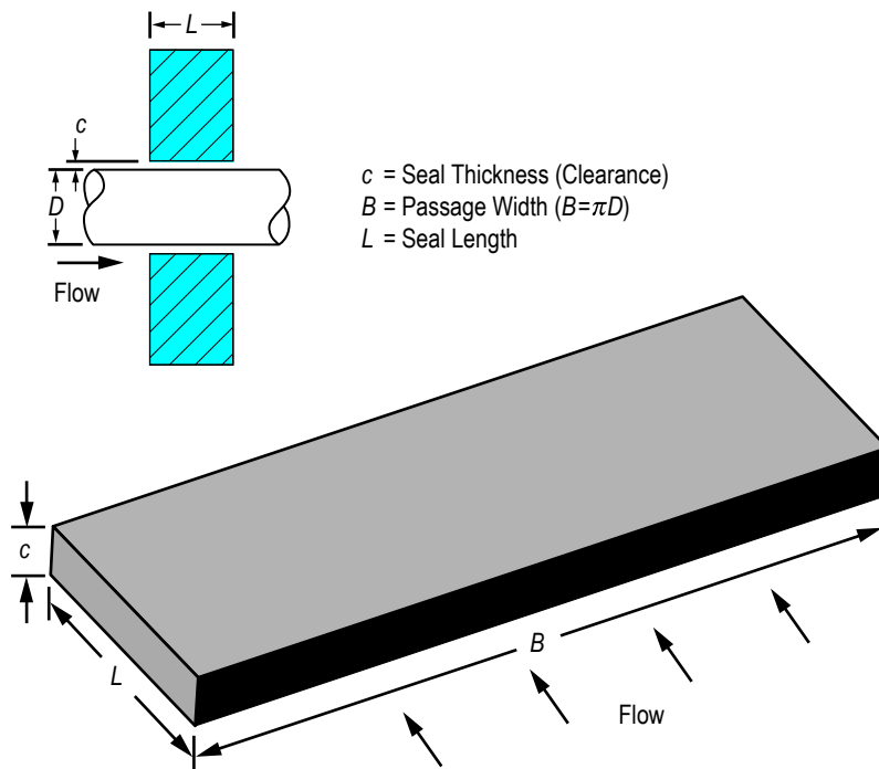
Figure 33. Parallel flat plate resistance option parameters.
