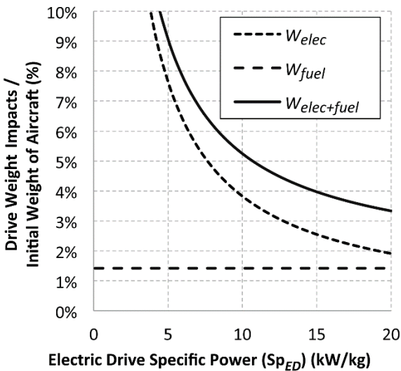
Figure 3.—Normalized weights of drive, fuel impact of inefficiency, and combined costs for 95 percent efficient drive.
