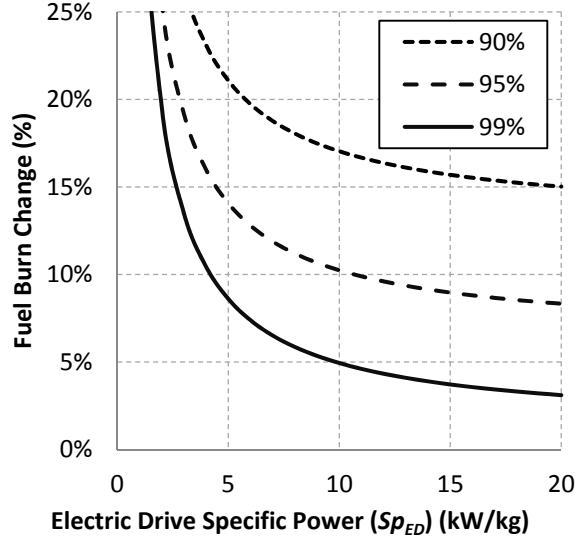
Figure 5.—Fuel burn change for select drive efficiencies.
