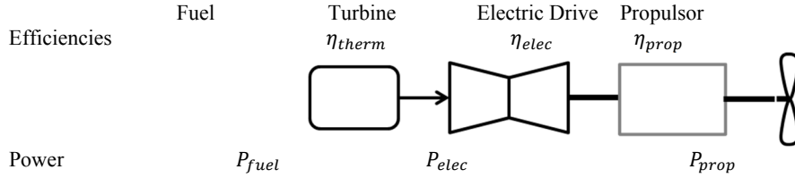
Figure 2.—Propulsion power and efficiency terms.
