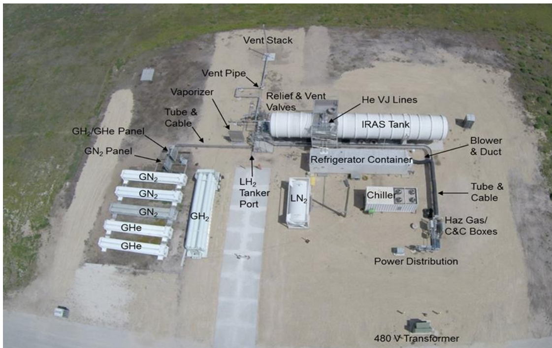
Figure 2: Aerial View of the GODU-LH2 Test Site
