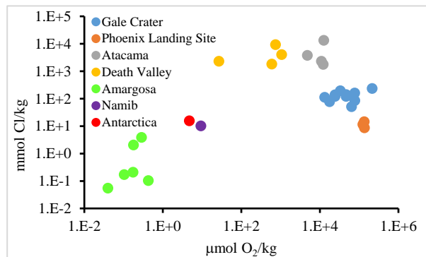
Fig. 1. Cl - versus O 2 content in terrestrial [3] and martian [1,4] soil and sediments.
