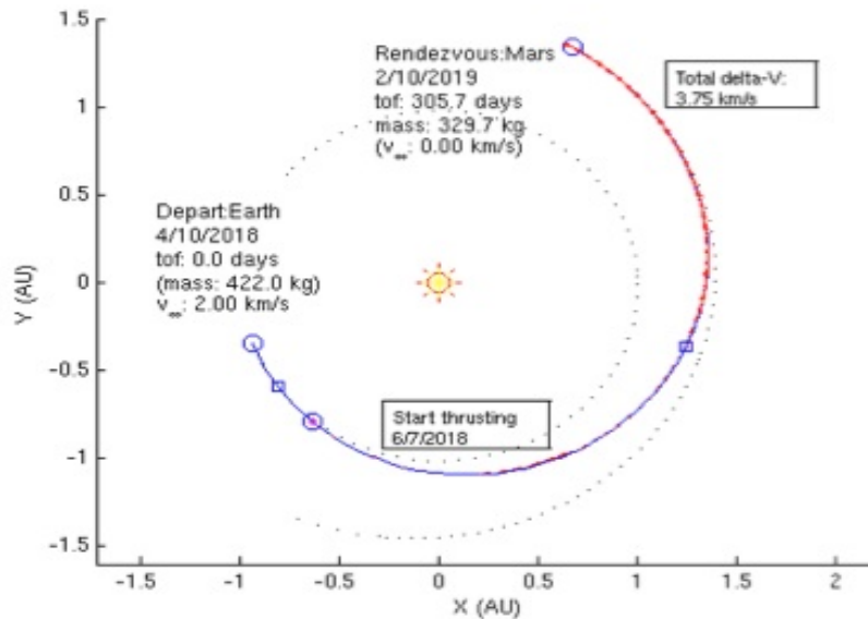
Figure 25: Trajectory from Earth departure to Mars rendezvous [39].
