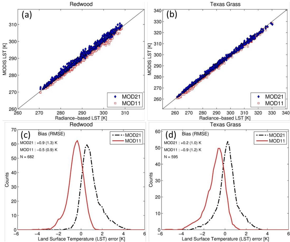
Figure 30. An example of the LST validation applied to the MODIS Aqua MOD11 and MOD21 LST products over Redwood and Texas Grassland sites (a, b) using three years of data collected (2003-2005). The bottom panels (c,d) show the histogram of the distribution of the LST error for MOD21 and MOD11 showing comparable performances.
