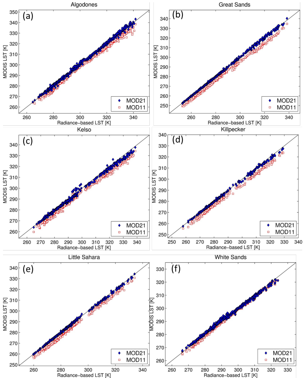
Figure 27. An example of the R-based validation method applied to the MODIS Aqua MOD11 and MOD21 LST products over six pseudo-invariant sand dune sites using all data during 2003-2005. AIRS profiles and lab-measured emissivities from samples collected at the sites were used for the R-based calculations.
