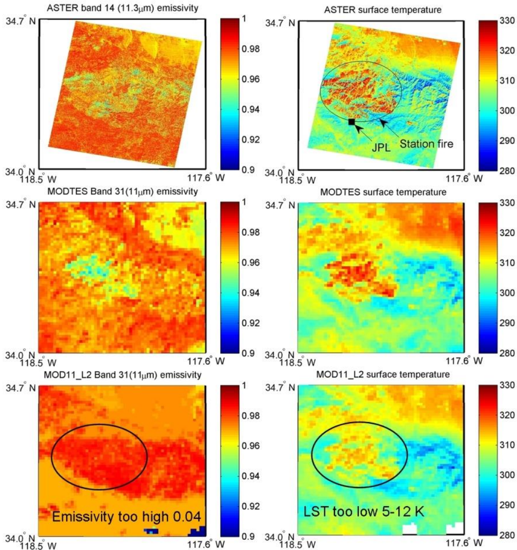
Figure 18. Emissivity images (left) and surface temperature images (right) for ASTER (top), MODIS TES (MODTES) (center) and MODIS SW (MOD11_L2) (bottom) products over the Station Fire burn scar just north of Pasadena, CA. Location of JPL in Pasadena and burn scar area indicated at top right. MODTES and ASTER results match closely; however, the MOD11_L2 temperatures are underestimated by as much as 12 K, due to an incorrect emissivity classification.
