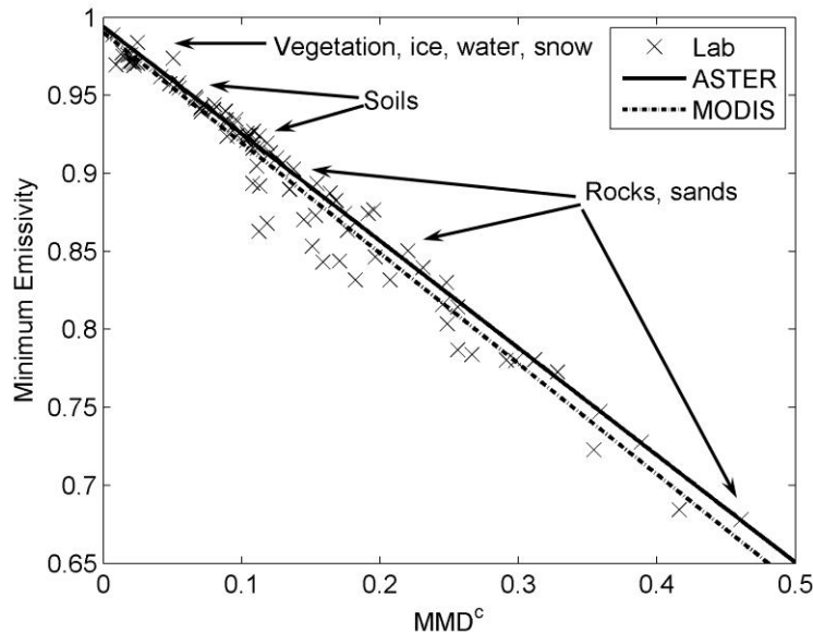
Figure 16. MODIS and ASTER calibration curves of minimum emissivity vs. MMD. The lab data (crosses) are computed from 150 spectra consisting of a broad range of terrestrial materials (rocks, sand, soil, water, vegetation, and ice).
