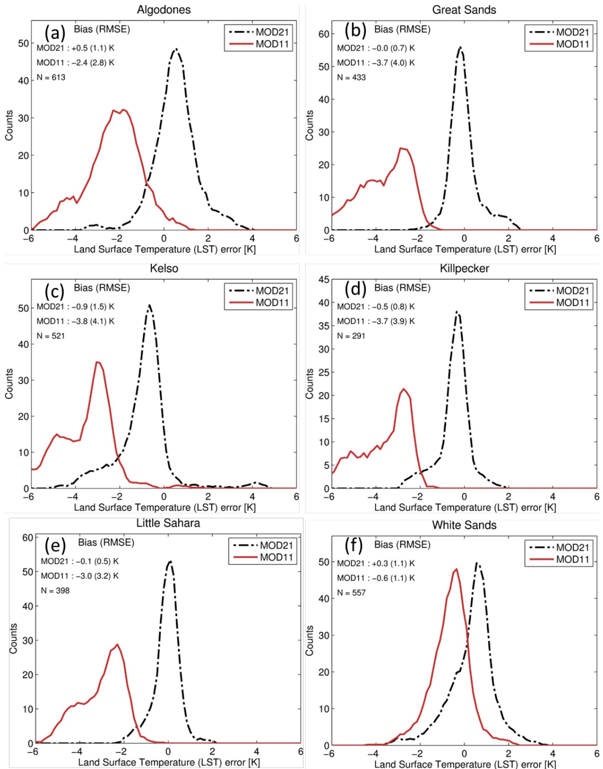
Figure 28. Histogram plots showing validation of the R-based method applied to the MODIS Aqua MOD11 and MOD21 LST products over six pseudo-invariant sand dune sites using all data during 2003-2005.
