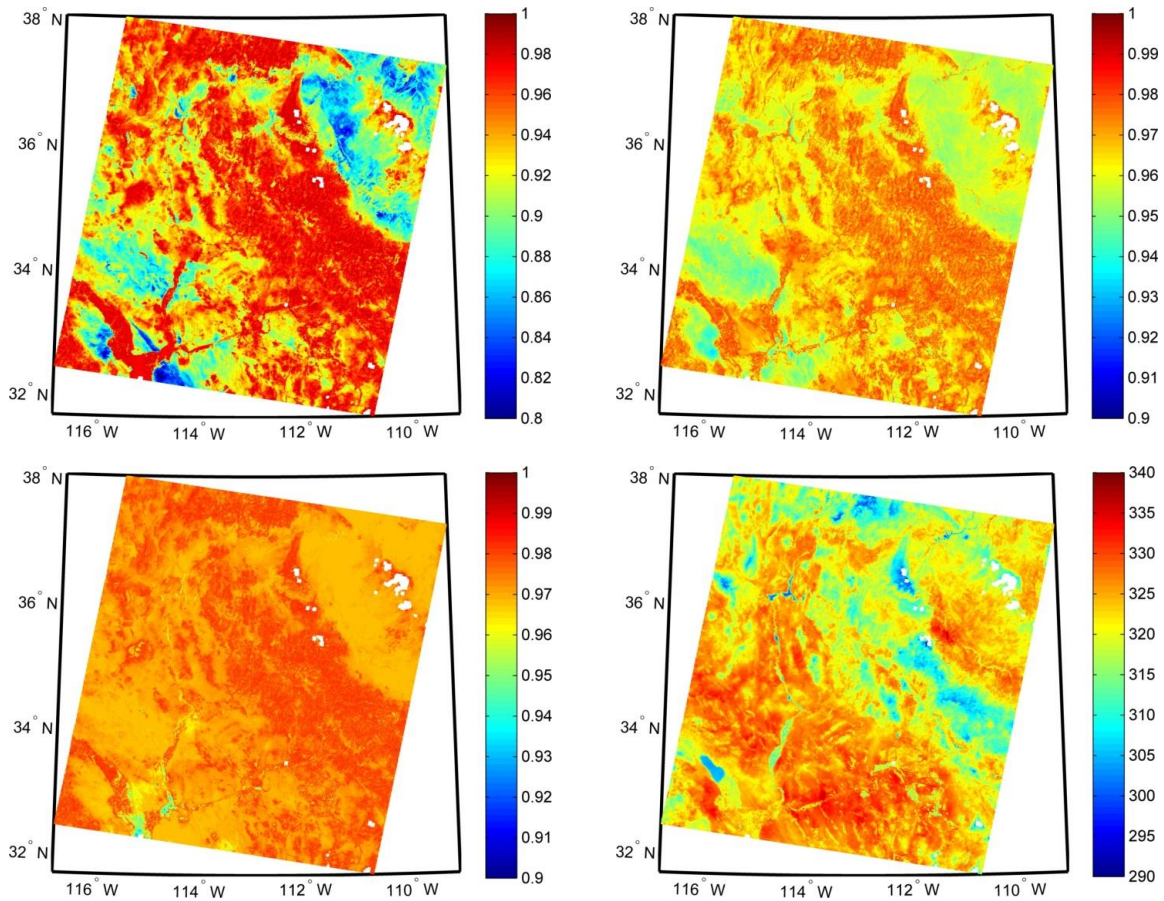
Figure 14. Clockwise from top left: MODIS cutouts of land surface emissivity for band 29 (8.55 \mu\text{m} ); band 31 (11 \mu\text{m} ), surface temperature (K) and band 32 emissivity (12 \mu\text{m} ); output from the TES algorithm over the Imperial Valley, southeastern California on 29 August 2004.
