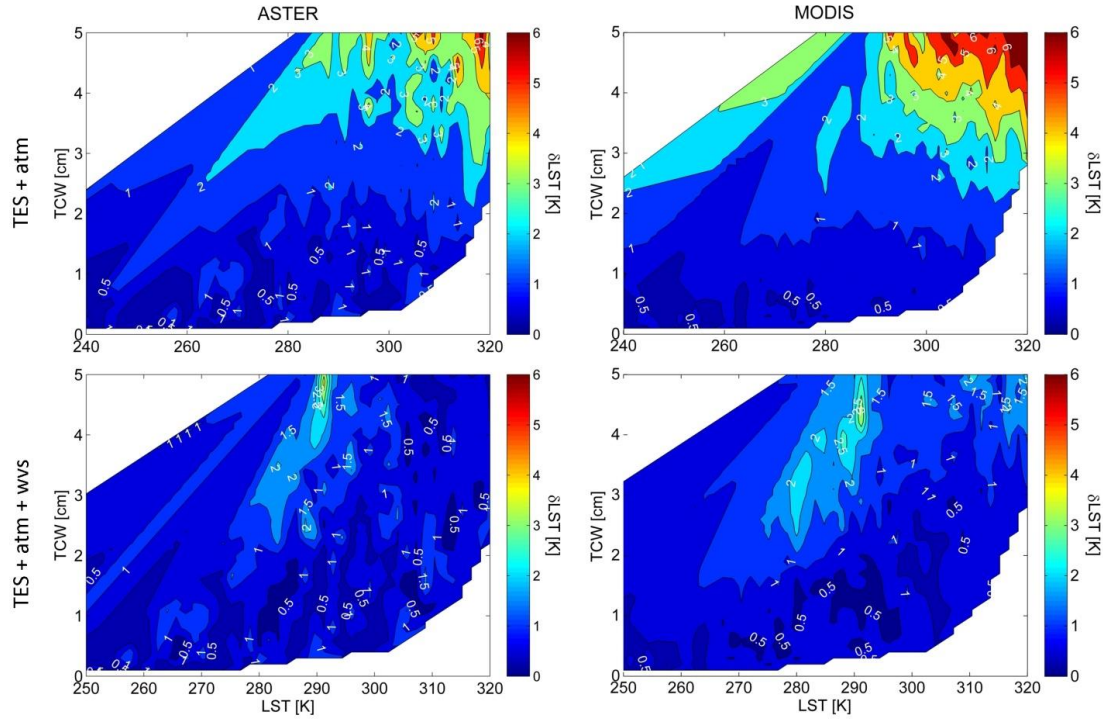
Figure 11. ASTER (left panels) and MODIS (right panels) LST uncertainty distributions plotted versus TCW and simulated LST for all end-member surface types (graybody, soils, sands, and rocks), for the TES algorithm including atmospheric error (TES+atm) and with the WVS method applied (TES+atm+wvs).
