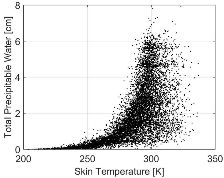
Figure 7. The total precipitable water versus skin temperature in the SeeBor profile used in the simulation for generating view angle and day–night-dependent coefficients.
