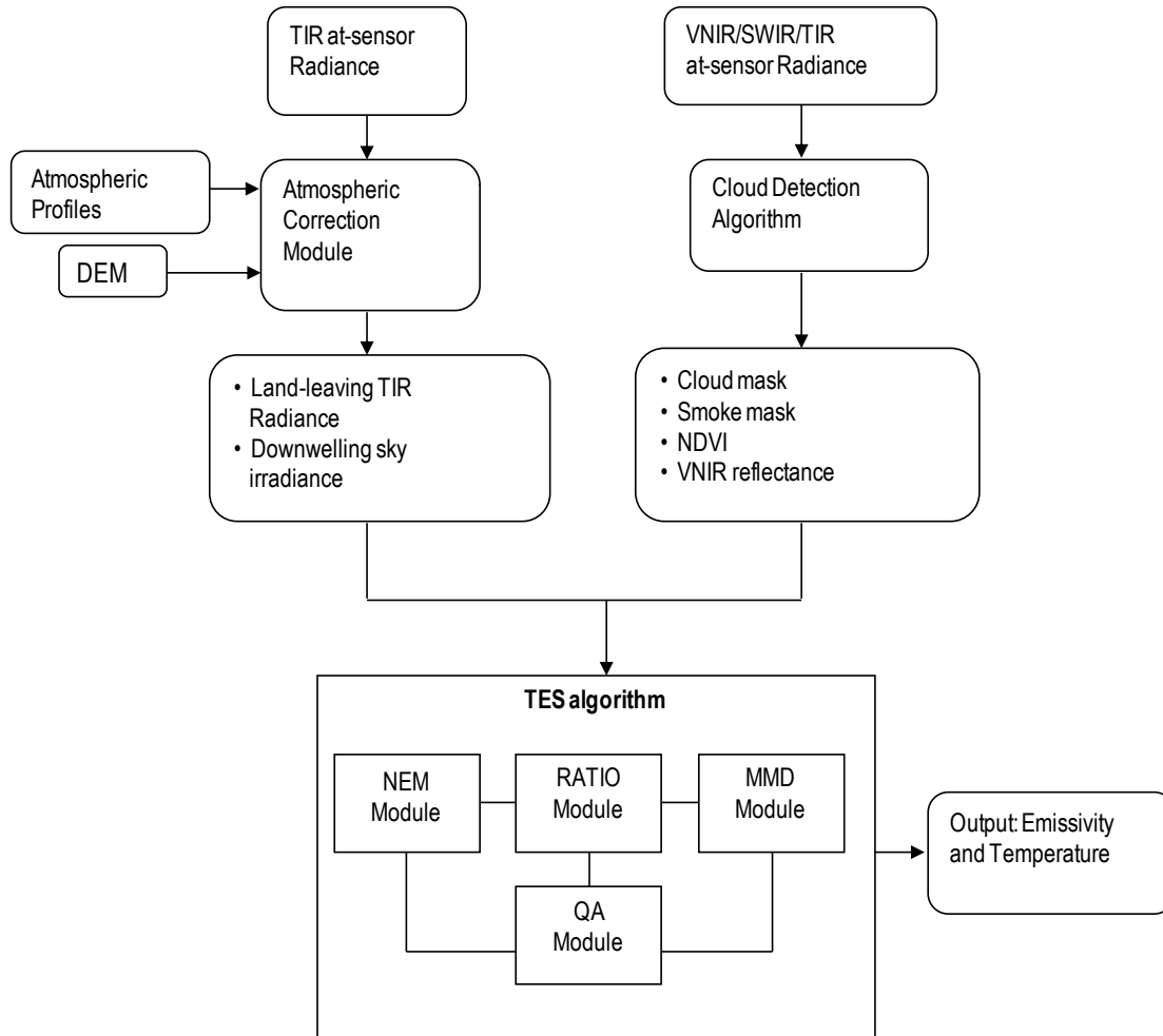
Figure 12. Flow diagram showing all steps in the retrieval process in generating the MODIS MOD21 LST&E product starting with TIR at-sensor radiances and progressing through atmospheric correction, cloud detection, and the TES algorithm.
