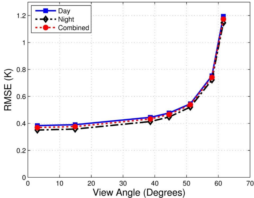
Figure 9. The RMSE between calculated and modeled surface brightness temperature for MODIS Aqua band 29 are plotted for corresponding view angles considered in the simulation using global radiosonde profile data as discussed in the text. The RMSE is less than 1 K for view angles less than 60°.
