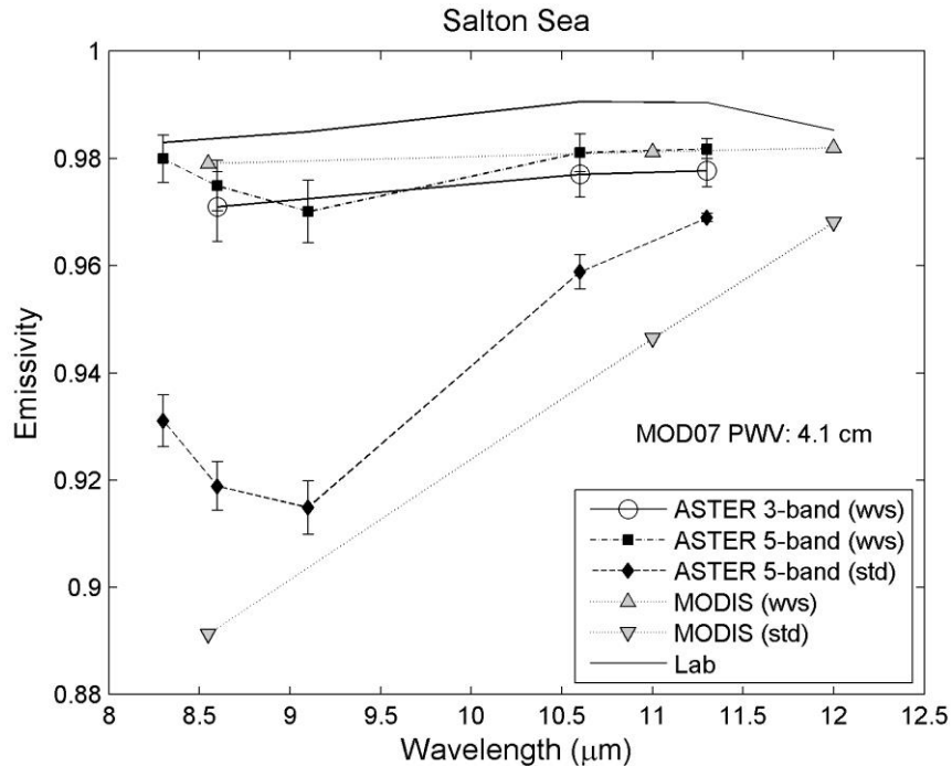
Figure 17. Emissivity spectra comparisons on June 15, 2000 over the Salton Sea between ASTER (3-band), ASTER (5-band), and MODTES, using the TES algorithm along with lab spectra of water from the ASTER spectral library. Results from the WVS method and the STD atmospheric correction are also shown. An estimate of the PWV from the MOD07 atmospheric product indicates very high humidity on this day.
