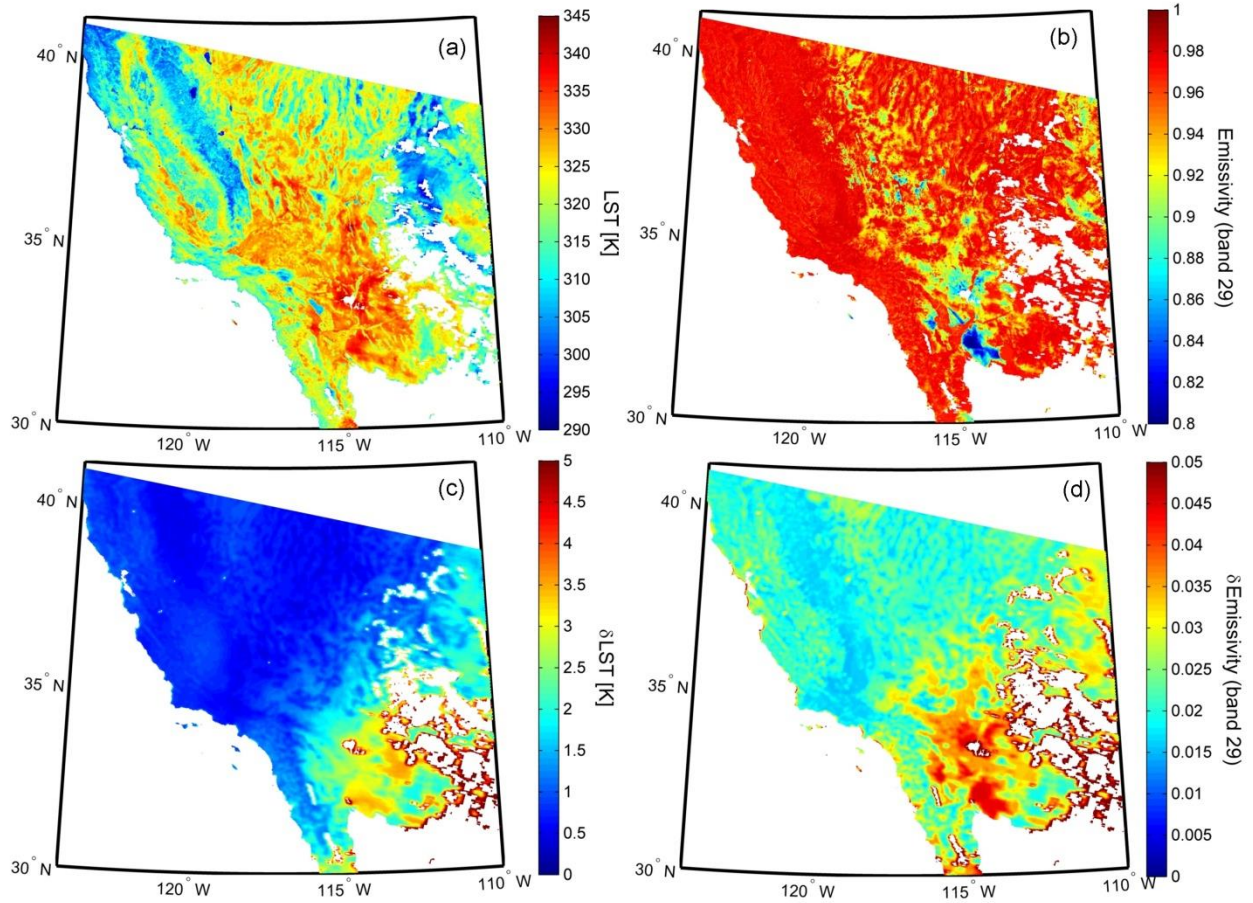
Figure 22. MODIS TES retrievals including WVS correction over the southwestern United States on 7 August 2004: (a) (top left) LST, (b) (top right) emissivity for band 29 (8.55 μm), (c) (bottom left) LST uncertainty, and (d) (bottom right) emissivity uncertainty for band 29 (8.55 μm). White areas over land indicate areas of cloud that have been masked out using the MOD35 cloud mask product.
