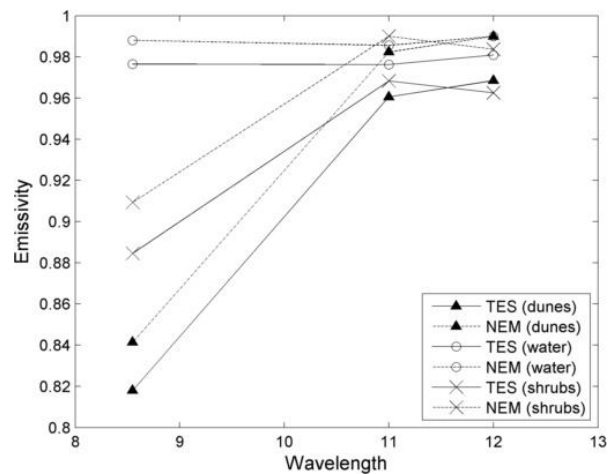
Figure 15. MODIS derived TES and NEM emissivity spectra for three different surface types for the MODIS cutout shown in Figure 11: Algodones Dunes, Salton Sea, and shrublands (mixed soil and vegetation). Details of the TES and NEM outputs from these spectra are shown in Table 5.
