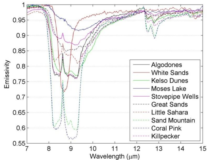
Figure 25. Laboratory-measured emissivity spectra of sand samples collected at ten pseudo-invariant sand dune validation sites in the southwestern United States. The sites cover a wide range of emissivities in the TIR region.
