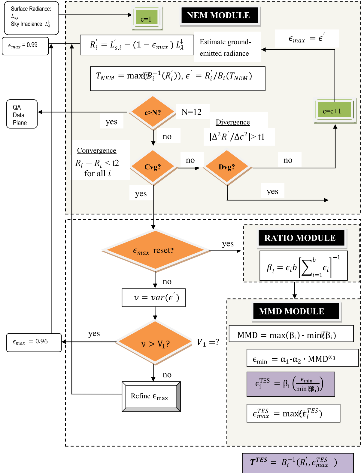
Figure 13. Flow diagram of the TES algorithm in its entirety, including the NEM, RATIO, and MMD modules.
