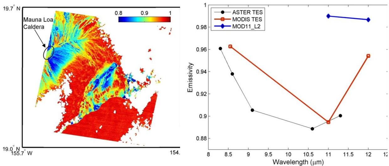
Figure 19. (left) ASTER band 12 (9.1 \mu\text{m} ) emissivity image over Mauna Loa caldera, Hawaii on 5 June 2000, and (right) emissivity spectra from ASTER, MODTES, and MOD11 emissivity classification. While ASTER and MODTES agree closely, MOD11 emissivities are too high, resulting in large LST discrepancies between MODTES and MOD11 (12 K) due to misclassification in bands 31 (11 \mu\text{m} ) and 32 (12 \mu\text{m} ).
