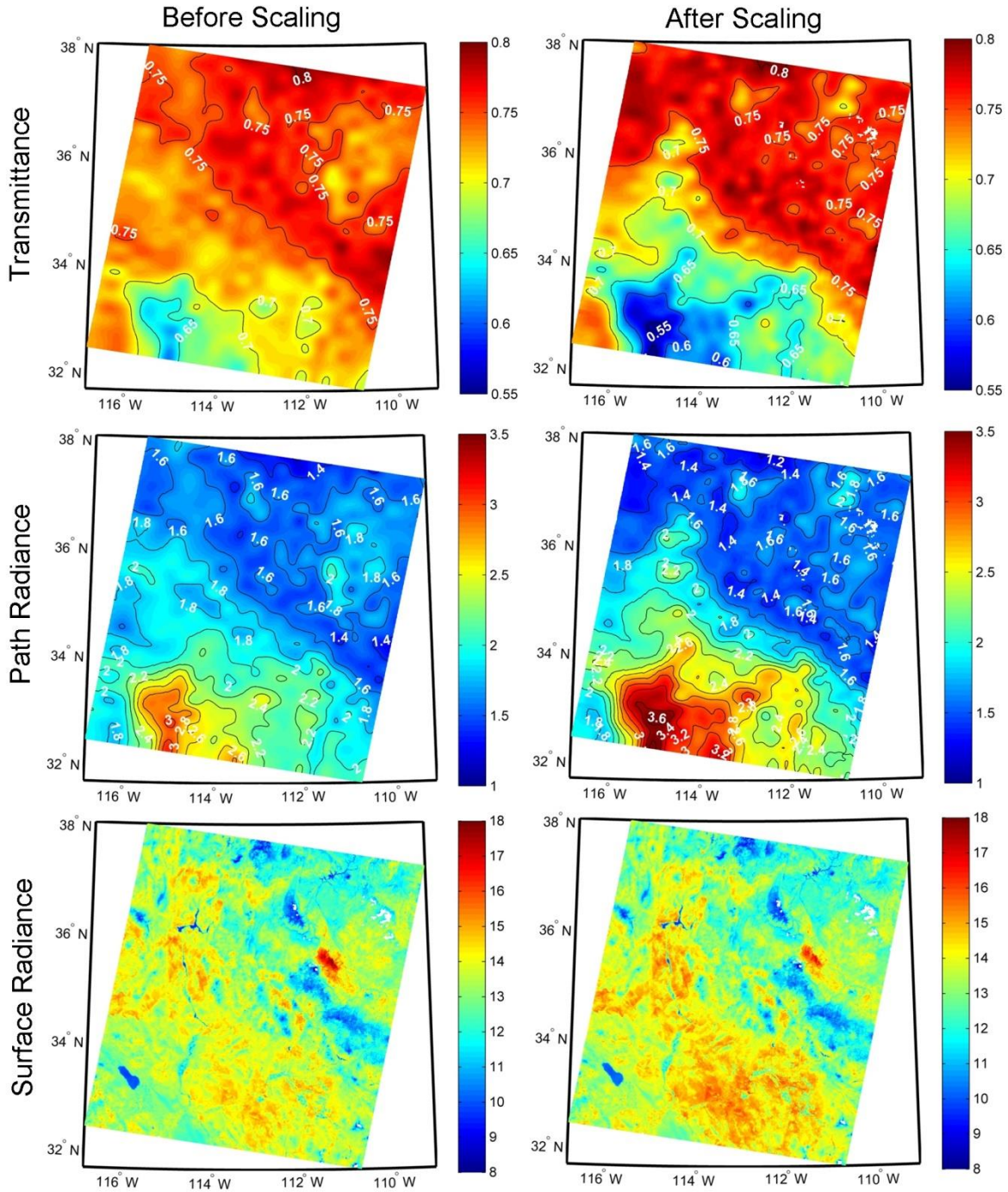
Figure 6. Comparisons between the atmospheric transmittance (top), path radiance ( W/m^2/\mu m^{-1} ) (middle), and computed surface radiance ( W/m^2/\mu m^{-1} ) (bottom), before and after applying the WVS scaling factor \gamma to a MODIS scene cutout shown in Figure 5. Results are shown for MODIS band 29 ( 8.55 \mu m ).
