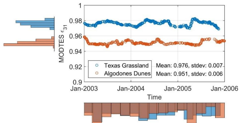
Figure 29. MODTES Emissivity retrievals for band 31 at the two sites show small fluctuations within the error range of 1% from the mean values. The histograms on the margins show a consistently high density of the data around the mean for each of the sites.
