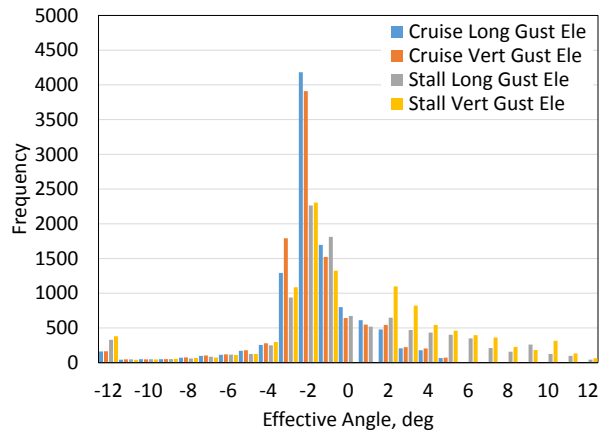
(d) SDynConFreeSM histogram of elevator gust responses.
