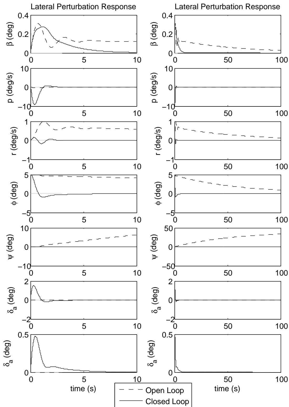
Figure 6.13: Roll hold perturbation check.
