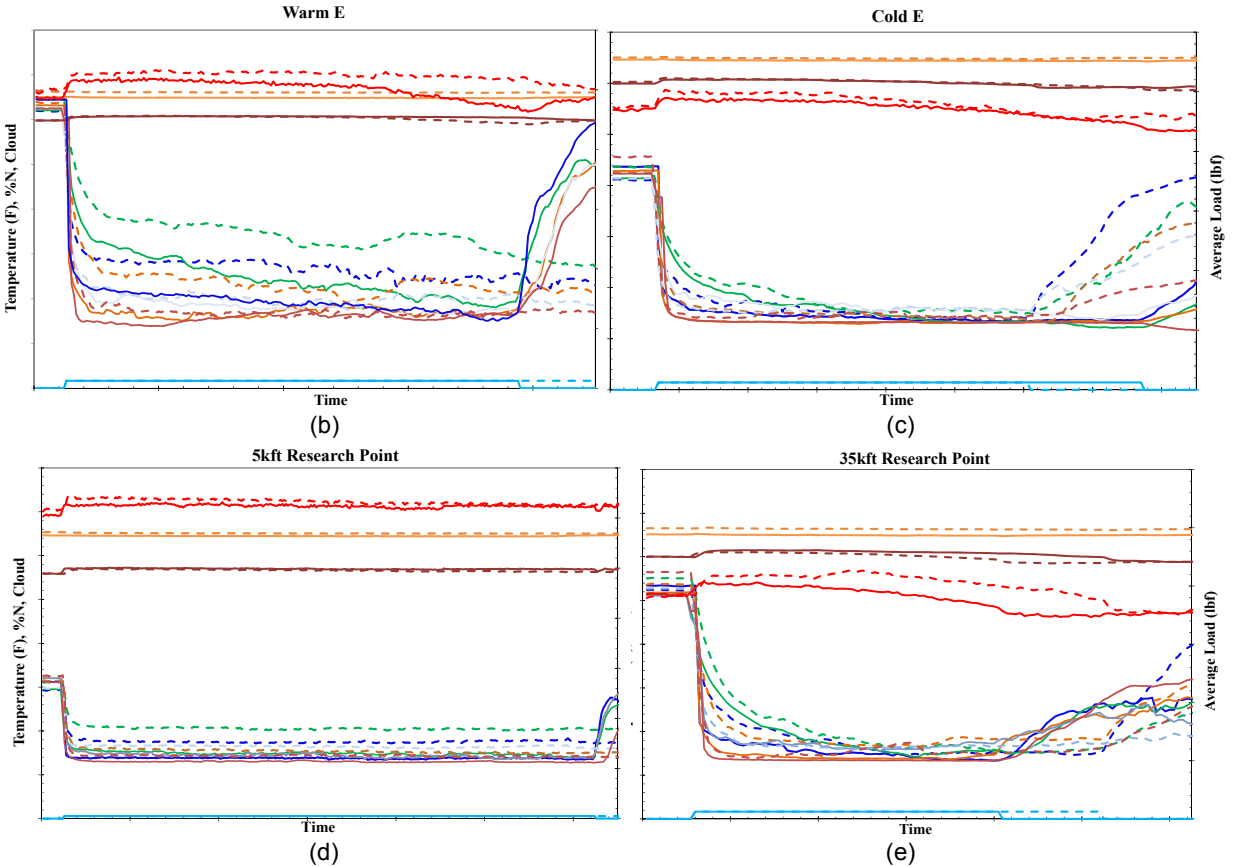
Figure 8.—Comparison of PSL LF11 and LF01 engine response.
