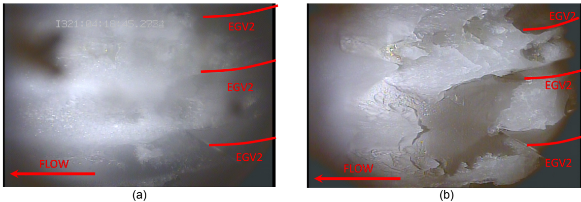
Figure 21.—Ice accretion at (a) 5 kft research point and (b) FLT850 at respective CRB times.
