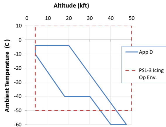
Figure 3.—PSL-3 icing operating envelope.
