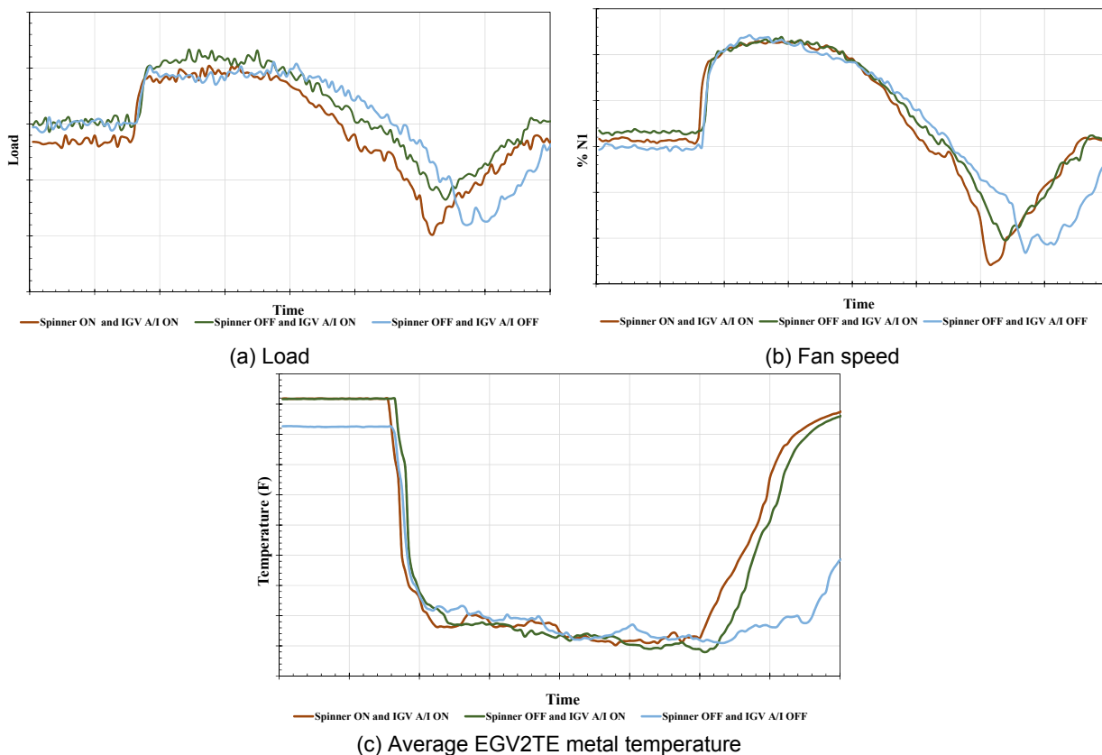
Figure 20.—Engine configuration effects on (a) load, (b) fan speed, and (c) EGV2 trailing edge metal temperature.
