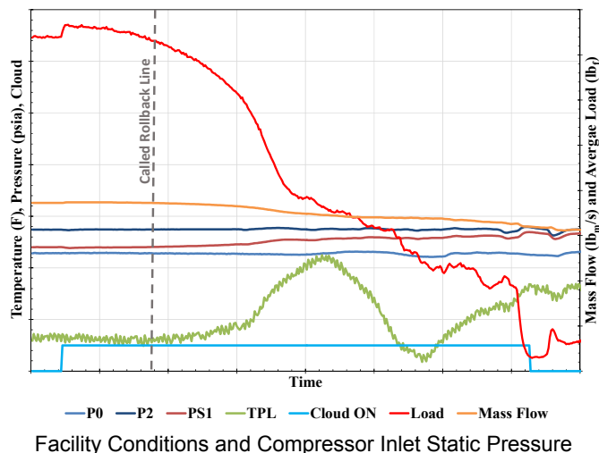
Figure 14.—Pressure and temperature response during full rollback.
