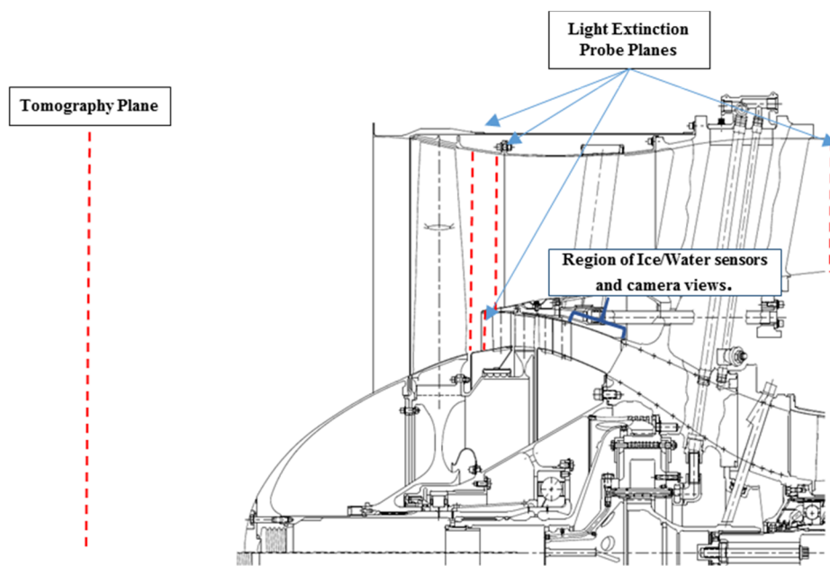
Figure 4.—Advanced instrumentation locations in an unmodified ALF502R-5 engine fan and booster section (Ref. 3).
