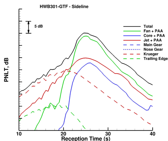
Figure 21 – Noise components and total PNLT for HWB301-GTF on sideline (65)
