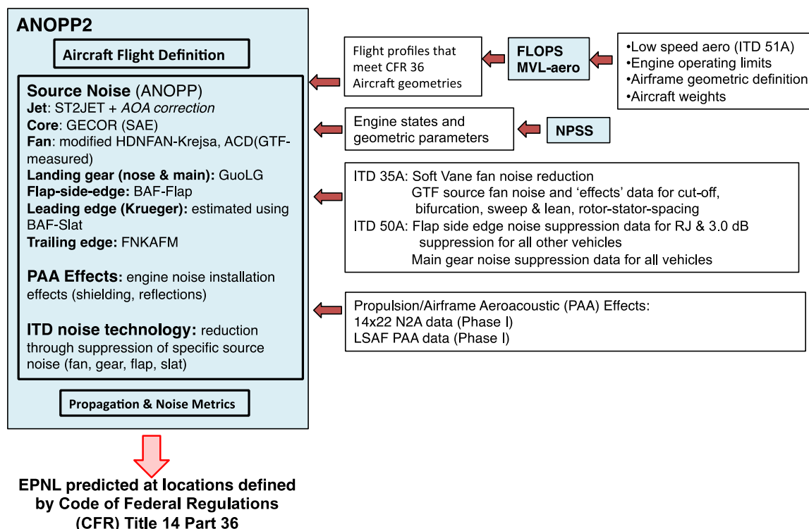
Figure 19 – Overview of the process used for the final 2015 ERA noise assessments (65).
