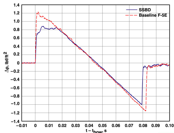
Figure 29 – Comparison of modified SSBD and baseline booms at the ground (90).
