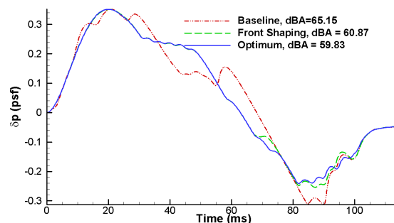
Figure 31 – Comparison of ground signatures (103).
