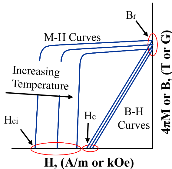
Figure 4.—Sample demagnetization curve.
