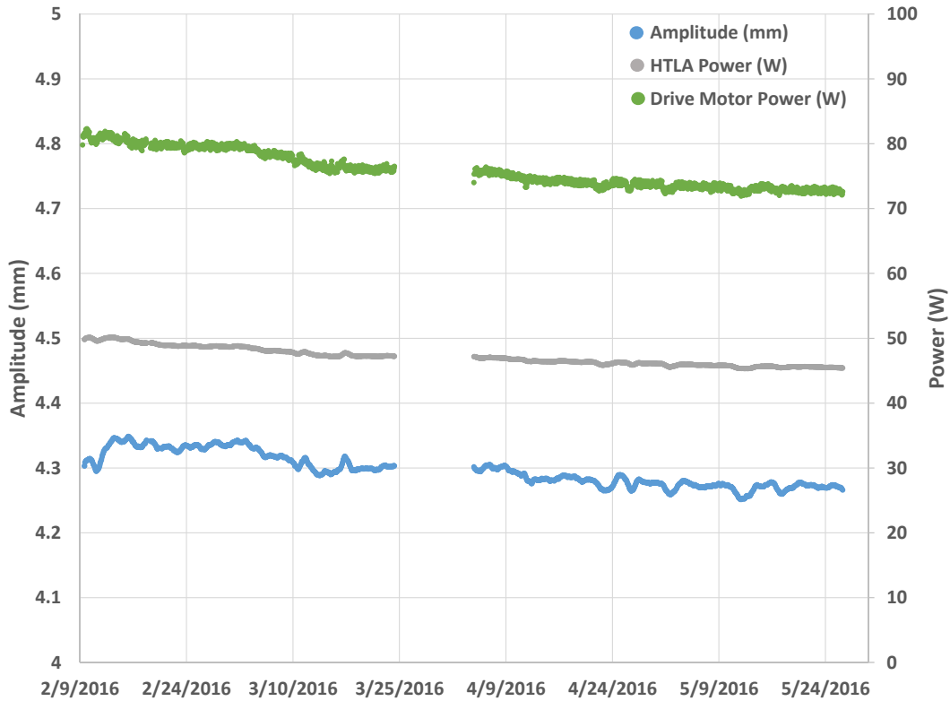
Figure 13.—Endurance test performance plot.
