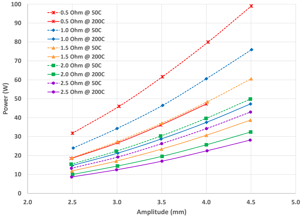
Figure 11.—Power vs. amplitude at 50 and 200 °C for each load tested.
