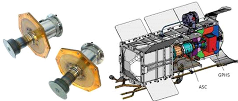
Figure 1.—Pair of ASCs and ASRG cutaway diagram.
