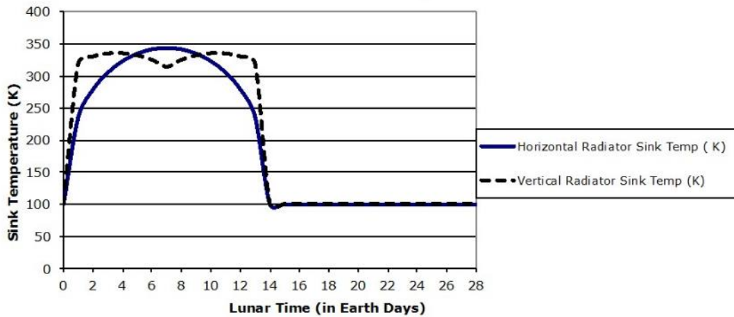
Figure 2.—Plot of lunar sink temperature (Ref. 4).
