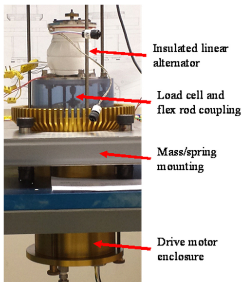
Figure 8.—HTLA coupled to the drive motor.
