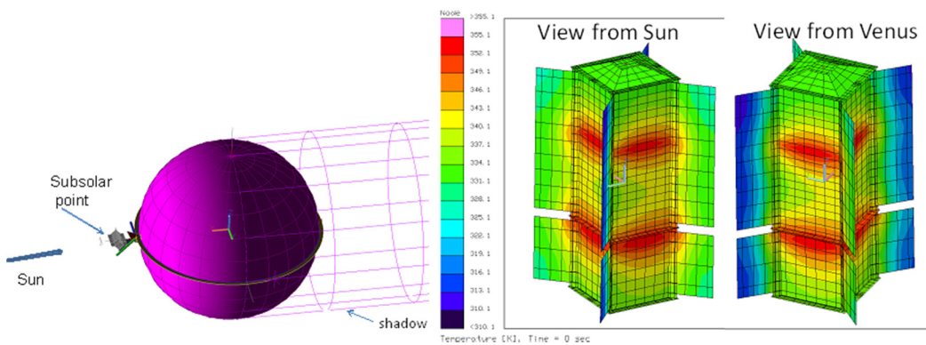
Figure 3.—Depiction of spacecraft position during Venus swing-by and ASRG thermal analysis (Ref. 6).
