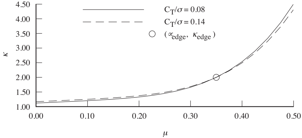
Figure 12-6. Induced power factor for rotor in edgewise flight.
