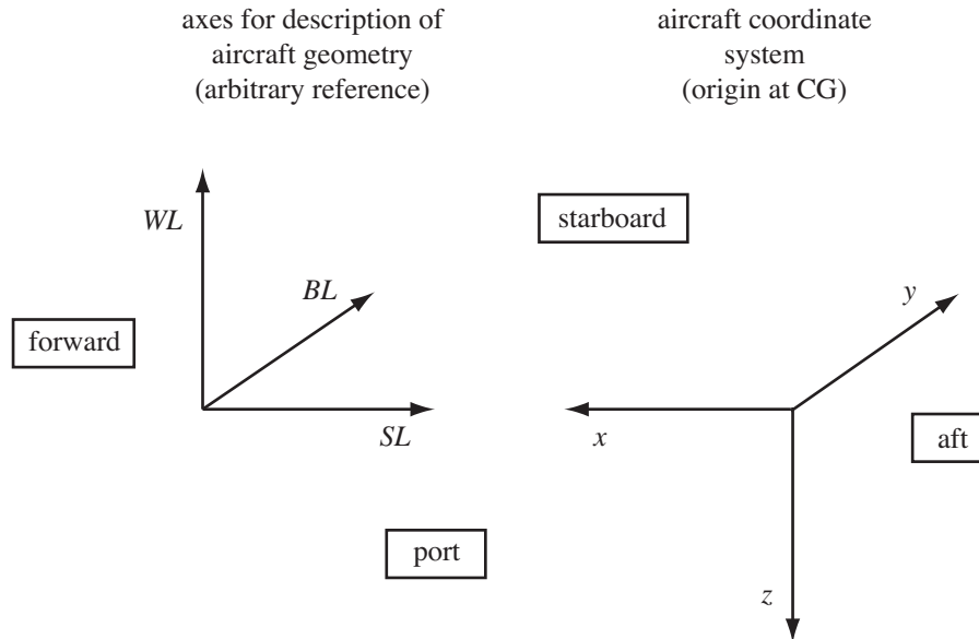
Figure 8-2. Aircraft geometry.
