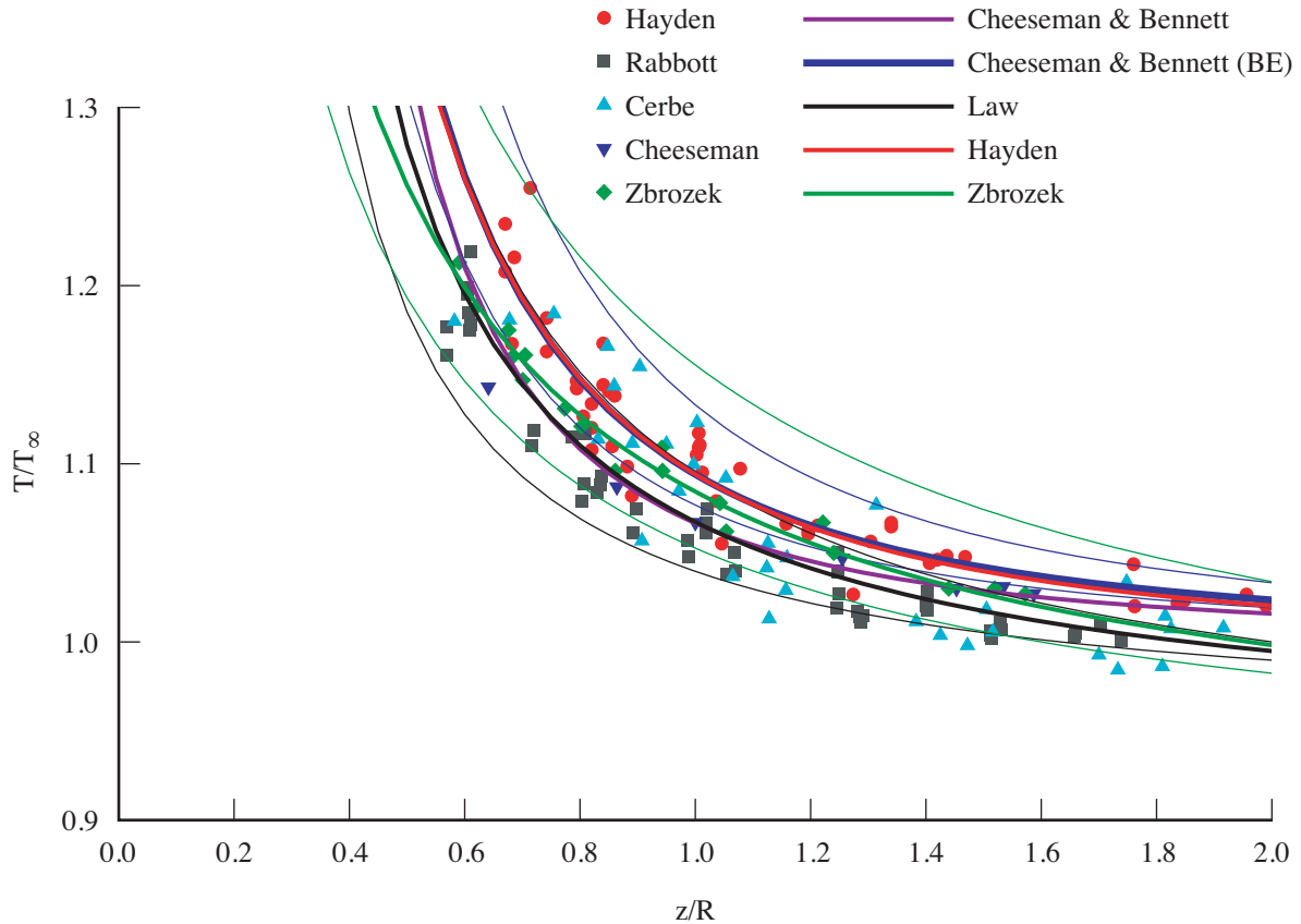
Figure 12-2. Ground effect models (hover).
