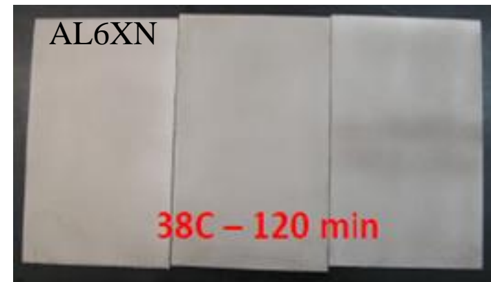
@ 504 Hours of ASTM B117 Exposure
