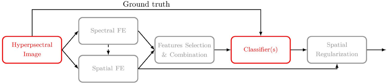
Fig. 4. General framework for the classification of hyperspectral images. FE means feature extraction.
