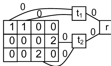
Fig. 17. Example of addition of extra vertices t_1, t_2, r to the image graph for construction of an MSF rooted on markers 1 and 2. Nonmarker pixels are denoted by "0."
