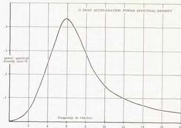
Figure 14: The acceleration power spectral density of this study. (Courtesy of North American Aviation, Inc.)
