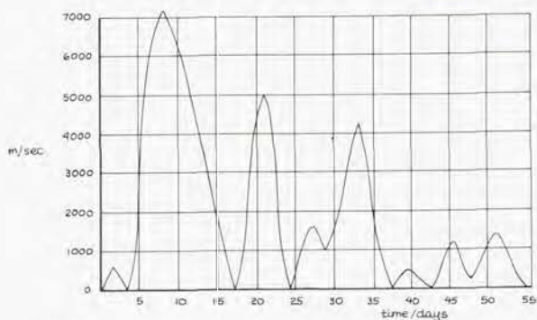
FIGURE 1 VELOCITY REQUIREMENT OVER NOMINAL FOR DEPARTURE FROM EARTH ORBIT TO MOON. LUNAR ORBIT INCLINATION 18.50^\circ , EARTH ORBIT ALTITUDE 485 KM, EARTH ORBIT INCLINATION 30^\circ
