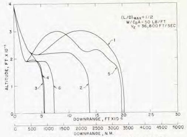
FIG 2 RE-ENTRY TRAJECTORIES FOR PARABOLIC VELOCITY
