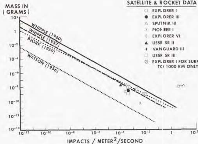
FIGURE 7. METEOROID ENVIRONMENT
