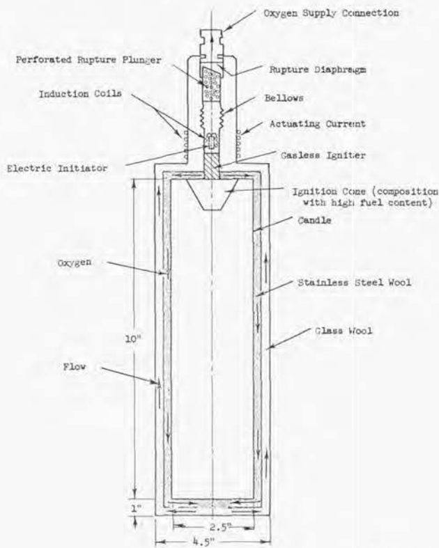
SCHEMATIC OF A ONE MAN-DAY PERCHLORATE CANDLE
