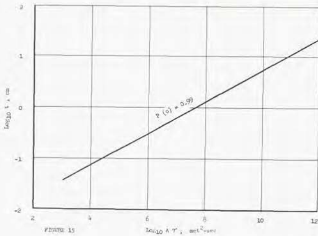
ALUMINUM SKIN THICKNESS REQUIRED FOR METEOROID PROTECTION
