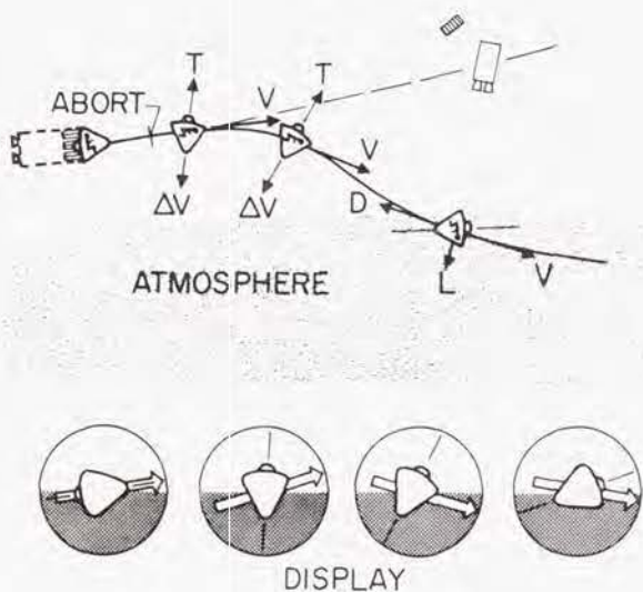
Figure 13.- Reorientation after superorbital abort.
