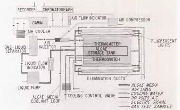
Photosynthetic Oxygen Regeneration System
