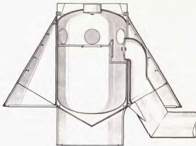
FIGURE 12. HUB SECTION
