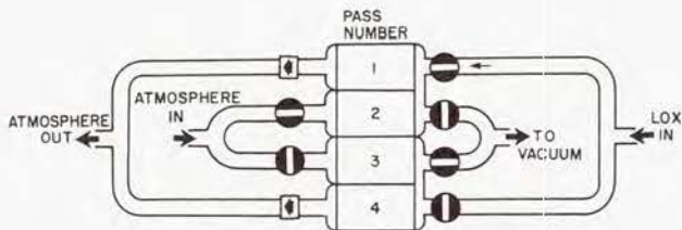
FIGURE 12. REGENERABLE CO 2 FREEZE-OUT SYSTEM
