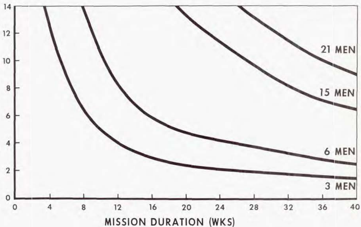
FIGURE 13. SATURN C-I BOOSTER REQUIREMENT
