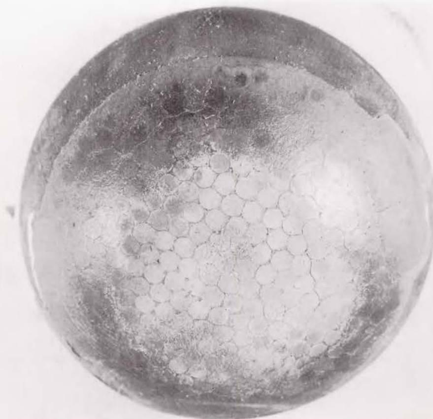
FIGURE 21. ZIRCONIA ROD TYPE NOSE TIP AFTER SECOND TEST AT 4100°F.
