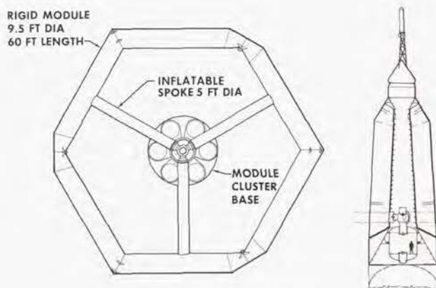
FIGURE 9. SPACE STATION CONFIGURATION (150 FT DIA)
