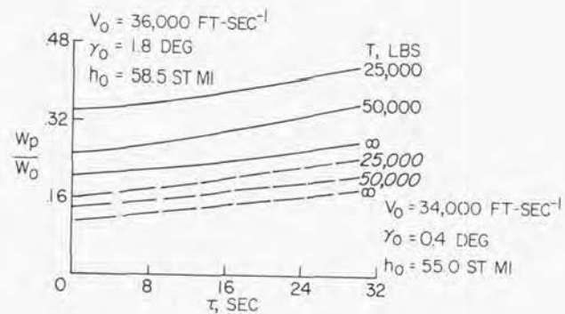
Figure 16.- Abort fuel requirements with time delay.
