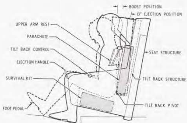
Figure 4 2 POSITION EJECTION SEAT
