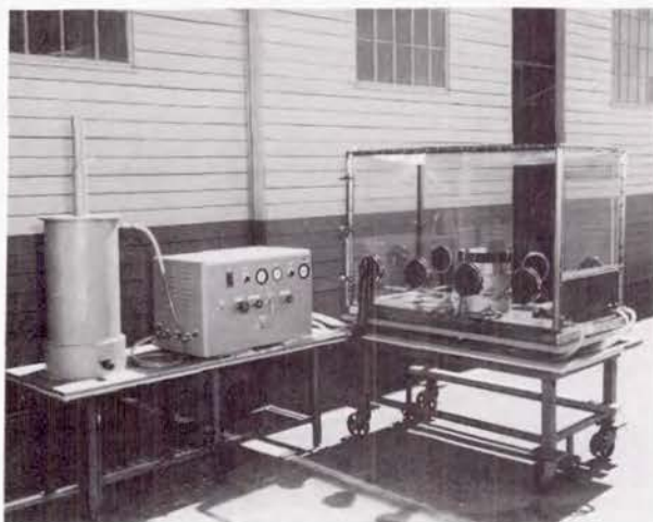
FIGURE 4 RANGER ASEPTIC ASSEMBLY EQUIPMENT
