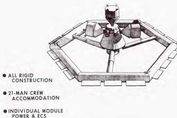
FIGURE 10. SELECTED CONFIGURATION
