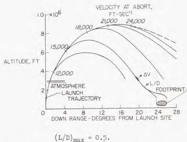
Figure 9.- Range after suborbital abort.
