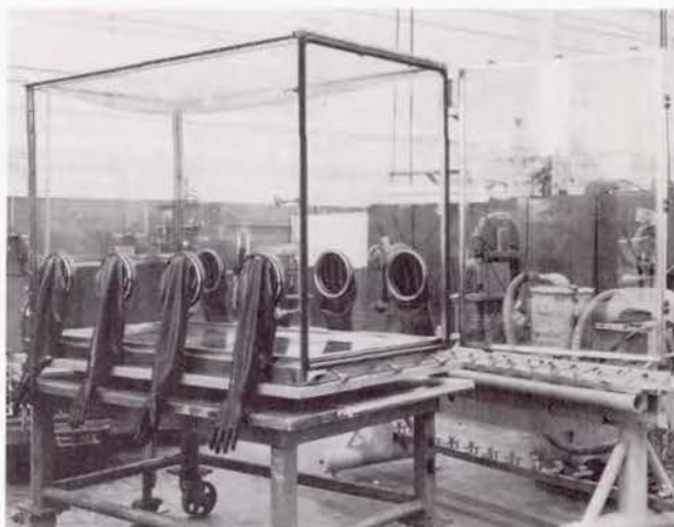
FIGURE 5 RANGER ASEPTIC ASSEMBLY GLOVE BOX
