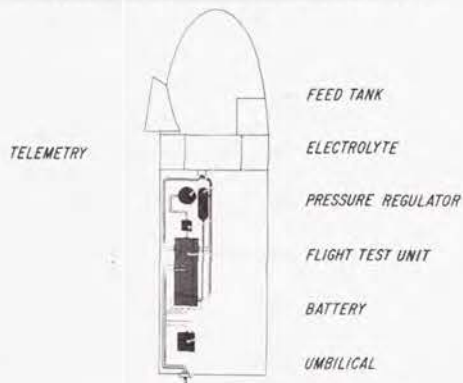
SIMPLIFIED SYSTEM DIAGRAM INTEGRATED SCIENTIFIC PASSENGER POD
