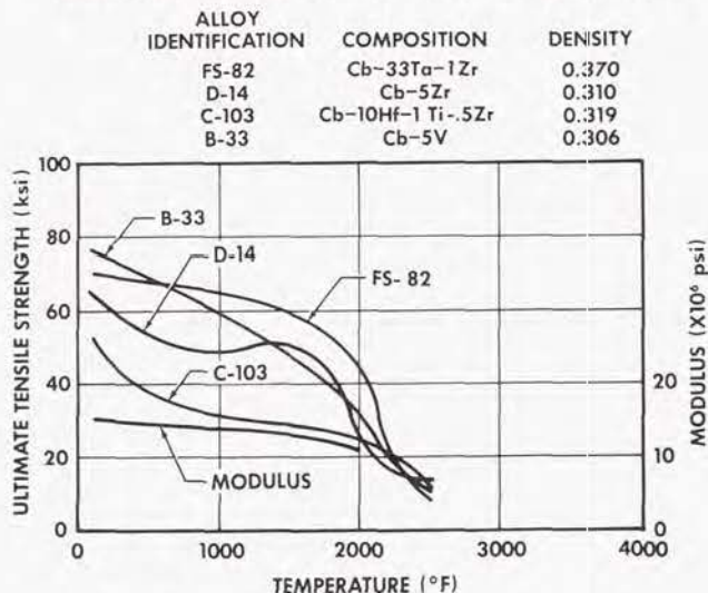
FIGURE 7. ULTIMATE TENSILE STRENGTH (GUARANTEED) AND MODULUS OF MODERATE STRENGTH COLUMBIUM BASE ALLOYS AS A FUNCTION OF TEMPERATURE.
