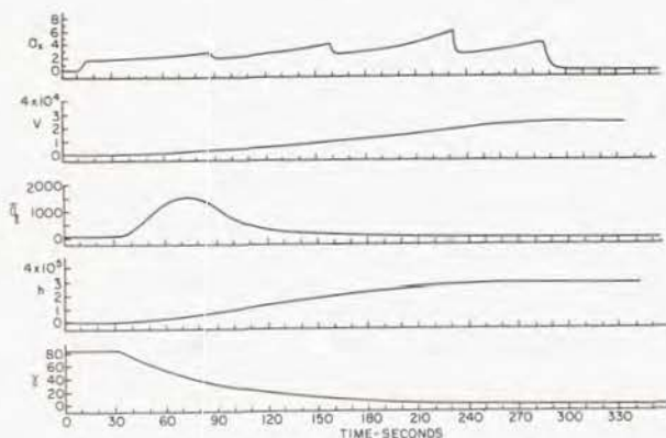
FIGURE 21. Acceleration profile used to simulate a 4-stage launch vehicle on the AMAL Human Centrifuge.
