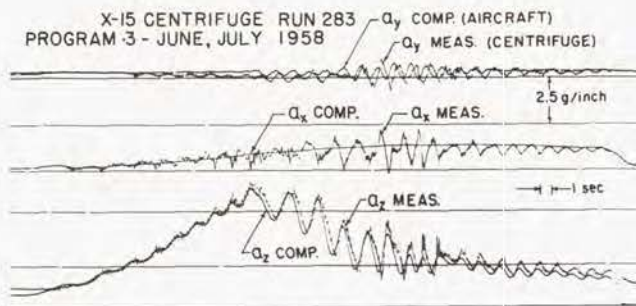
Figure 6: Accelerations computed for an X-15 reentry with dampers off, and Navy centrifuge simulation by pilot-computer control. (Official U. S. Navy photograph).
