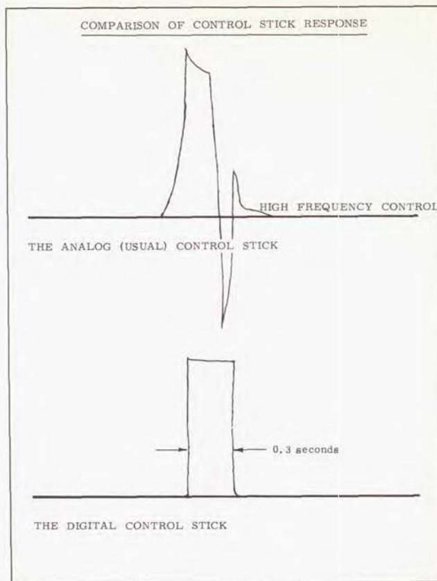
Figure 19: Typical control pulses for the analog and digital controllers.
