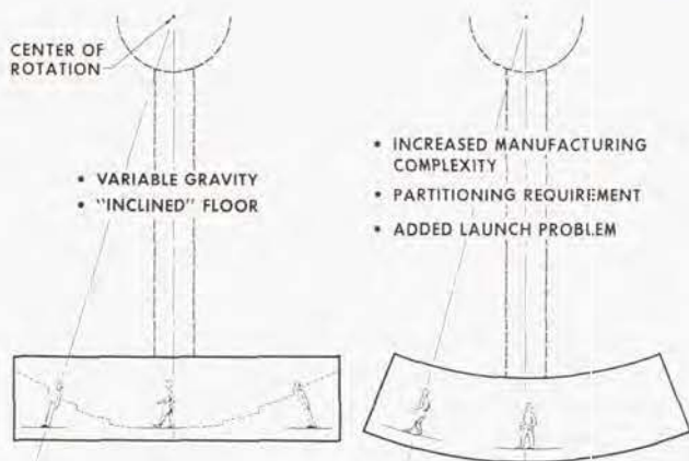
FIGURE 5. MODULE DESIGN CONSIDERATIONS
