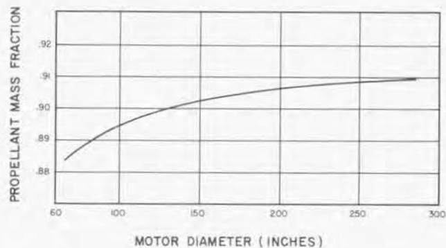
FIG. 3 SOLID PROPELLANT MOTOR MASS FRACTION VS. MOTOR DIAMETER
