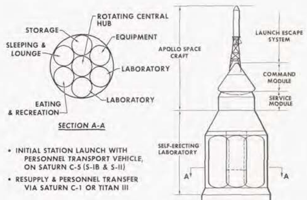
FIGURE 3. LAUNCH CONFIGURATION
