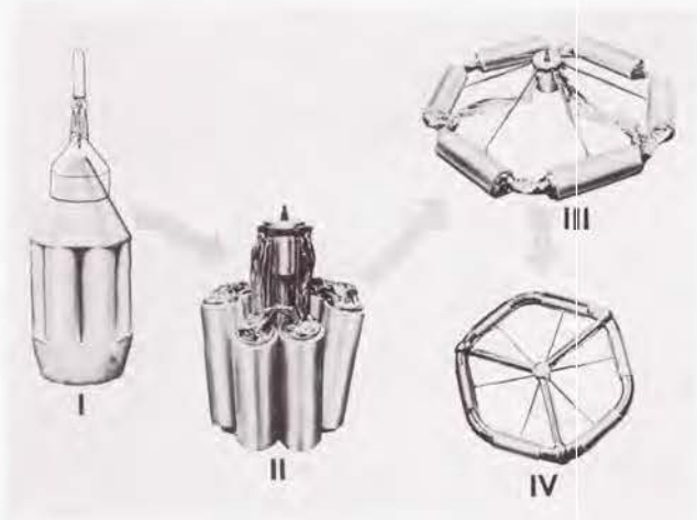
FIGURE 1. ERECTION SEQUENCE
