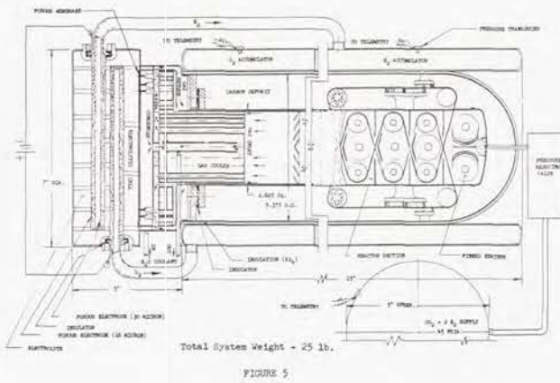
OXYGEN REGENERATION (FLIGHT TEST SYSTEM)
