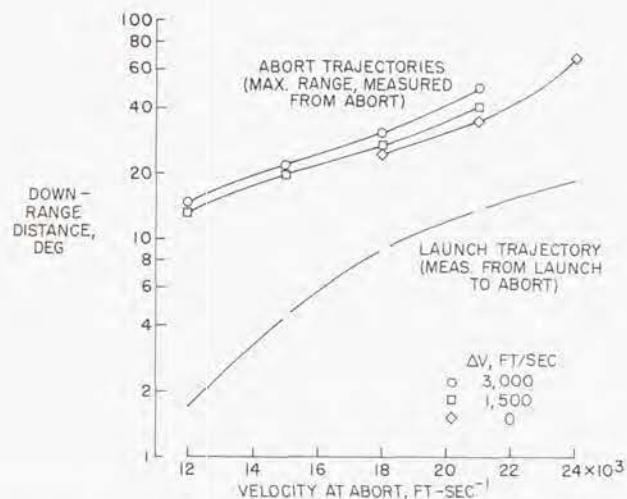
Figure 12.- Maximum down-range distance obtained following an abort.
