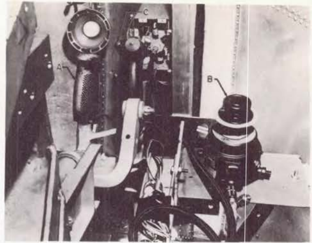
A. Mercury Type Control Handle B. Oxygen Regulator C. Visual Response Button
