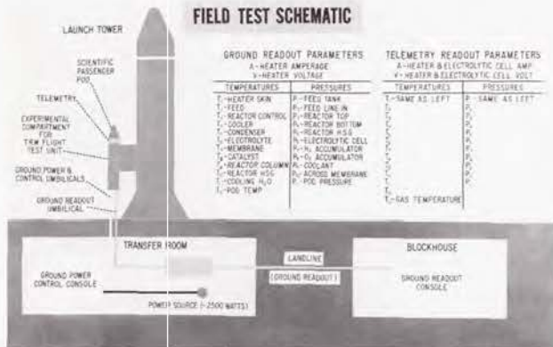
FIELD TEST SCHEMATIC
