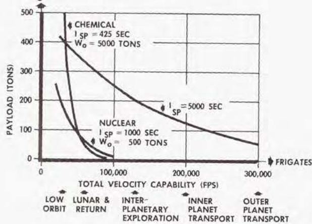
FIGURE 11 PAYLOAD VELOCITY CAPABILITIES CHEMICAL & NUCLEAR VEHICLES (PRACTICAL STAGING)
