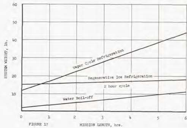
SYSTEM WEIGHT AS A FUNCTION OF MISSION TIME
