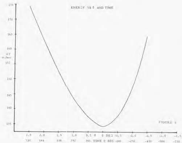
VELOCITY INCREMENT VS. TIME OF LAUNCH FOR ROTATION OF A 225 KM ORBIT INTO THE DESIRED ORBITAL PLANE (VARIABLE LAUNCH AZIMUTH)
