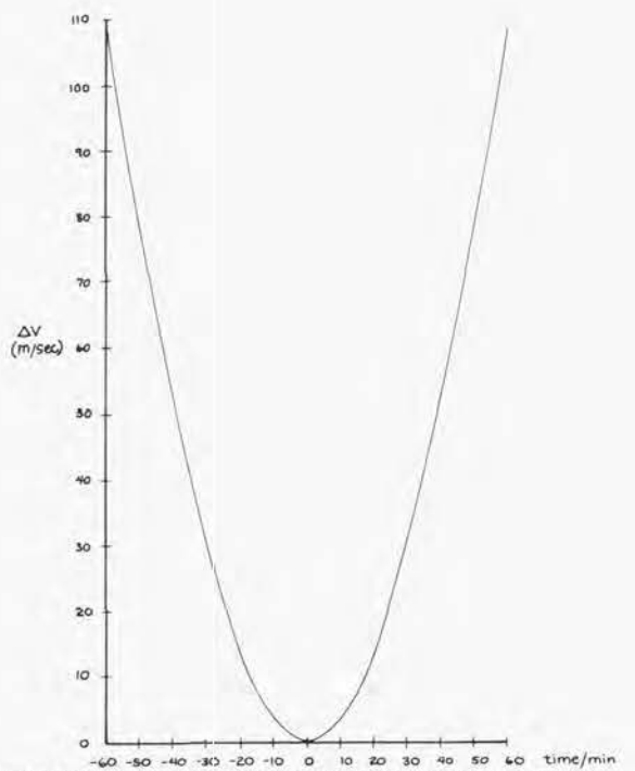
VELOCITY INCREMENT VS. TIME OF LAUNCH FOR ROTATION OF A 225 KM ORBIT INTO THE DESIRED ORBITAL PLANE (VARIABLE LAUNCH AZIMUTH)
