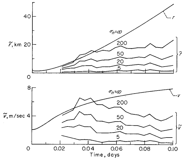
FIGURE 4.—Time histories of the estimation errors for various magnitudes of observation error.
