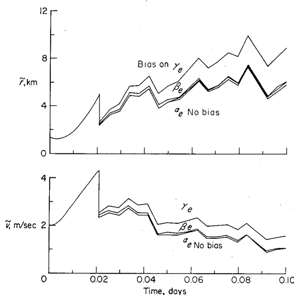
FIGURE 10.—Time histories of the errors in estimate with 5 sec arc uncompensated bias on \alpha_e , \beta_e , \gamma_e , \sigma_n = 20 sec arc.
