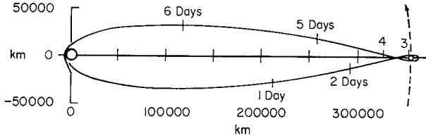
FIGURE 2.—Reference trajectory for circumlunar mission.
