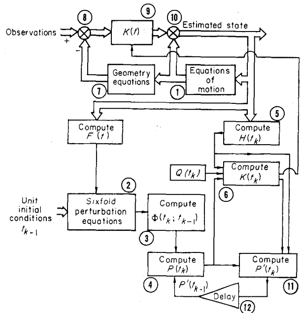
FIGURE 1.—Block diagram of trajectory estimation system.
