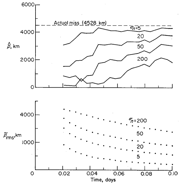
FIGURE 7.—Performance of the system in estimating the miss at nominal perilune for various magnitudes of observation errors.
