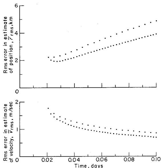
FIGURE 9.—Root-mean-square estimation errors for two different observation rates.
