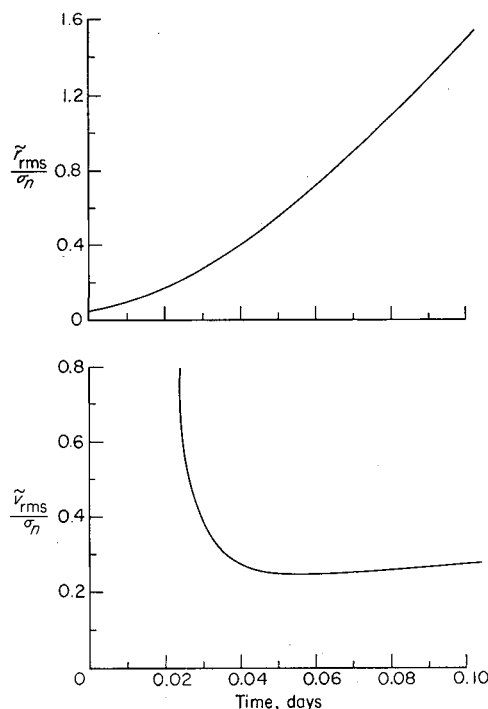
FIGURE 11.—Root-mean-square estimation errors for a minimum data method of trajectory estimation.
