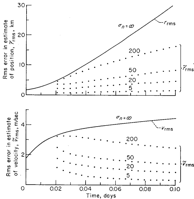
FIGURE 6.—Root-mean-square estimation errors for various standard deviations of observation errors.
