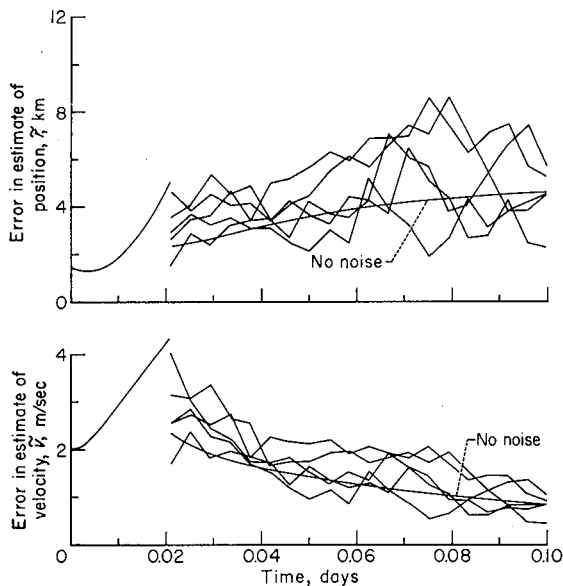
FIGURE 5.—Time histories of the estimation errors for various observation error samples; \sigma_n = 20 sec arc.
