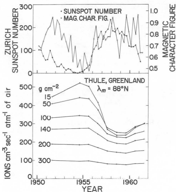
FIGURE 16-31.—Relation of the cosmic-radiation cycle to the sunspot cycle. (Data in top part give quarterly Zurich sunspot number and quarterly planetary magnetic character figure. Data in bottom part give cosmic-ray ionization measured with standard ionization chambers in balloon at selected depths (in g/cm 2 ) in atmosphere. Note that at large depths, where only high-energy particles penetrate, the modulation disappears. From Ref. 54.)
