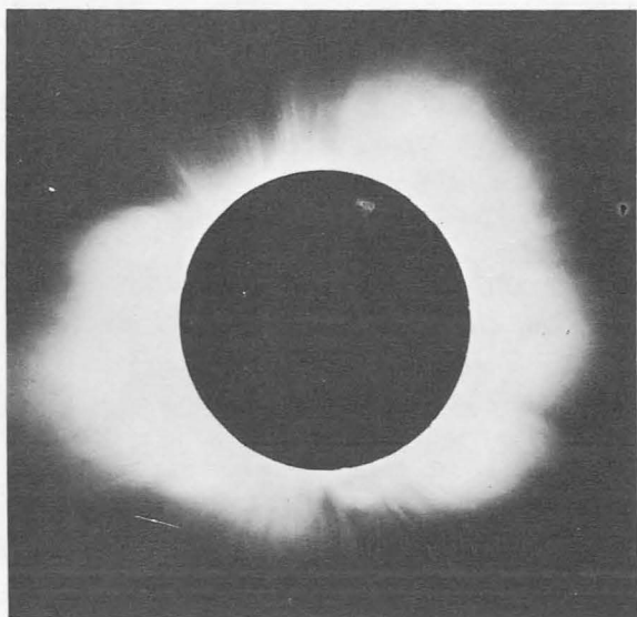
FIGURE 16-1.—Solar corona, photographed at the total eclipse of June 8, 1918, Green River, Wyoming.
