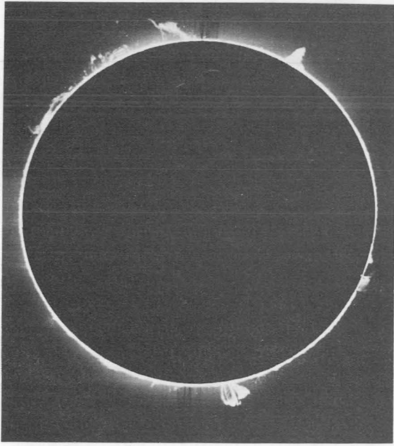
FIGURE 16-17.—Solar prominences. Photospectroheliograph of the whole edge of the Sun, taken with the calcium K line, December 9, 1929.
