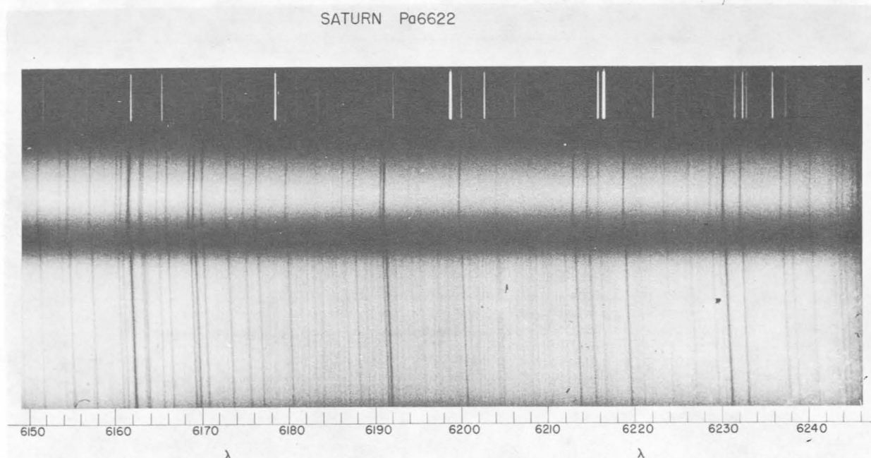
FIGURE 17-5.—A Palomar 200-in. reflector coude spectrogram of Saturn taken by Münch with the slit parallel to the equator. Original dispersion 3.3 \text{ \AA/mm} . Methane lines can be separated from Fraunhofer lines by the difference in inclination. Note the lack of any methane in the spectrum of the rings at the top.
