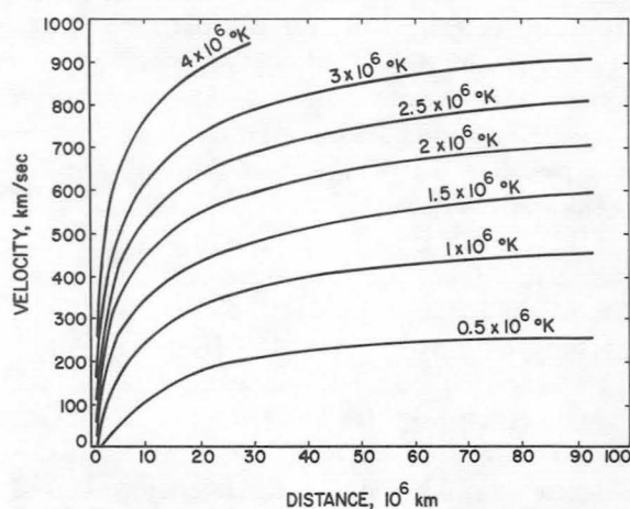
FIGURE 16-6.—Parker's spherically symmetric hydrodynamic expansion function, giving velocity as function of radial distance from Sun for an isothermal solar corona having specified values of temperature at unit radius, taken to be 10^6 km. (From Ref. 16.)
