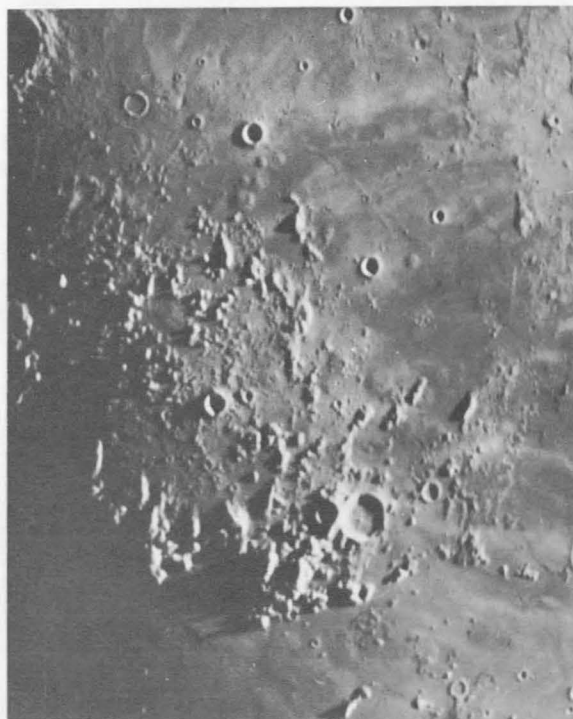
FIGURE 18-4.—Domes (some showing central craters) near Tobias Mayer, small crater which is 30 km in diameter (lower central part). Rhinhold is partly shown in upper left. (Photograph courtesy Mt. Wilson and Palomar Observatories.)
