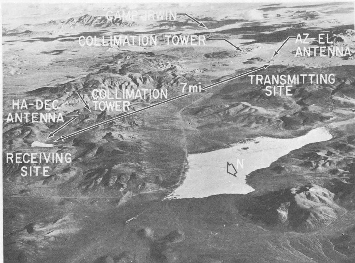
FIGURE 9-2.—Goldstone tracking station.
