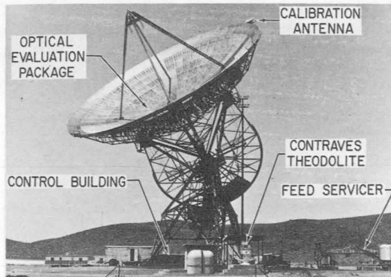
FIGURE 9-3.—85-ft. diameter Goldstone hour angle-declination (HA-Dec) antenna.
