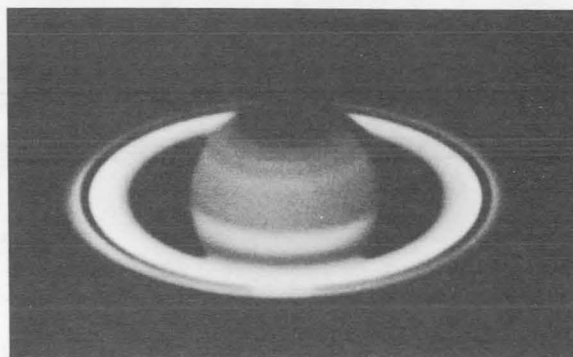
FIGURE 17-4.—Saturn in blue light. 200-in. photograph, courtesy of Mt. Wilson and Palomar Observatories.
