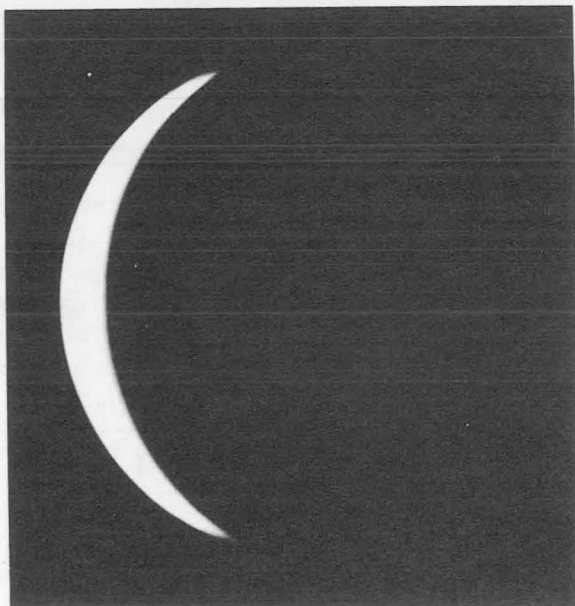
FIGURE 18-10.—Venus in blue light. (Photograph from 200-inch reflector, Mt. Wilson and Palomar Observatories. Note lack of irregularities in terminator and absence of other features.)
