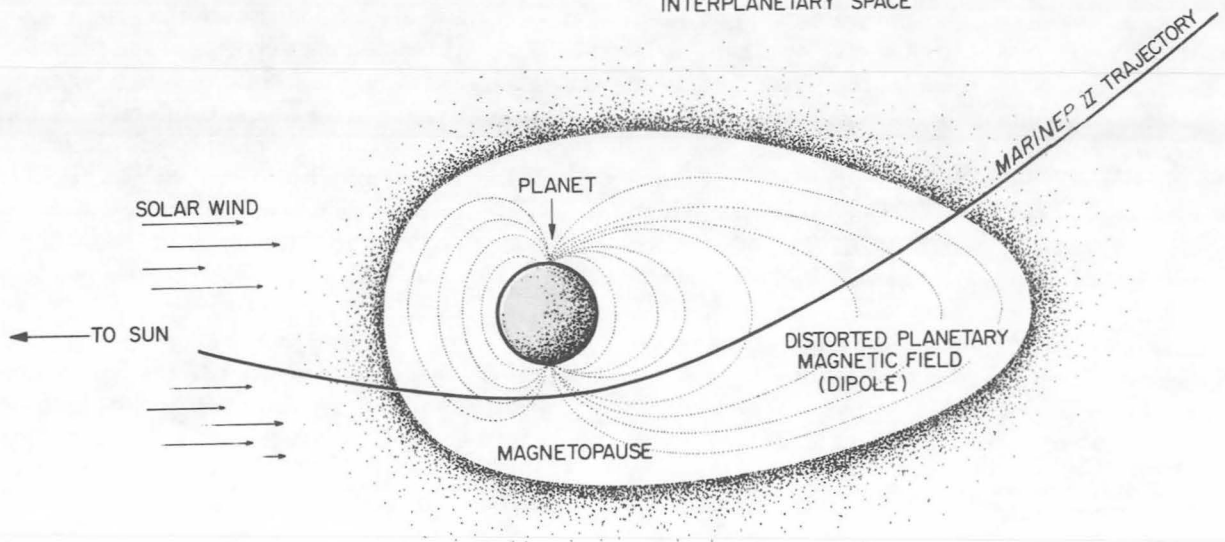
FIGURE 16-8.—Representation of possible shape of field lines of geomagnetic dipole as distorted by solar wind. (Shape of magnetosphere is highly conjectural, particularly in antisolar direction, and actual situation is considerably more complex than indicated.)
