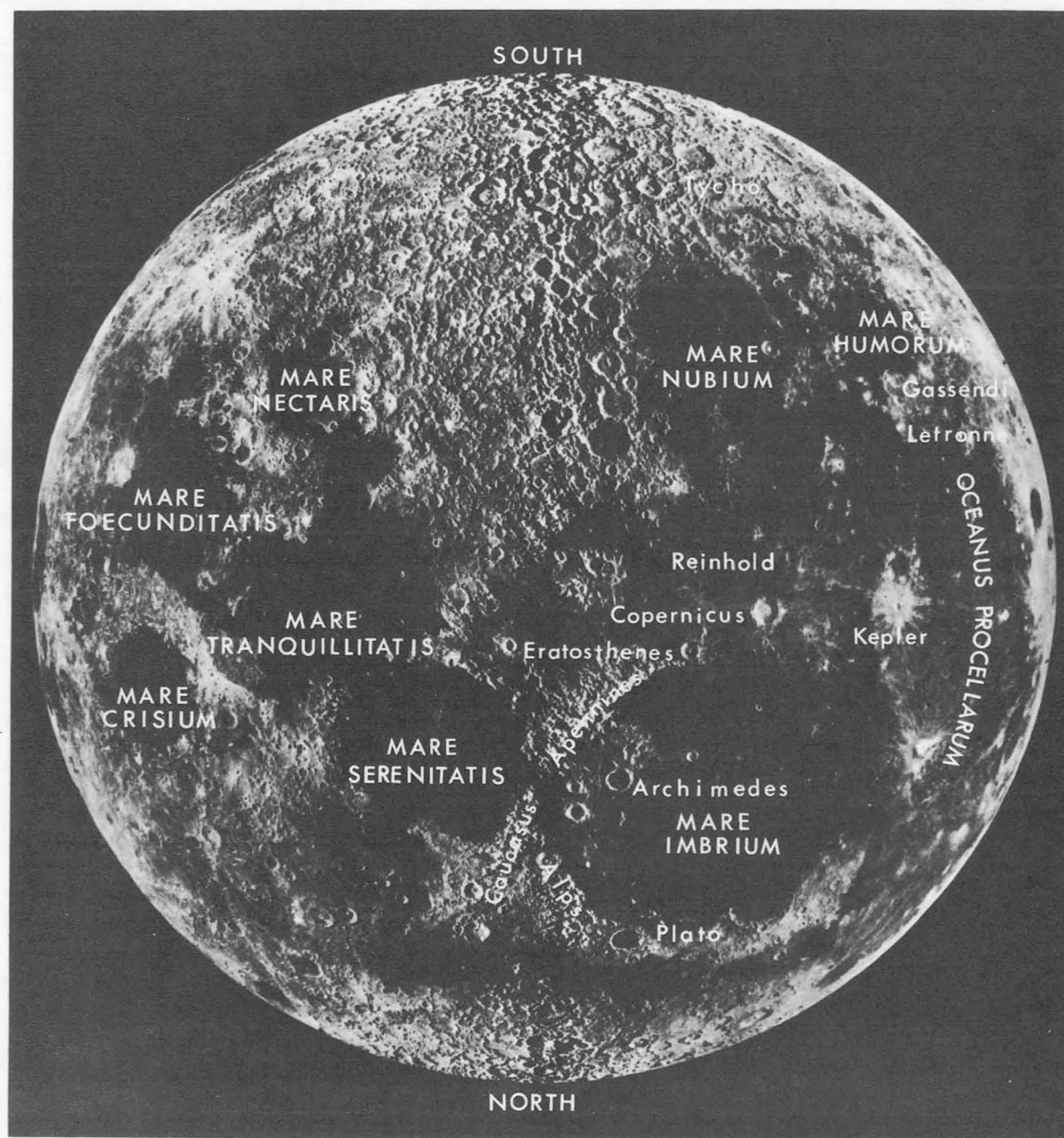
FIGURE 18-1.—Composite photograph of the full Moon. (North is down. Photograph courtesy Mt. Wilson and Palomar Observatories.)
