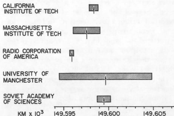
FIGURE 9-7.—Radar measurement of astronomical unit in April 1961.
