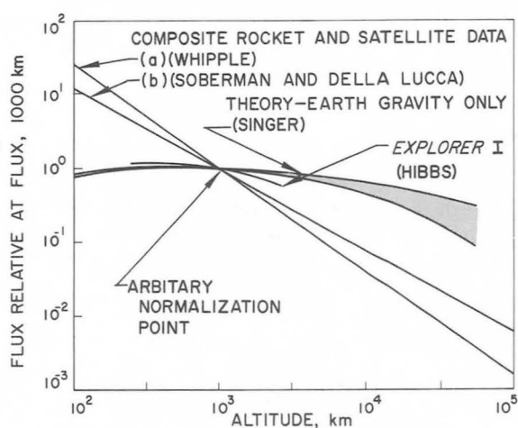
FIGURE 16-4.—Relative integral flux of dust particles as a function of altitude. (Compiled from Refs. 11, 12, 13, and 14.)
