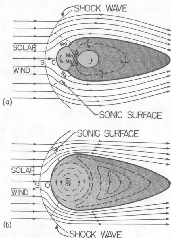
FIGURE 16-10.—Magnetosphere in a "supersonic" solar wind. (Diagrammatic sections (a) in plane of geomagnetic axis and solar-wind direction, and (b) in geomagnetic equatorial plane looking from above North pole. Geomagnetic tail is indicated by shading and sense of rotation of magnetosphere by short arrows. Lines outside magnetosphere represent streamlines of solar wind, and bow shock wave is shown on upstream side of magnetosphere. Flow behind shock wave becomes supersonic as it passes through sonic surface, roughly in position indicated by lightly dotted lines. From Ref. 21.)
