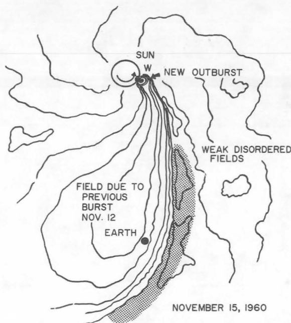
FIGURE 16-27.—Proposed solar magnetic field configuration to explain phenomena observed in connection with the solar flare event of November 15, 1960. (From Ref. 44.)
