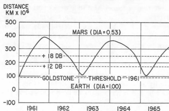
FIGURE 9-13.—Radar detectability of Mars with Goldstone-type radar.
