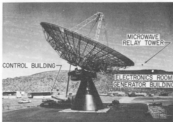
FIGURE 9-4.—85-ft.-diameter Goldstone azimuth-elevation (Az-El) antenna.
