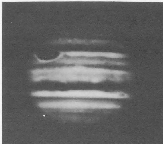
FIGURE 17-3.—Jupiter in blue light. 200-in. photograph, courtesy of Mt. Wilson and Palomar Observatories.
