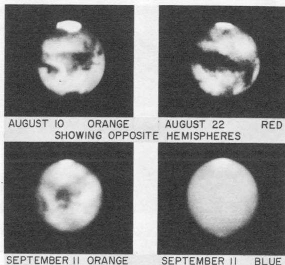
FIGURE 18-14.—Photographs of Mars in different colored light, in different months, during the opposition of 1956. (Wilson and Palomar Observatories photographs.)
