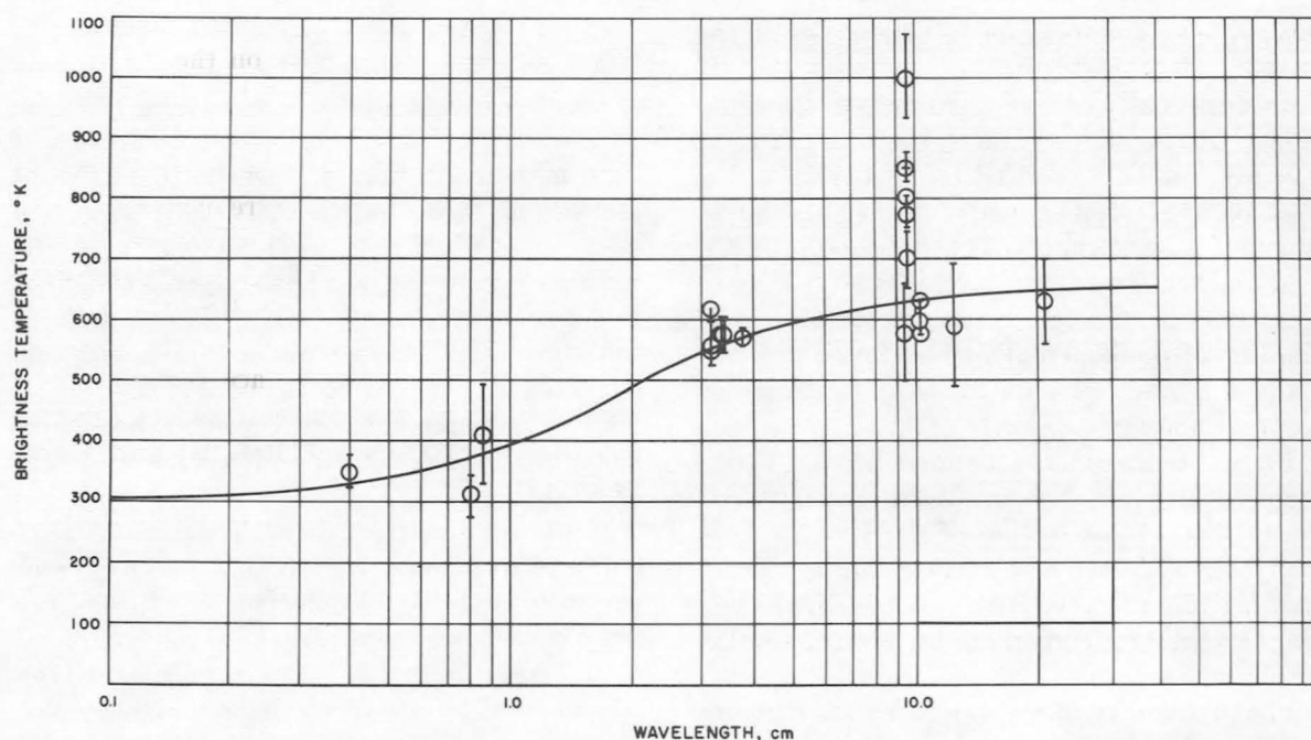
FIGURE 18-11.—Microwave temperatures of Venus obtained near inferior conjunction. (Length of vertical bars indicates uncertainty. From Victor, et al.)
