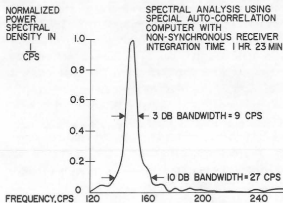
FIGURE 9-8.—Venus-reflected signal, April 21, 1961.
