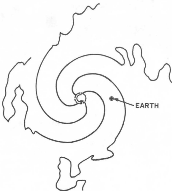
FIGURE 16-9.—Hypothetical shape of solar equatorial magnetic field resulting from radial solar wind, showing "garden-hose effect" and onset of turbulence at large radii.
