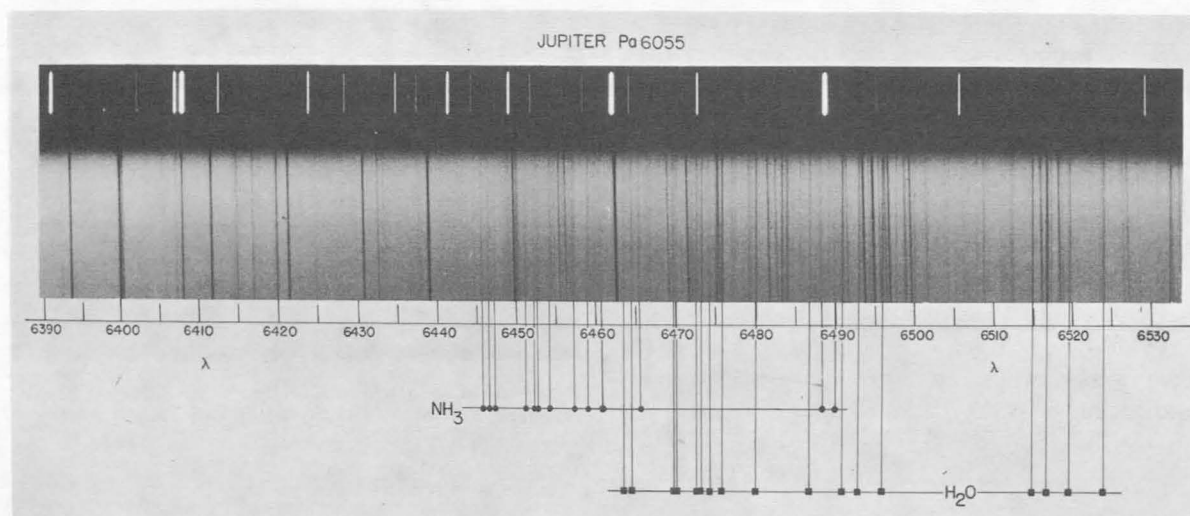
FIGURE 17-2.—A Palomar 200-in. reflector coude spectrogram of Jupiter taken by Münch with the slit parallel to the equator. Original dispersion 3.3 \text{ \AA/mm} . Most of the unmarked lines are reflected Fraunhofer lines.
