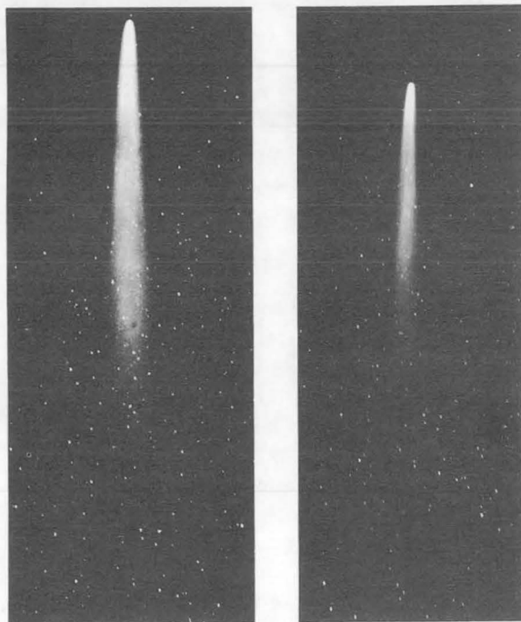
FIGURE 16-5.—Halley's Comet, May 12 and 15, 1910. (Tails 30 and 40 deg long. Photographed from Honolulu with 10-in. focal-length Tessar lens.)
