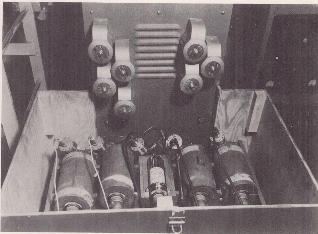
Figure 7.- Alphatron and diaphragm sensing heads. L-62-4750
