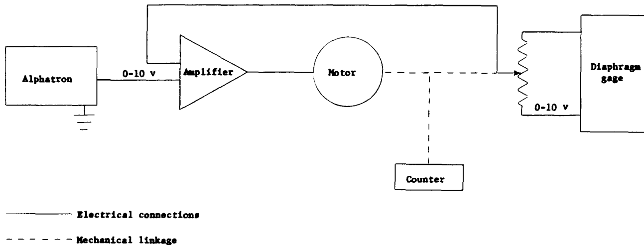
Figure 1.- Ratio meter.
