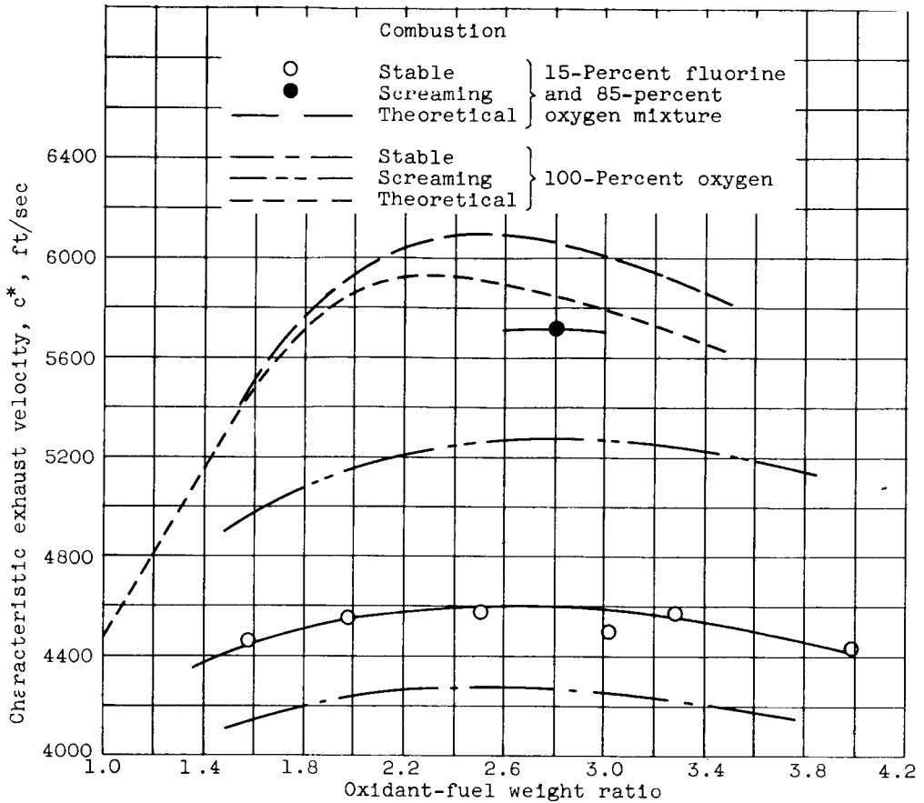
(a) Characteristic velocity.
