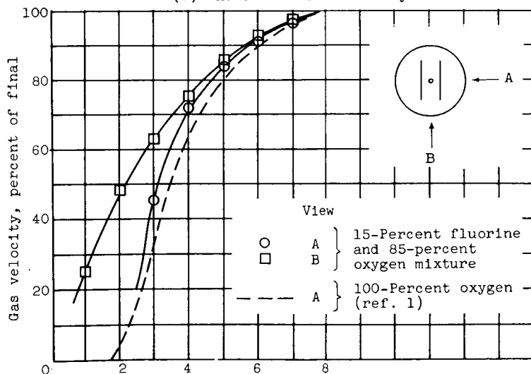
(b) Chamber gas velocity.
