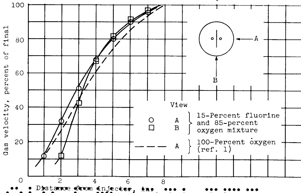
(b) Chamber gas velocity.
