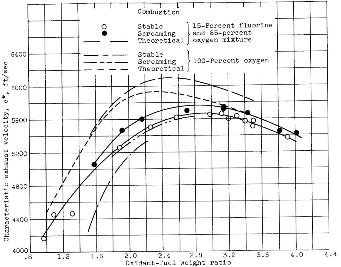
(a) Characteristic velocity.
