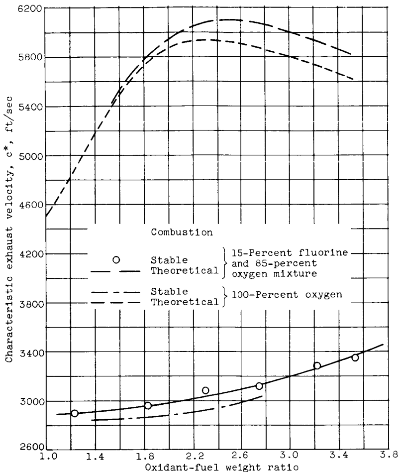
(a) Characteristic velocity.
