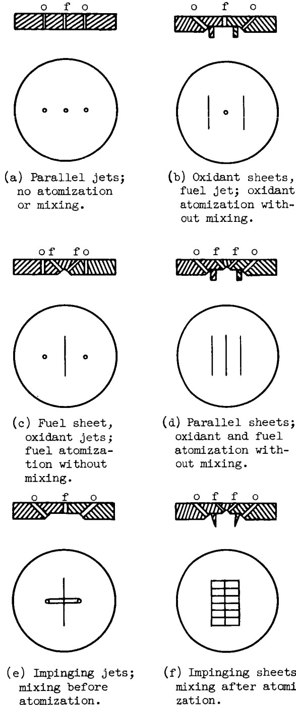
Figure 1. - Injector designs and spray patterns. Fuel injection equally spaced between two positions of oxidant injection. Centerline spacing between fuel and oxidant injection, 0.25 inch. Oxidant orifice diameter, 0.111 inch; single fuel orifice diameter, 0.116 inch; double fuel orifice diameter, 0.082 inch.
