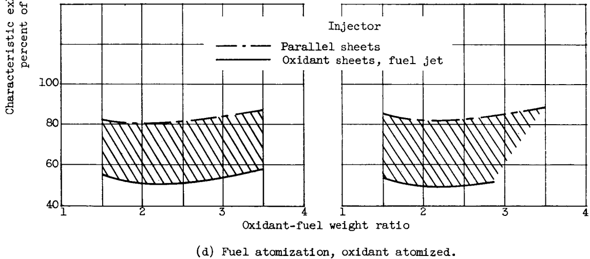
Figure 8. - Continued. Performance gain for various injection processes from a comparison of injector performance for both 15-percent fluorine and 85-percent oxygen mixture and 100-percent oxygen with heptane.
