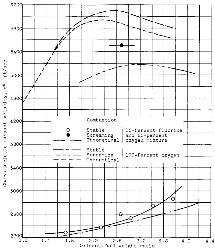
(a) Characteristic exhaust velocity.
