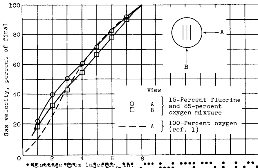
Figure 5. - Performance of parallel-sheets injector.
