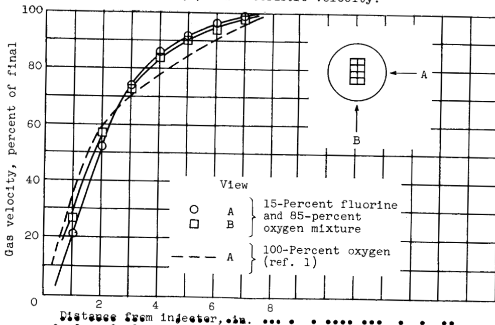
(b) Chamber gas velocity.
