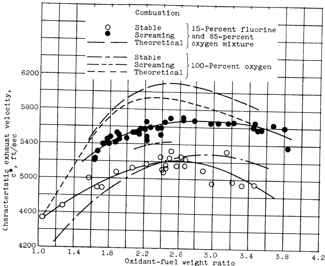
(a) Characteristic velocity.
