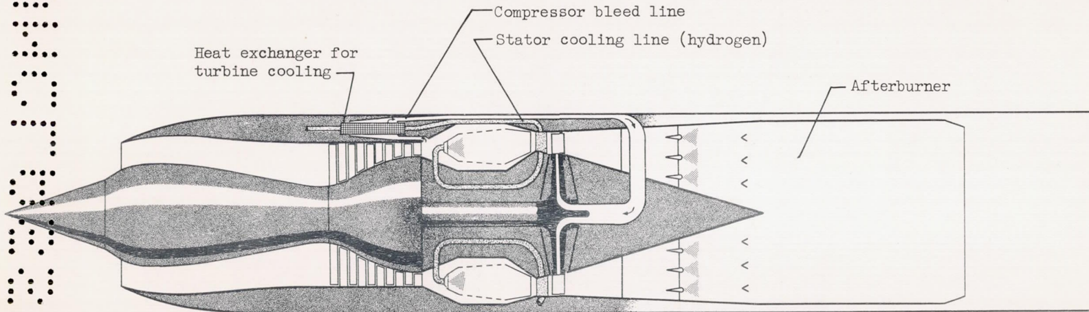
Figure 24. - Schematic diagram of turbojet engine C and turbine-cooling arrangement.
