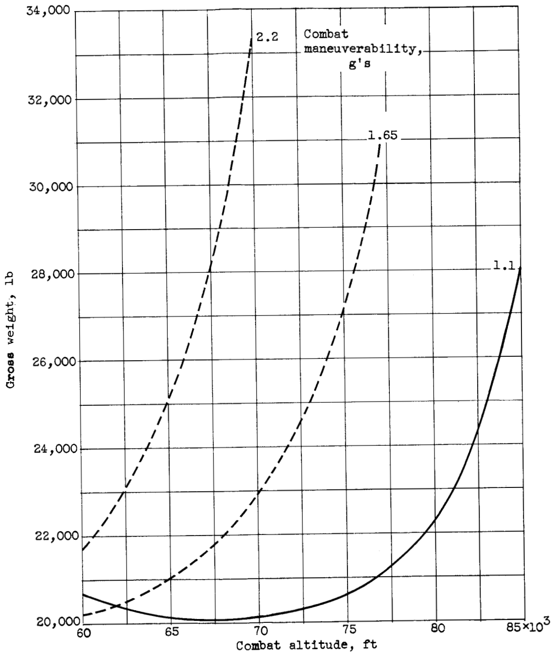
Figure 30. - Effect of combat altitude and maneuverability on gross weight of supersonic fighter. Flight Mach number, 2.5; engine C; combat radius, 500 nautical miles.
