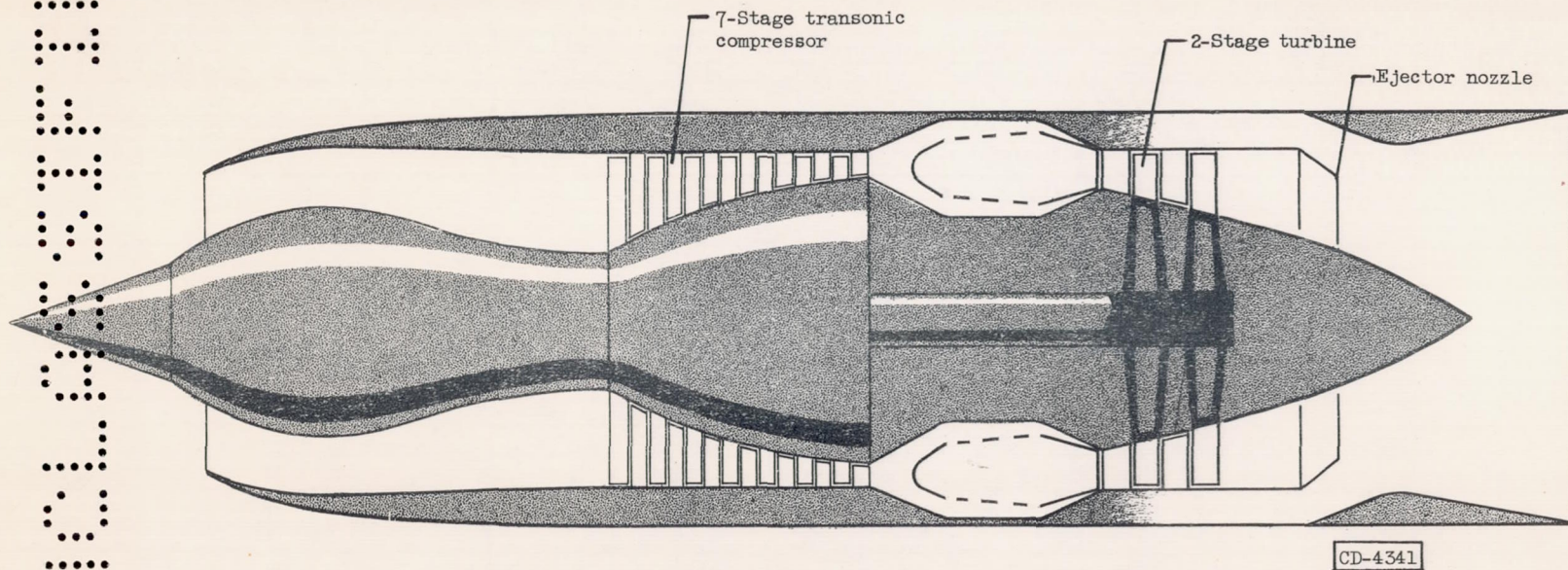
Figure 21. - Schematic diagram of turbojet engine B.
