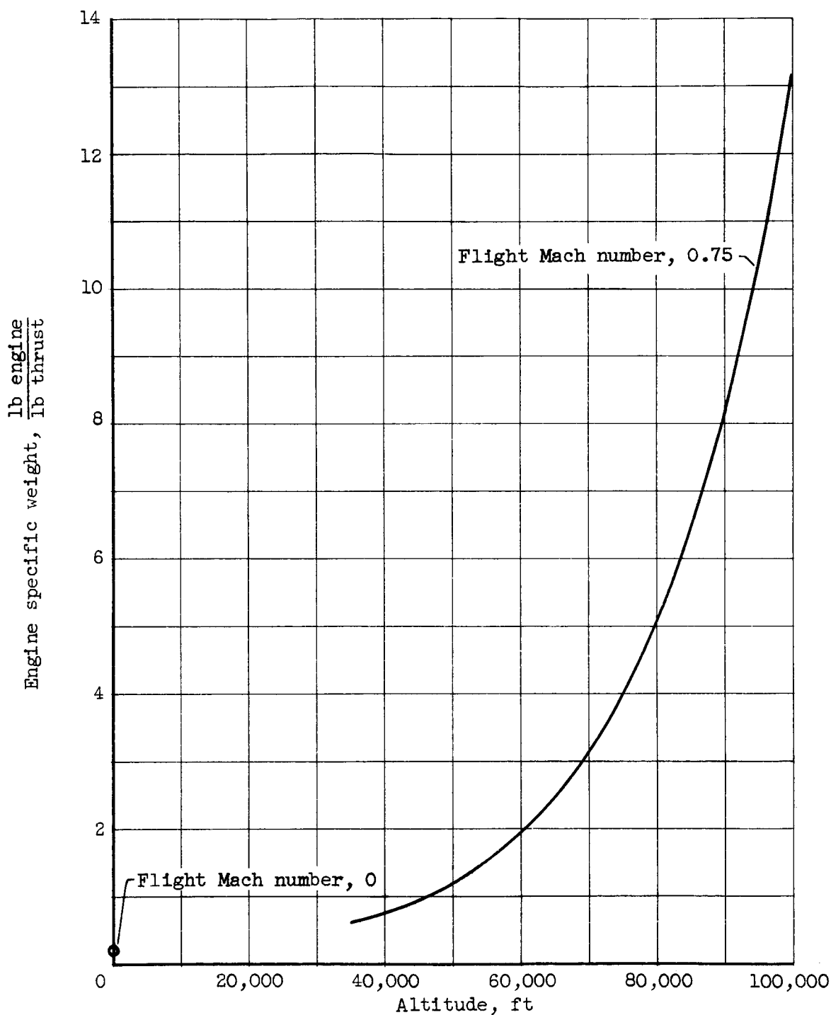
Figure 10. - Effect of altitude on engine specific weight.
