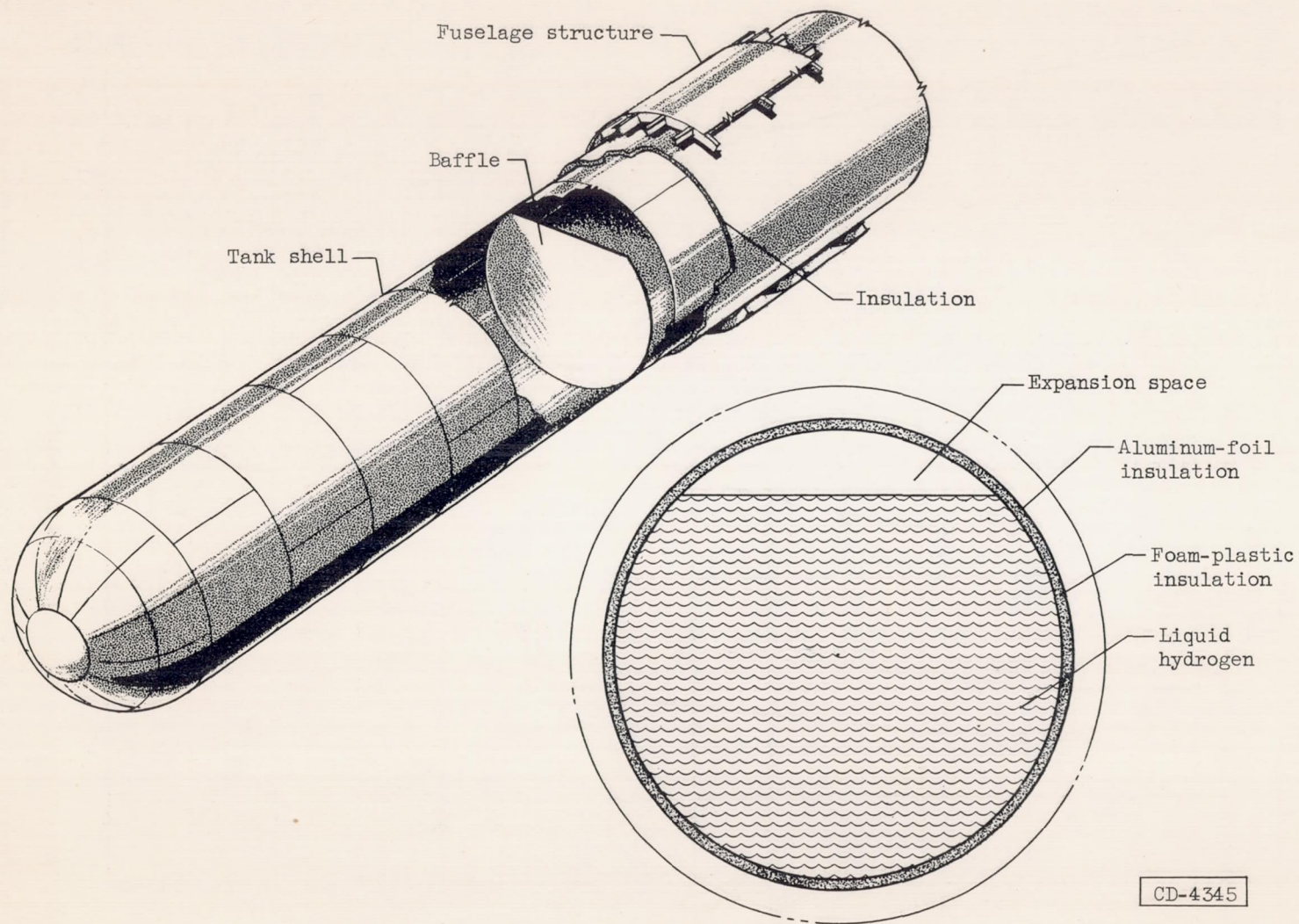
Figure 9. - Liquid hydrogen fuel tank.
