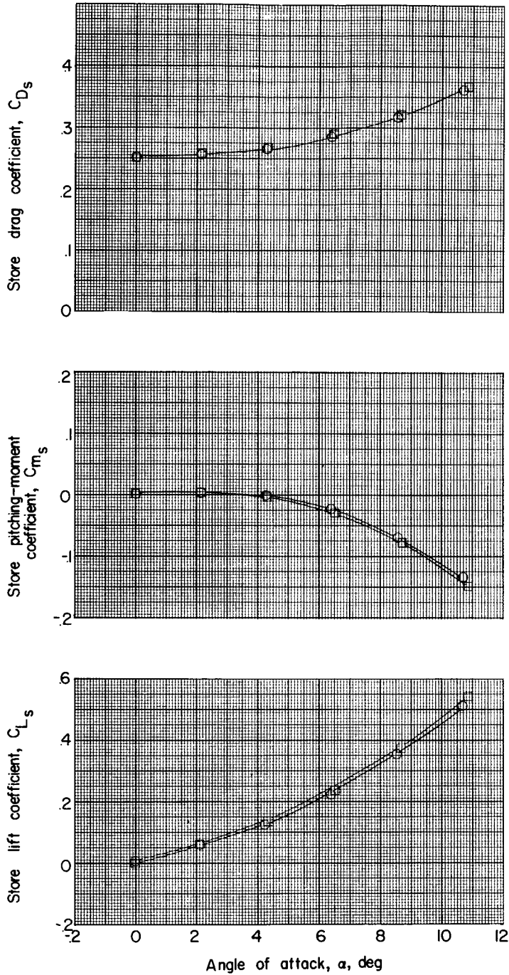
(a) Large and small ogive-cylinder stores.
