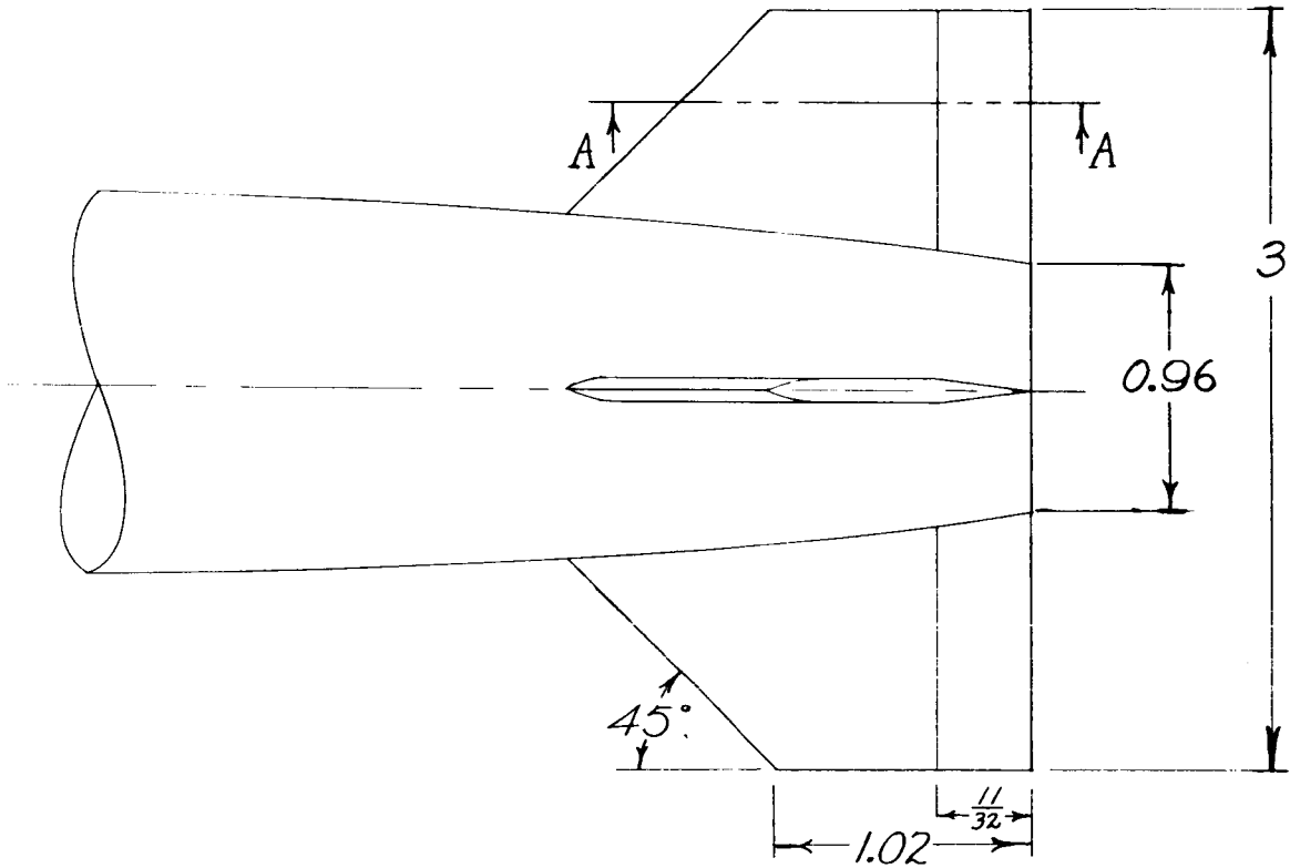
Figure 4.- Details of fins for large ogive-cylinder store. All dimensions are in inches. Fins were oriented at 45° for all tests.
