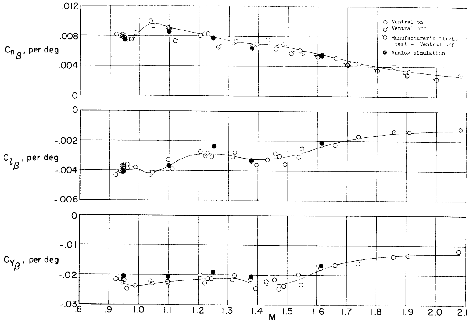
Figure 13.- Flight-determined static lateral-directional stability derivatives.
