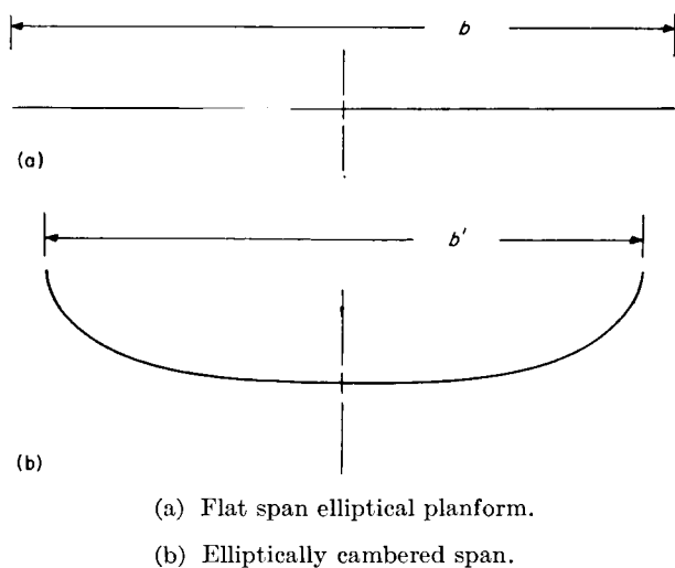
FIGURE 38.—Comparison of a flat elliptical-planform span with an elliptically cambered span.
