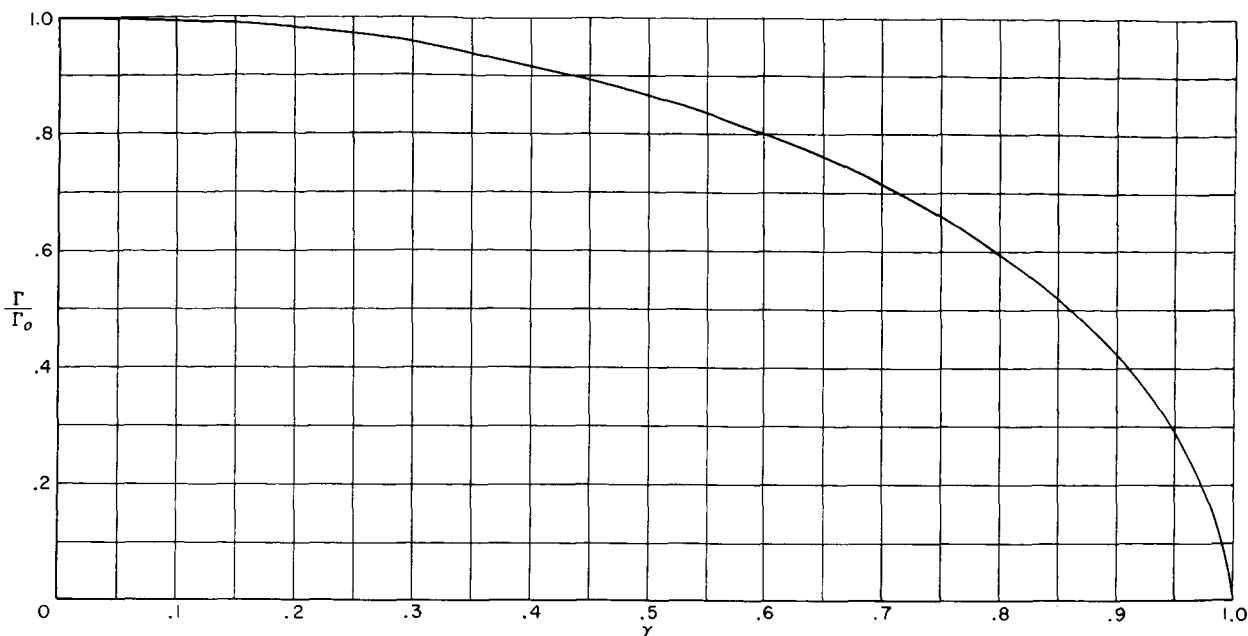
FIGURE 21.—The optimum nondimensional circulation loading for closed ellipses. 0 \leq \beta \leq 1.0 .
